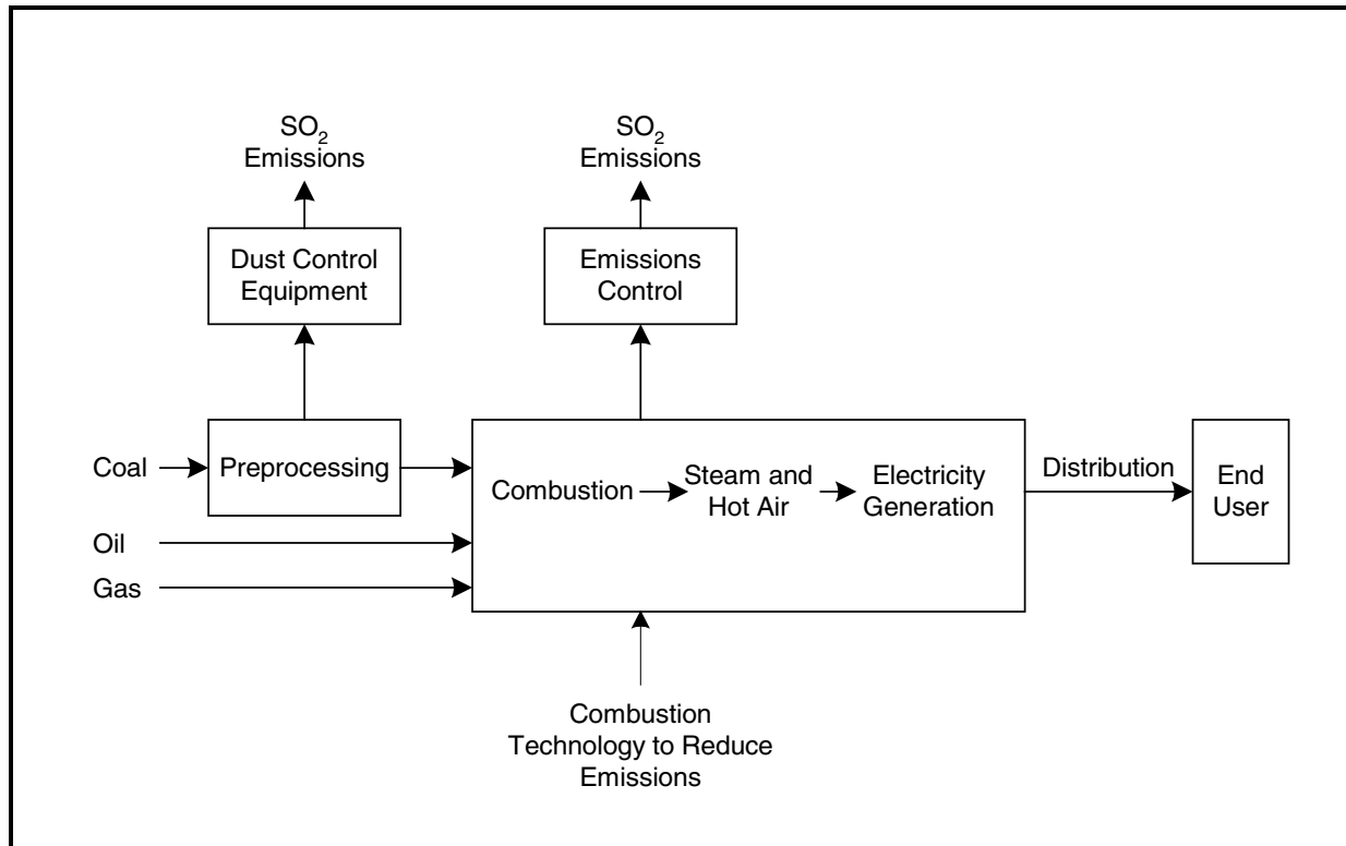
Figure C-6. Electricity Generation Process
