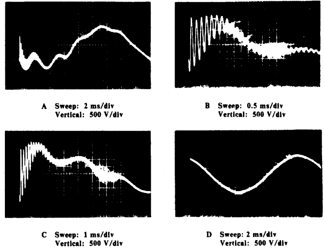
Figure 4. Capacitor switching transients and steady-state voltage
