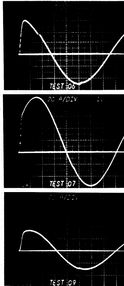
Fig. 5 Output of the second circuit.
