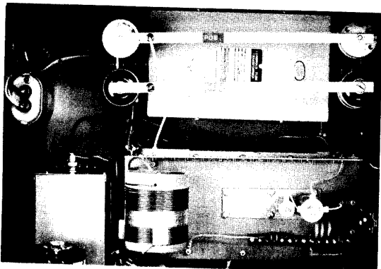
Fig. 9(a) Interior, top view.
