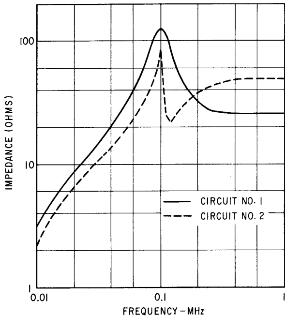
Fig. 6 Impedance of the two TCL circuits.
