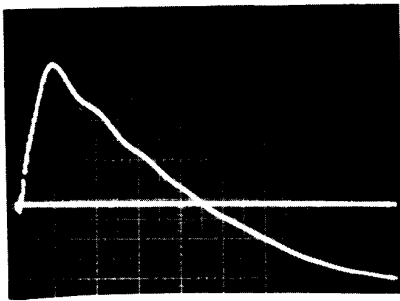
Fig. 14 Open-circuit voltage at maximum setting: 2 kV/div, 0.5 \mu s/div.
