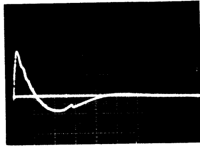
Fig. 16 Output voltage with 50-ohm load at maximum setting: 2 kV/div, 2 \mu s/div.
