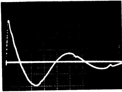
Fig. 13 Open-circuit voltage at maximum setting: 2 kV/div, 2 \mu s/div.
