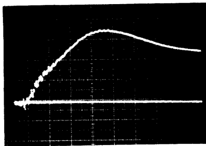
Fig. 15 Open-circuit voltage at maximum setting: 2 kV/div, 0.1 \mu s/div.
