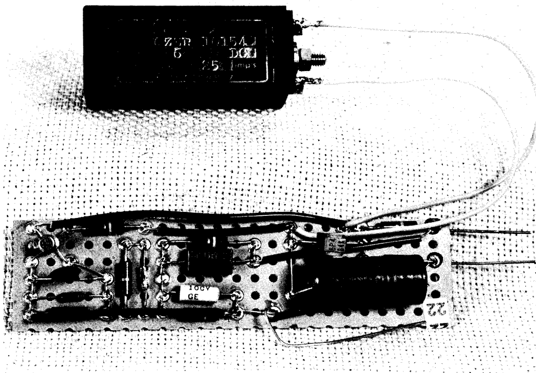
Surge counter - Active circuit and counter . The left side of the circuit, shielded by tubing shown in preceding photograph, is visible here. (ATL Photo No. 833103)
