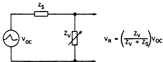
Figure 3. Voltage-clamping action
