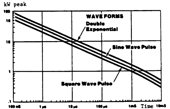
Figure 5. Peak pulse power vs. pulse time
