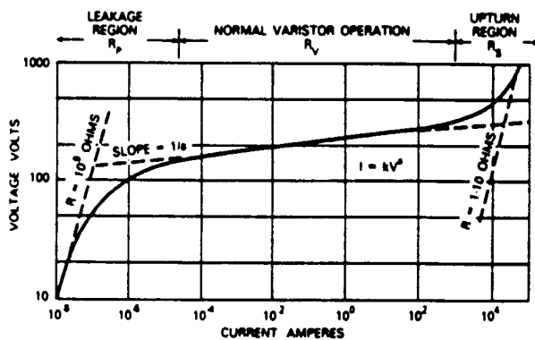
Figure 7. Theoretical V-I characteristic
