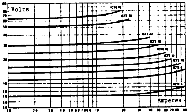
Figure 4. Typical V-I characteristic
