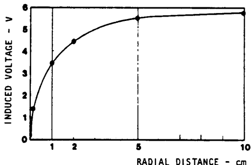
Figure 9. Voltage observed by probes versus radial distance from conductor to opposite side of rectangular loop
