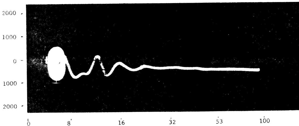
Internal switching transient (15 such transients in 1500 hours)
