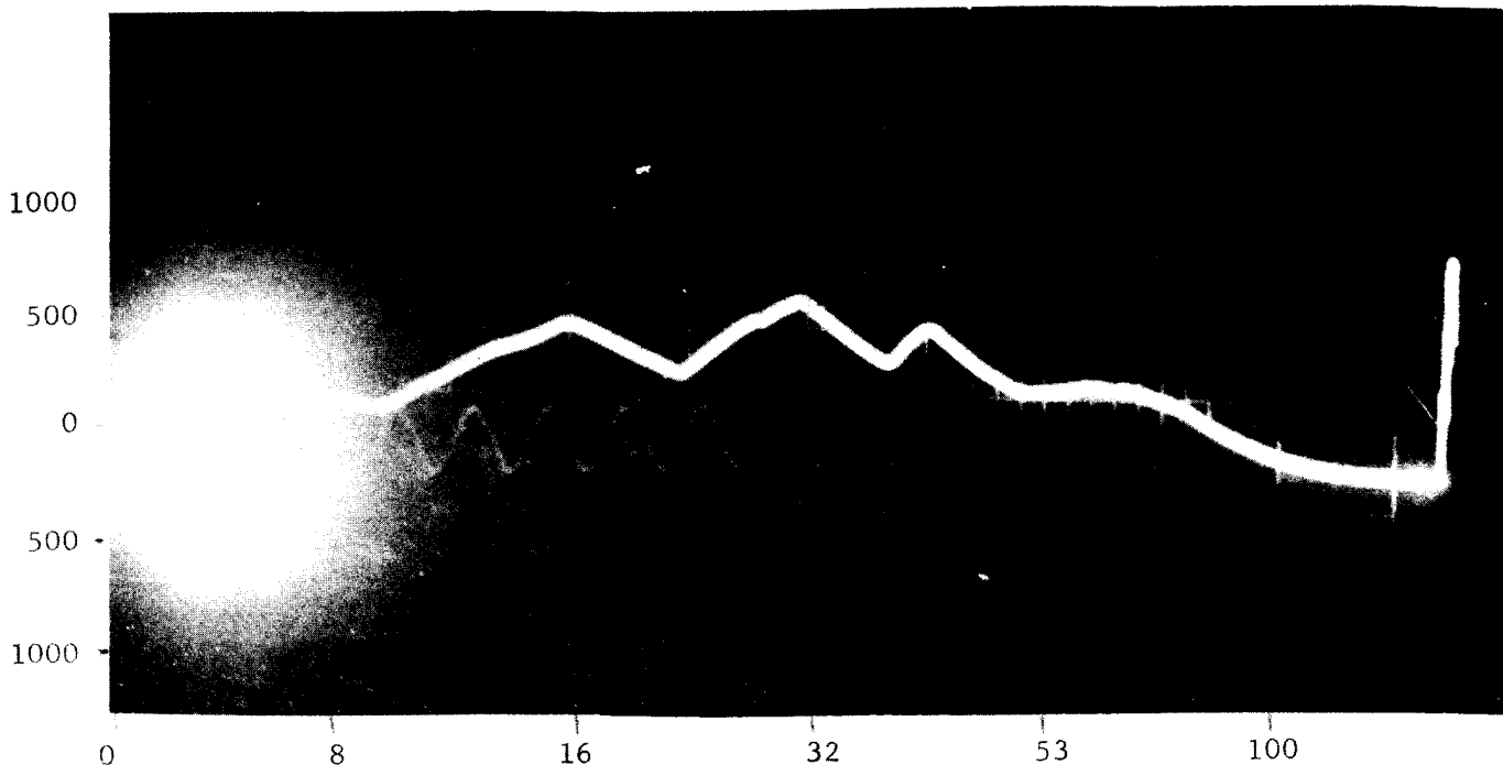
Switching transient with restrikes--probably external to the house. (The faint sine wave corresponds to the return of the electron beam which was not completely blanked out. It illustrates the peak-to-peak value of the steady state 117 voltage, but not at the same rate as the forward sweep.)
