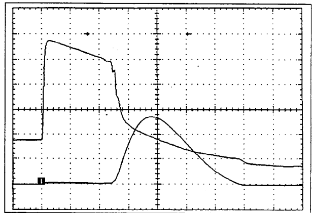
Top trace: Voltage across bulb terminals, 200 V/div Bottom trace: Current in bulb, 100 A/div Sweep: 10 \mu s/div
