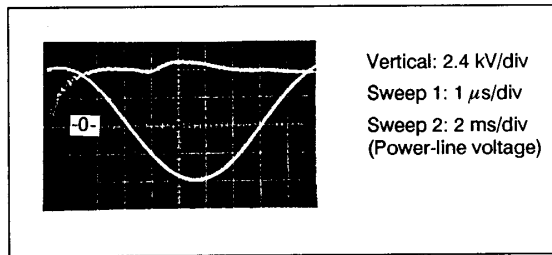
Figure 8. Surge Occurring on 6 kV Cable, between Conductor and Shield
