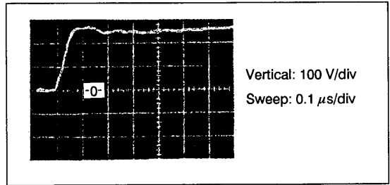
Figure 10. Surge Occurring on 380 V Cable
