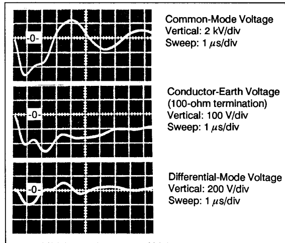
Figure 4. Transients Induced in Unshielded Control Cable
