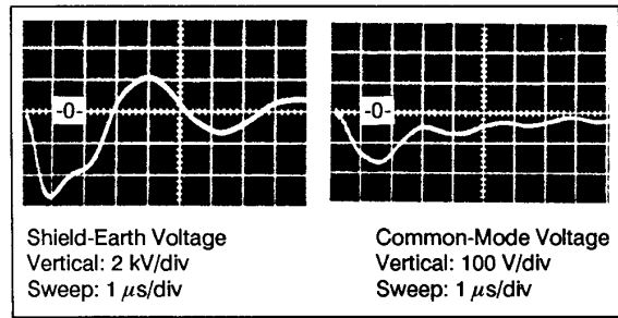
Figure 5. Transients Induced in Shielded Telephone Pair
