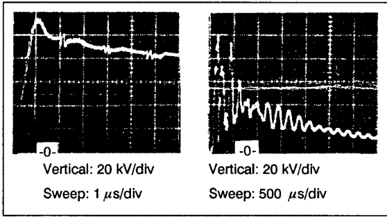
Figure 2. Surge Voltage Applied to the High-Voltage Line
