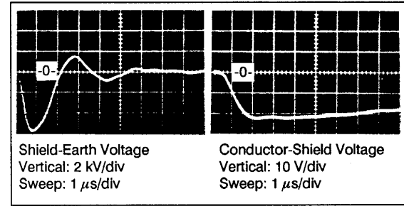
Figure 6. Transients Induced in Coaxial Cable
