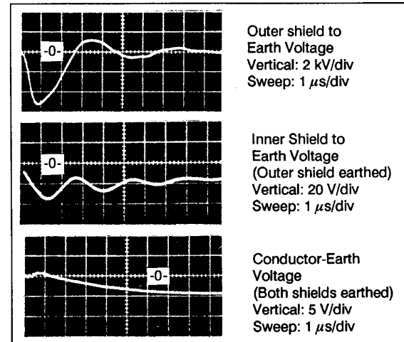
Figure 7. Transients Induced in Triaxial Cable
