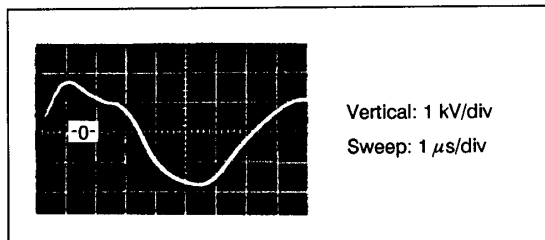
Figure 9. Surge Occurring on 6 kV Cable, between Shield and Earth, at Floating End of Shield
