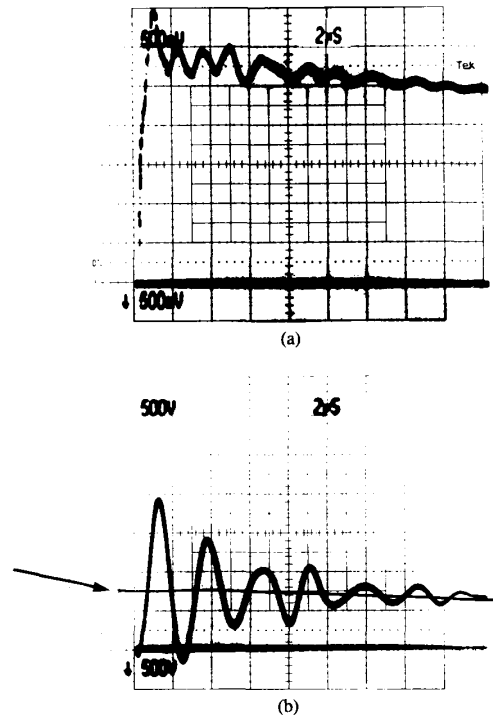
Fig. 5. Recordings at sending end (1) and receiving end (2), for 3-kV unidirectional surge. Minimum wiring connected 480-V bus (all breakers to 277 V branch circuits and 120 V branch circuits open). Voltage: 500 V/div; sweep: 2 \mu s/div. (a) Voltage at sending end. (b) Voltage at receiving end. Note line showing unidirectional component.
