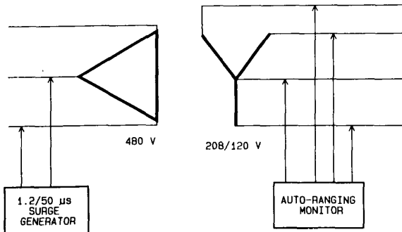
Fig. 2. Coupling of surge through delta-wye step-down transformer.
