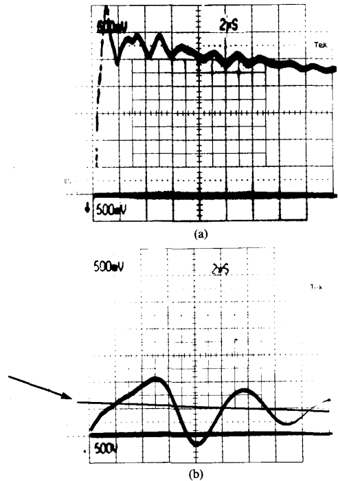
Fig. 6. Recordings at sending end (1) and receiving end (2), for 3-kV unidirectional surge. All 277-V lighting branch circuits connected to 480-V bus. Voltage: 500 V/div; sweep 2 \mu s/div. (a) Voltage at sending end. (b) Voltage at receiving end. Note line showing unidirectional component.
