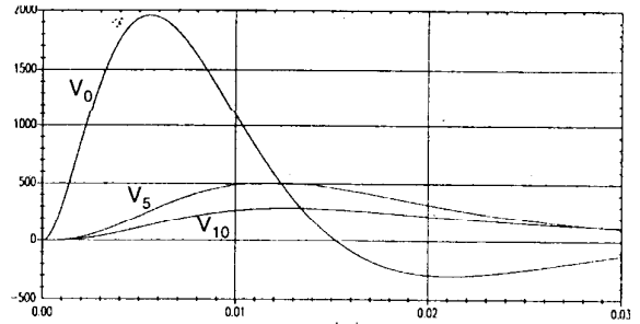
Voltages at nodes: Time in milliseconds, peaks in volts
