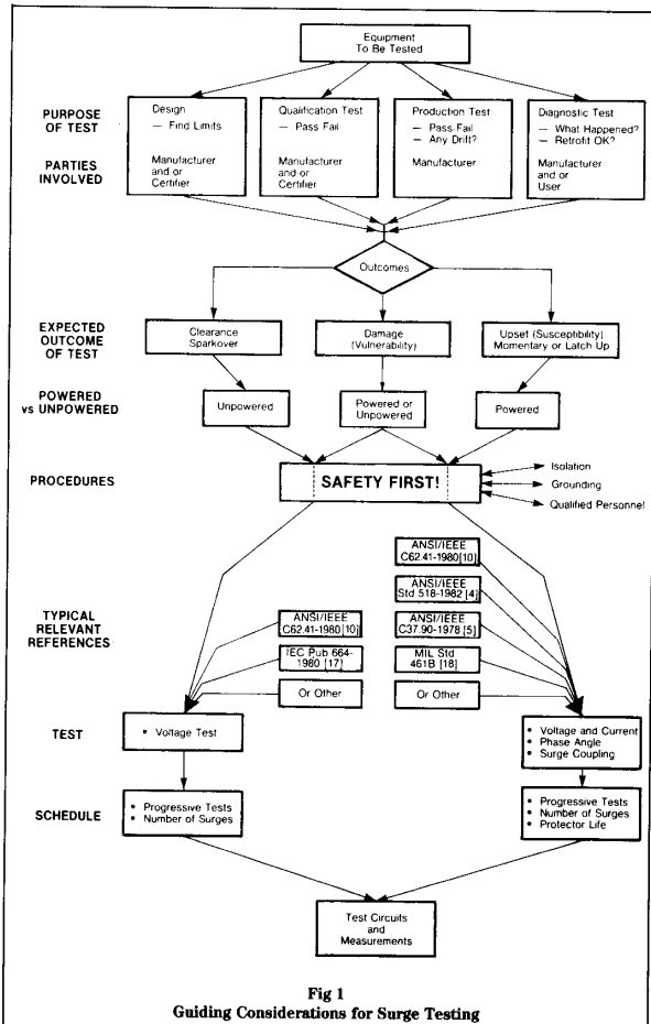
Figure 1—Considerations Involved in Planning a Surge Test
