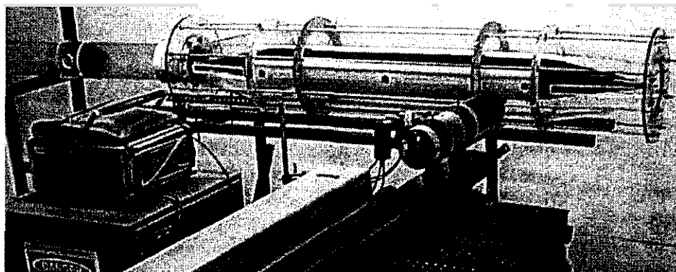
Figure 3. Quarter-Scale Simulator with LDA test setup.
