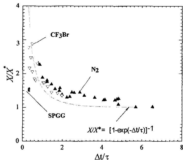
Figure 1. Comparison of N_2 , CF_3Br , and SPGG effectiveness in the TARPF.
