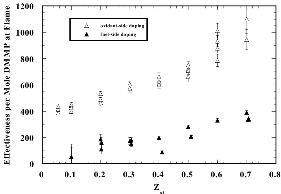
Figure 13. Normalized flame suppression effectiveness for DMMP in methane/nitrogen vs. oxygen/nitrogen flames with fixed a_{q_0} . Effectiveness is normalized by the quantity of DMMP at the maximum temperature location in the flame, as predicted by a numerical simulation treating DMMP as inert. Error bars represent standard deviation of data and uncertainty in calculated loading.
