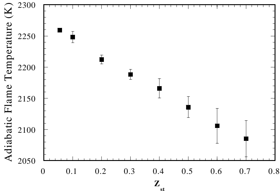
Figure 6. Adiabatic flame temperature as a function of stoichiometric mixture fraction for methane/nitrogen vs. oxygen/nitrogen flames with a_{q_0} held constant at 350 \pm 10 \text{ s}^{-1} . Error bars represent standard deviation of data.
