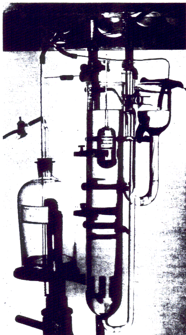
FIGURE 1. Hydrometer comparator.
