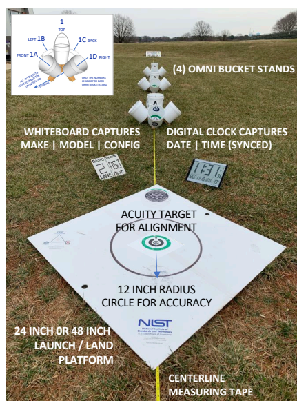
FIGURE 1) This Open Area Lane supports both Maneuvering (MAN) and Payload Functionality (PAY) test methods along with several other tests at various altitudes.
