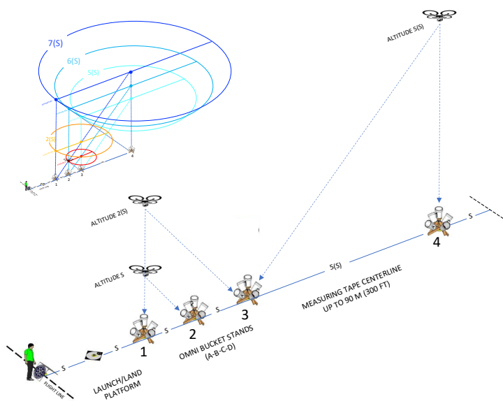
FIGURE 1) This Open Area Lane supports both Maneuvering (MAN) and Payload Functionality (PAY) test methods along with several other tests at various altitudes.
