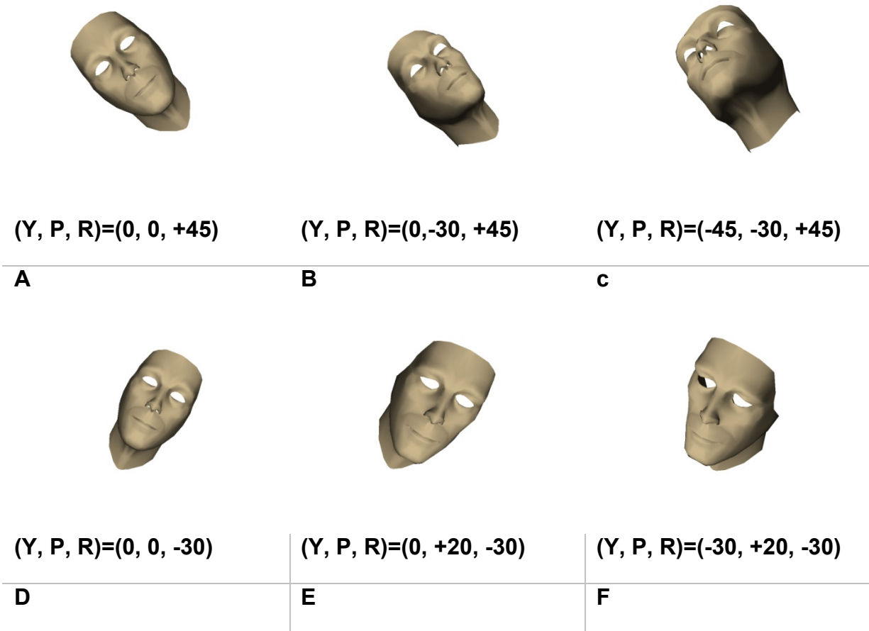
Figure 5 – Examples of the order of rotation through pose angles with an origin of coordinate system at the nose tip. Figures (a)-(c) show three successive rotation steps to achieve the pose angles (Y, P, R) of (-45, -30, +45). Figures (d)-(f) show three successive rotation steps to achieve the pose angles (Y, P, R) of (-30, +20, -30).
