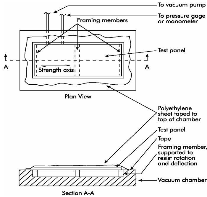
Figure 2. Vacuum Test Chamber Equipment
