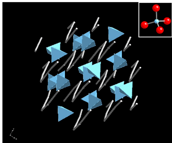
Fig. 14. Rendering of the structure of \text{Ba}_2\text{TiO}_4 . The structure is a repetition of nearly perfect Ti-O tetrahedra that are rotated with respect to each other and are separated by zig-zag chains of Ba atoms. The lack of inversion symmetry in the Ti-O tetrahedra leads to a very large low-energy resonance in the XANES.
