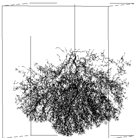
Fig. 15. Simulation of a dense streamer growth associated with a low cutoff-voltage parameter.
