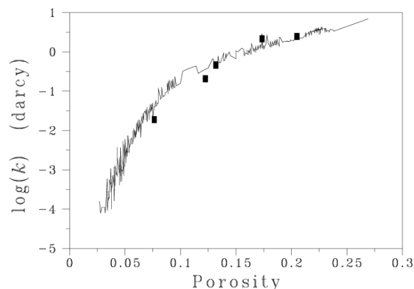
Fig. 6. Measured and modeled permeabilities ( k ) of Fontainebleau sandstone media as a function of porosity. The solid rectangles show the modeled results.
