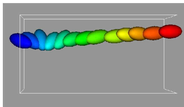
Fig. 7. Motion of a single ellipsoidal inclusion subject to shear. The single ellipsoid rotation is a well known phenomenon seen in experiments called Jefferies orbits.
