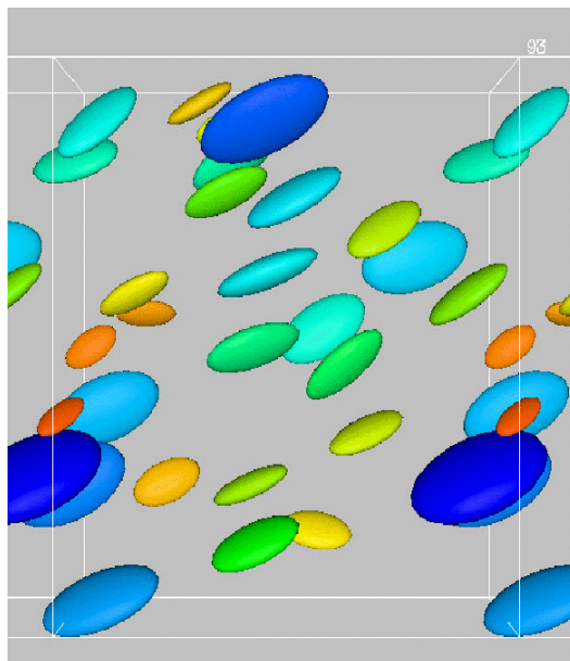
Fig. 8. Motion of twenty eight ellipsoidal inclusions, of size varying up to a factor of two, subject to shear. Note that the Jefferies orbits are suppressed due to hydrodynamic interactions between ellipsoids.
