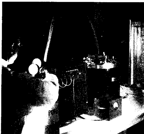
Figure 12.—Pure helium from a cylinder at high pressure is passed through a pressure-reduction gage into the humidifying unit, from which it is directed into the document enclosure. The gas is allowed to flow through the enclosure for several days to flush out the air and replace it with an inert atmosphere. Mr. E. C. Creitz is adjusting the helium flow preparatory to flushing the test enclosure.
