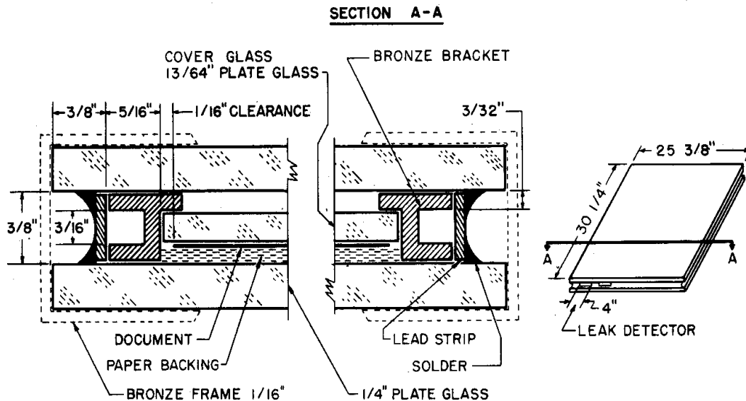
Figure 1. —Section sketch of the glass enclosure recommended for the preservation of the Declaration of Independence and the Constitution of the United States. The backing paper and cover glass position the document, the bronze bracket separates the glass plates from the assembly, and the lead strip soldered to the glass plate completely seals the document from the outside atmosphere. The size shown is for the Constitution.
