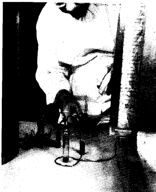
Figure 11.—The outlet tube of the enclosure is connected by copper tubing to a bubble counter and gas seal, consisting of a glass tube dipping just below the surface of a small quantity of oil. Humidified helium passes through the enclosure, over the document, and out through the liquid seal. The seal prevents air from backing up into the enclosure should the flow of helium be interrupted. Mr. E. C. Creitz is installing the liquid seal apparatus.
