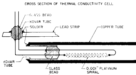
Figure 18.—The special thermal conductivity cell developed at the National Bureau of Standards for the preservation of the Declaration of Independence and the Constitution. The small filament (left in the photograph) consists of a fine platinum wire, wound into a helix, and supported on a pair of Kovar wires which, in turn, are sealed in the Kovar tube by a glass bead. The assembly is soldered in the copper tube (right) so that the position of the filament is fixed in relation to the tube. An electrical current passing through the platinum spiral causes it to increase in temperature, with a corresponding increase in electrical resistance; this increase is greater in air than in helium. The ammeter of the leak detector unit is set to read zero when the platinum spiral is in helium and 100 when it is in air.
