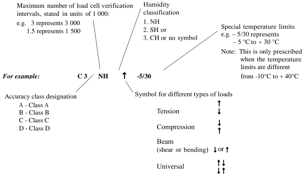
Figure 43. Complete load cell classification
