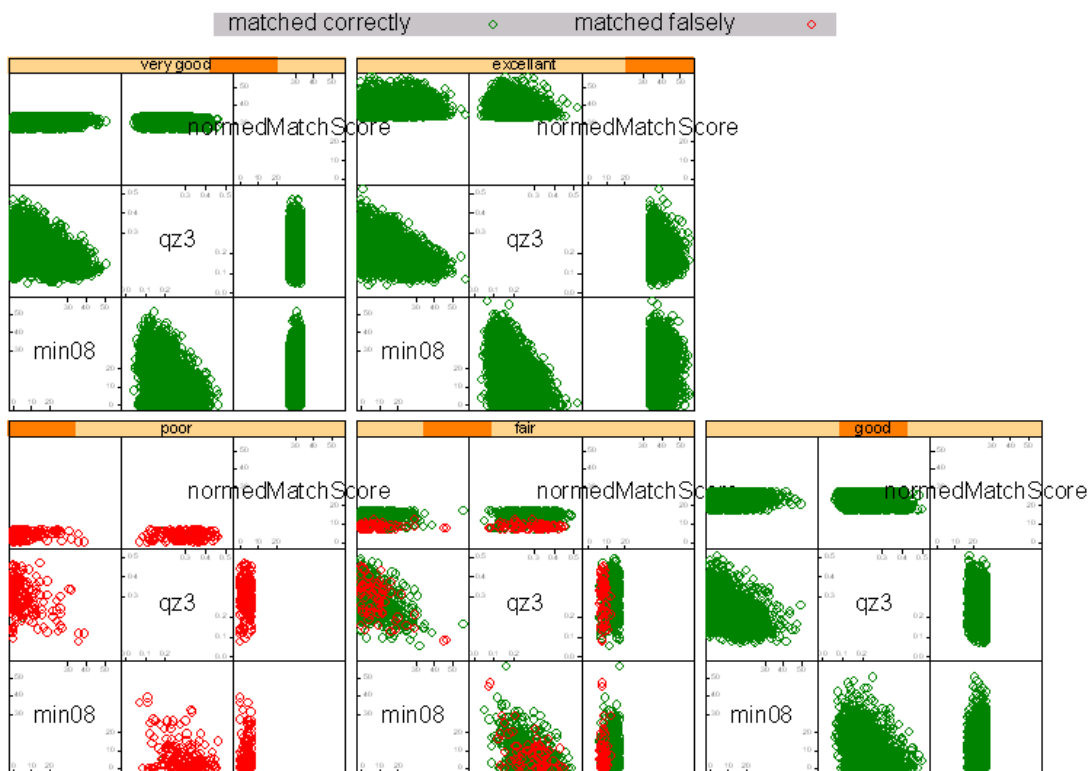
Figure 14. Trellis plot of min08 quality zone3 and normalized match scores of vendor F and right index fingerprints of dataset DOS-C
