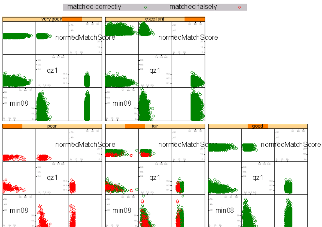
Figure 4. Trellis plot of min08 quality zone1 and normalized match scores of vendor F and right index fingerprints of dataset DOS-C
