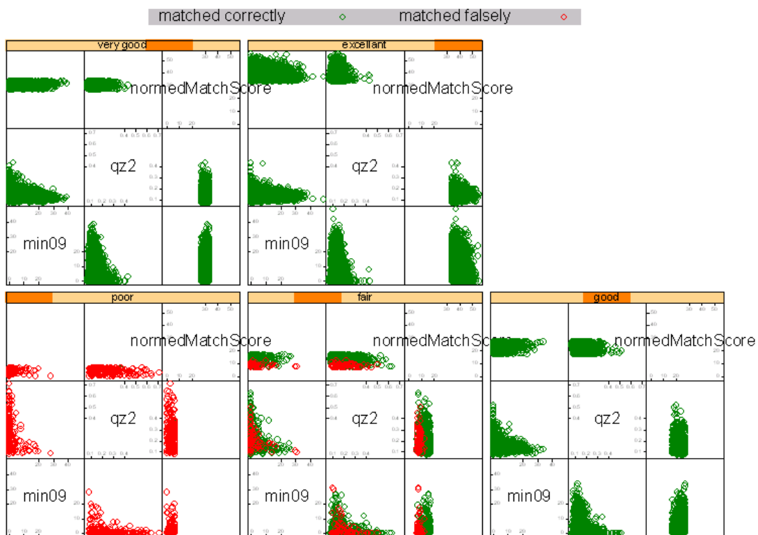
Figure 10. Trellis plot of min09 quality zone2 and normalized match scores of vendor F and right index fingerprints of dataset DOS-C
