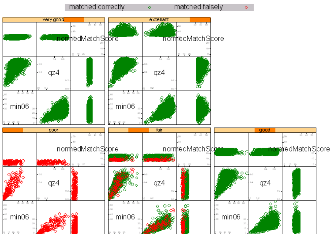
Figure 17. Trellis plot of min06 quality zone4 and normalized match scores of vendor F and right index fingerprints of dataset DOS-C
