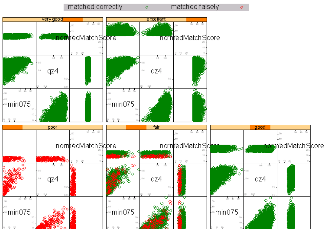
Figure 18. Trellis plot of min075 quality zone4 and normalized match scores of vendor F and right index fingerprints of dataset DOS-C
