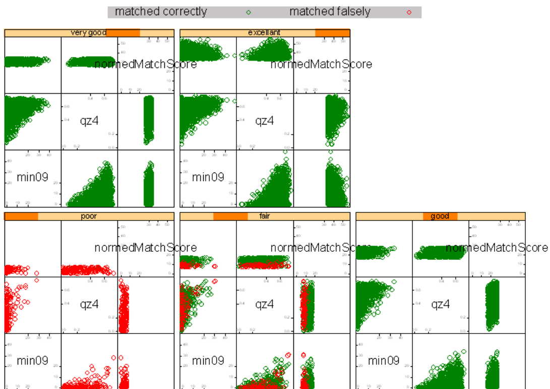
Figure 20. Trellis plot of min09 quality zone4 and normalized match scores of vendor F and right index fingerprints of dataset DOS-C
