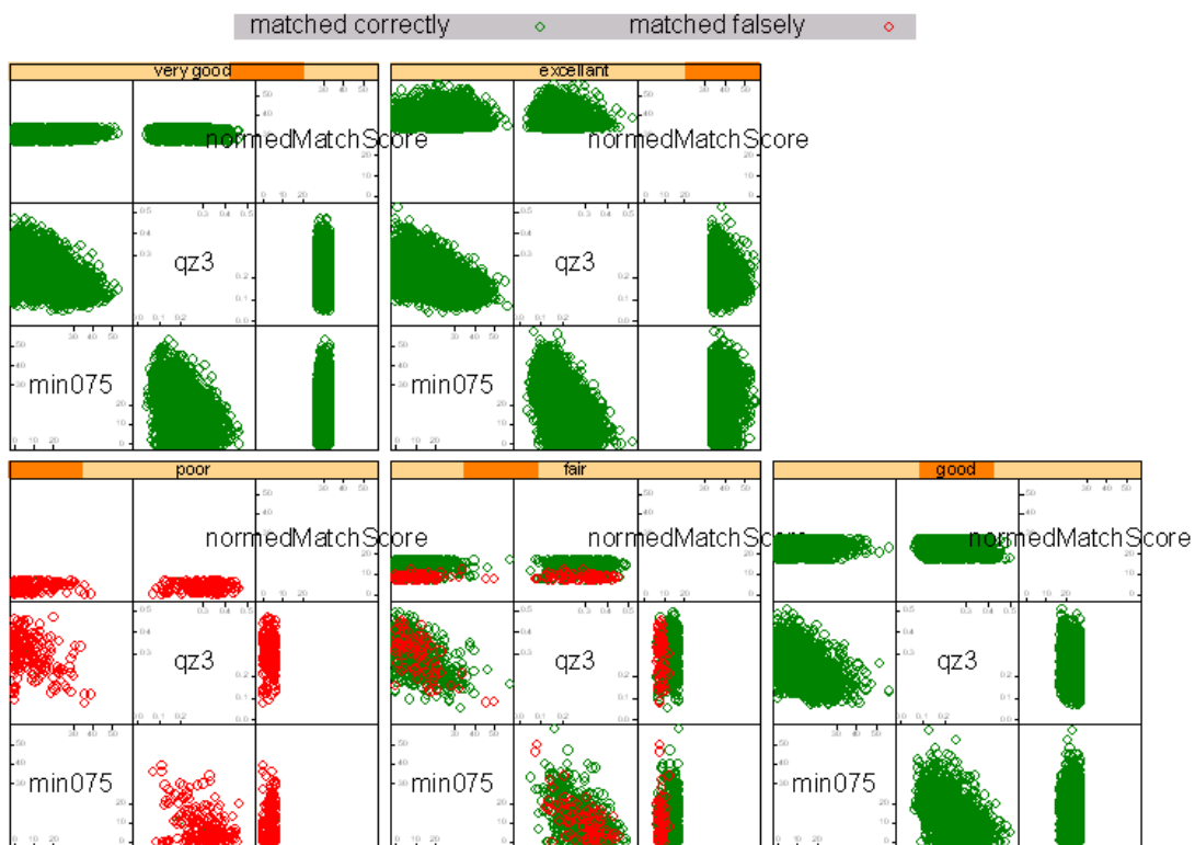
Figure 13. Trellis plot of min075 quality zone3 and normalized match scores of vendor F and right index fingerprints of dataset DOS-C
