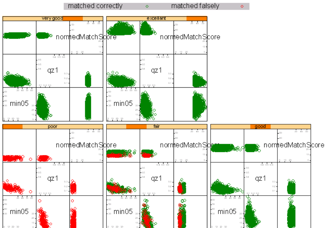
Figure 1. Trellis plot of min05 quality zone1 and normalized match scores of vendor F and right index fingerprints of dataset DOS-C
