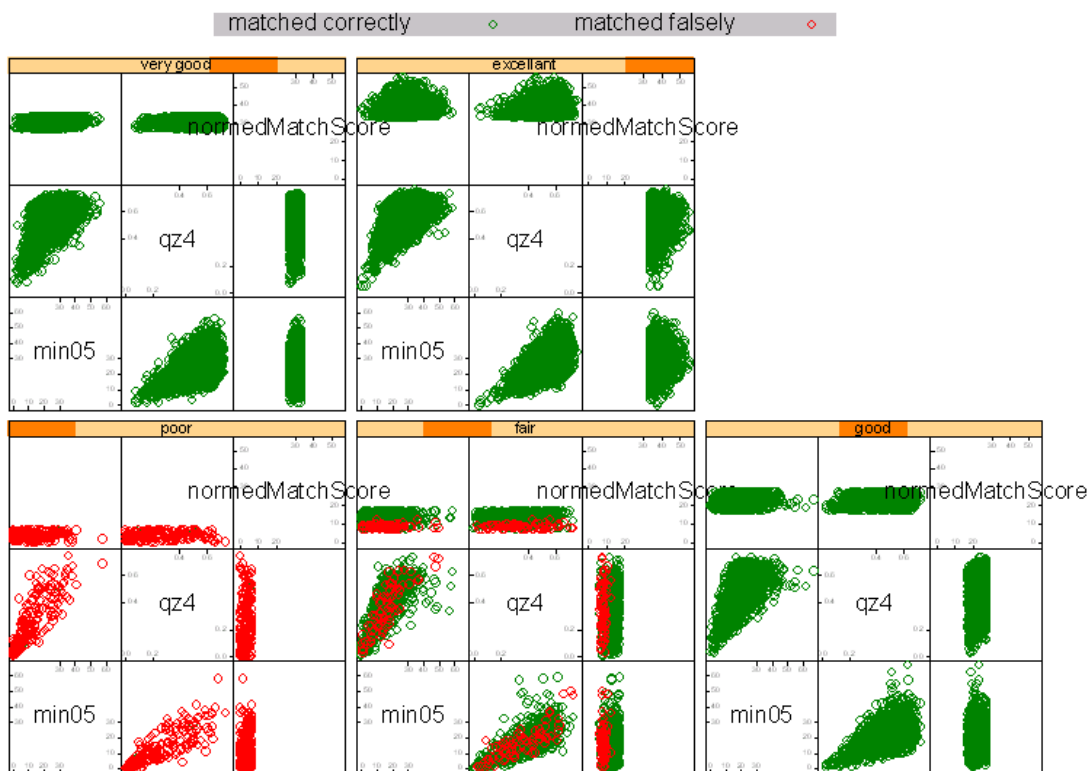
Figure 16. Trellis plot of min05 quality zone4 and normalized match scores of vendor F and right index fingerprints of dataset DOS-C
