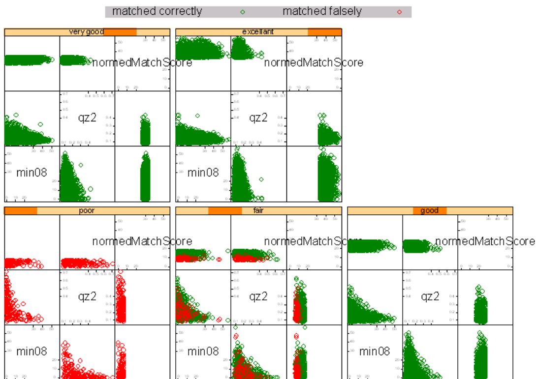
Figure 9. Trellis plot of min08 quality zone2 and normalized match scores of vendor F and right index fingerprints of dataset DOS-C
