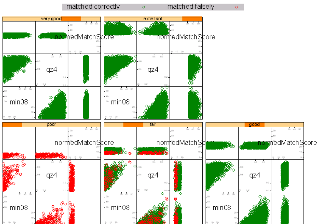
Figure 19. Trellis plot of min08 quality zone4 and normalized match scores of vendor F and right index fingerprints of dataset DOS-C
