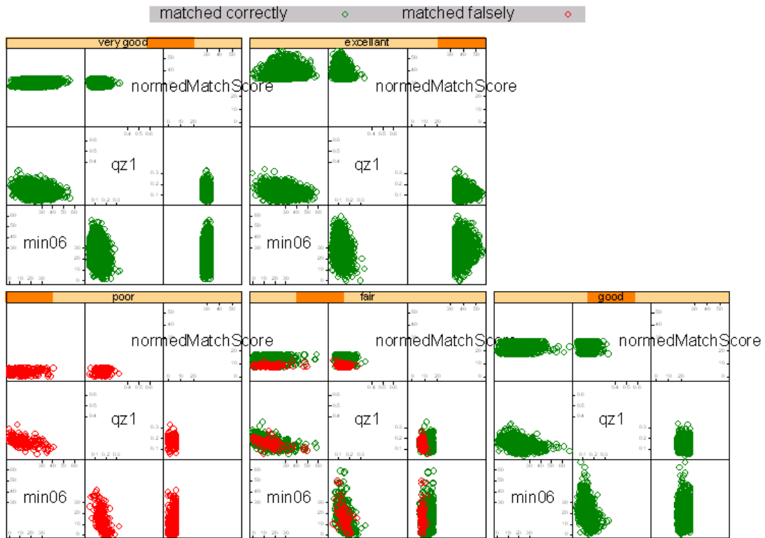
Figure 2. Trellis plot of min06 quality zone1 and normalized match scores of vendor F and right index fingerprints of dataset DOS-C
