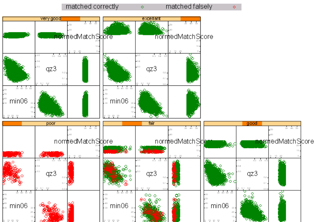
Figure 12. Trellis plot of min06 quality zone3 and normalized match scores of vendor F and right index fingerprints of dataset DOS-C
