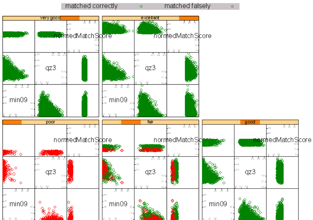
Figure 15. Trellis plot of min09 quality zone3 and normalized match scores of vendor F and right index fingerprints of dataset DOS-C
