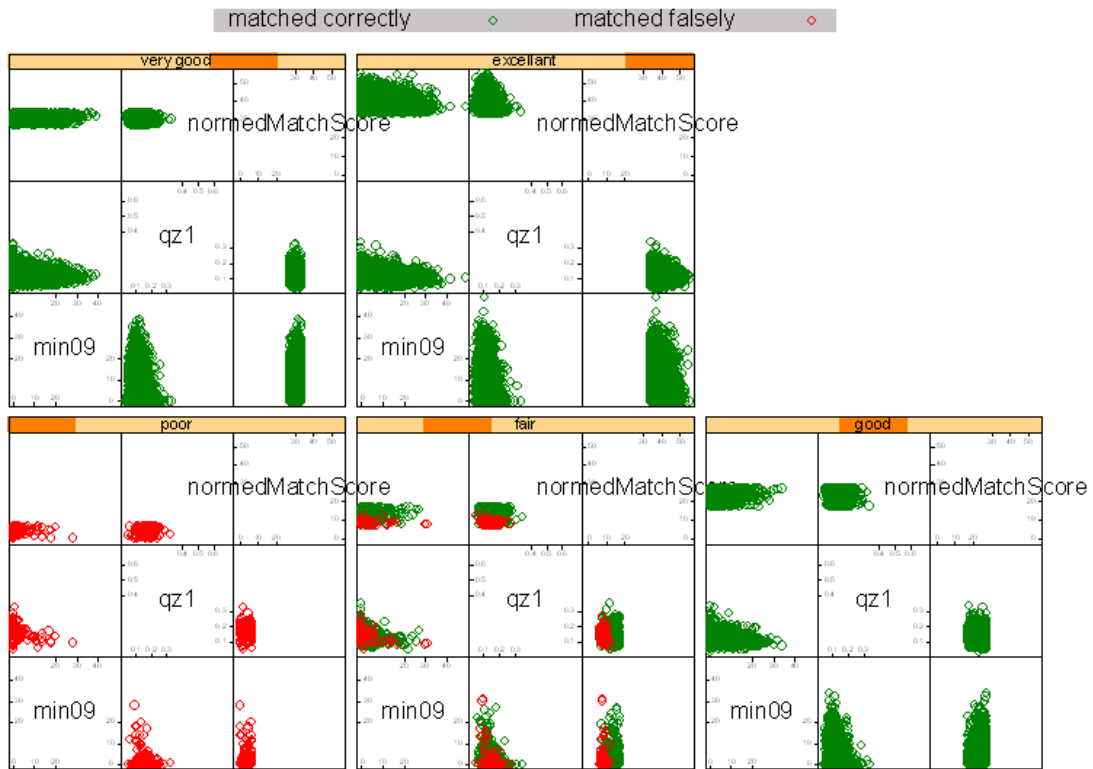
Figure 5. Trellis plot of min09 quality zone1 and normalized match scores of vendor F and right index fingerprints of dataset DOS-C
