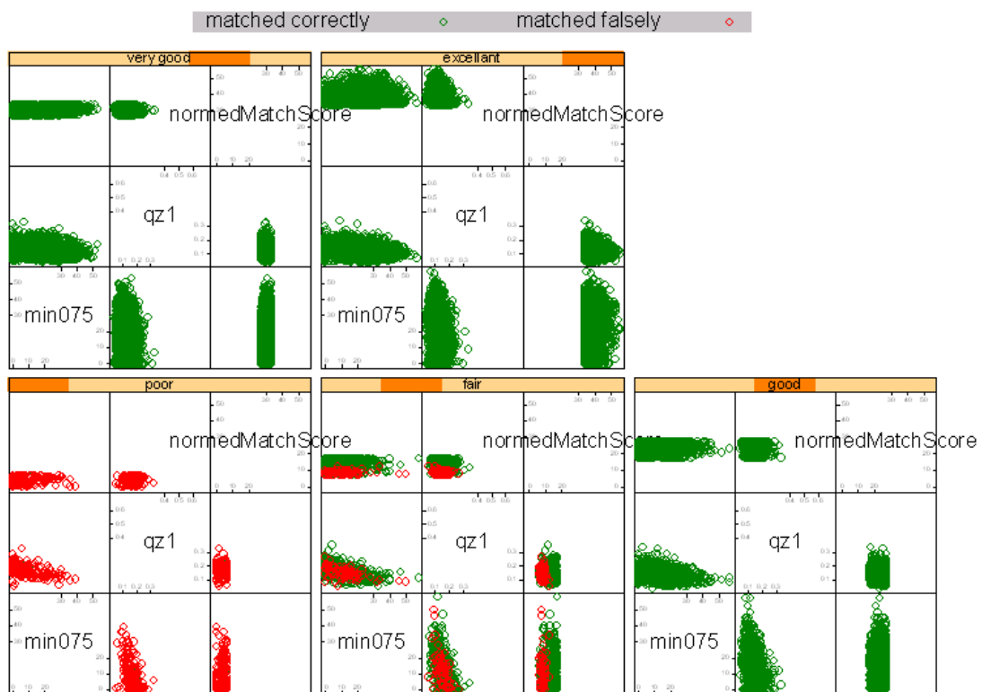
Figure 3. Trellis plot of min075 quality zone1 and normalized match scores of vendor F and right index fingerprints of dataset DOS-C
