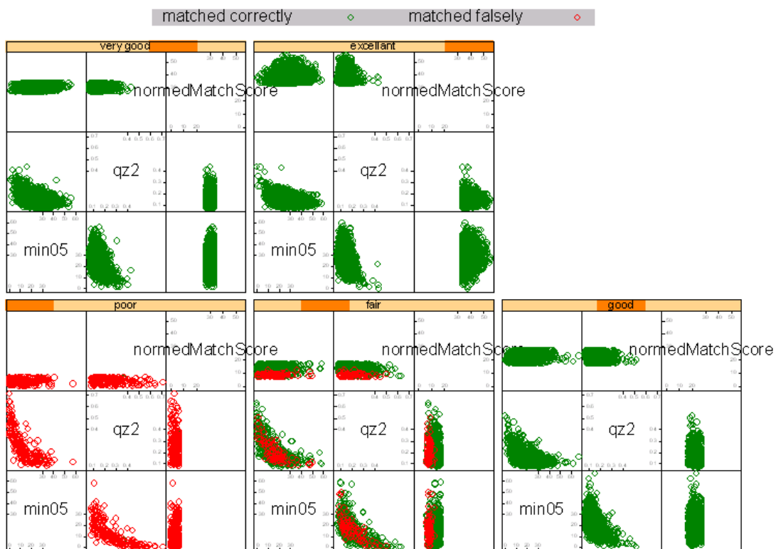
Figure 6. Trellis plot of min05 quality zone2 and normalized match scores of vendor F and right index fingerprints of dataset DOS-C
