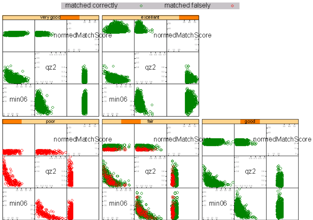
Figure 7. Trellis plot of min06 quality zone2 and normalized match scores of vendor F and right index fingerprints of dataset DOS-C
