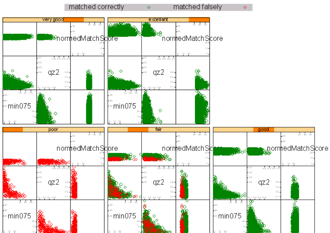
Figure 8. Trellis plot of min075 quality zone2 and normalized match scores of vendor F and right index fingerprints of dataset DOS-C
