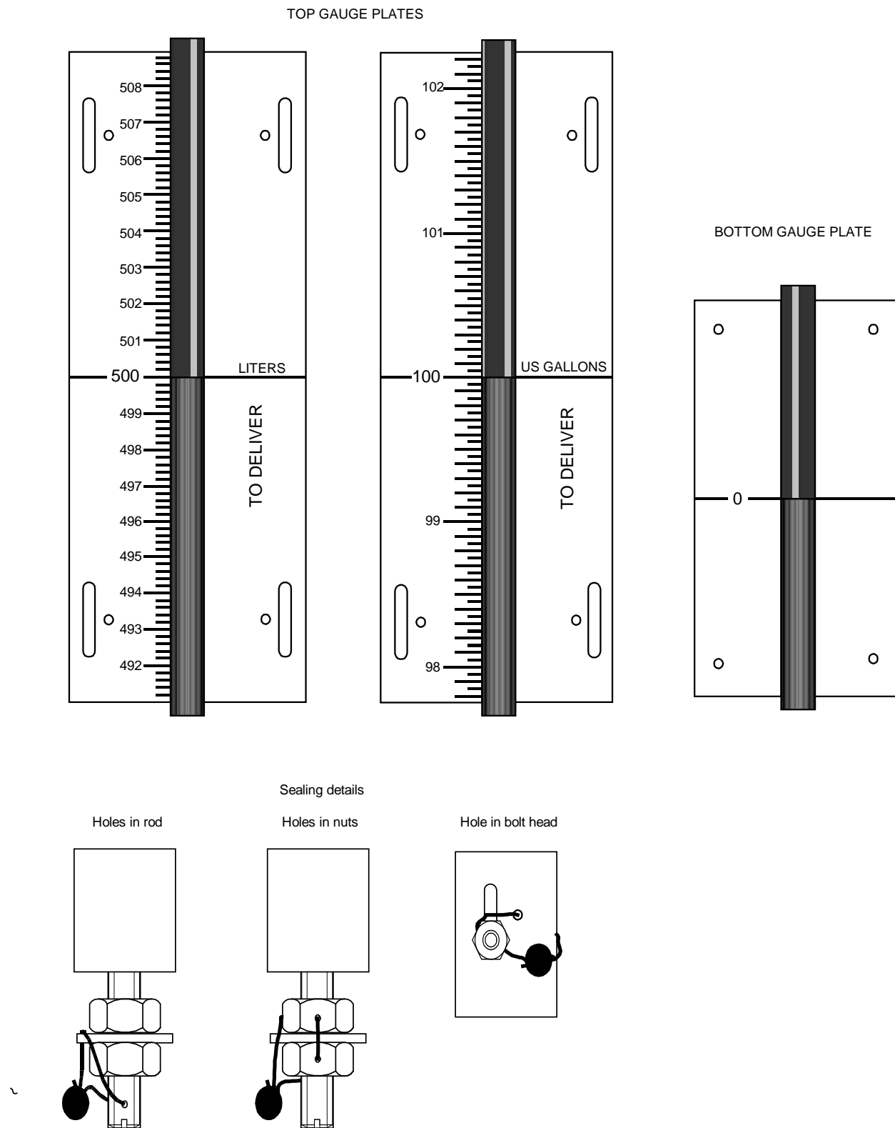
Figure 2. Schematic Drawing of Gauge Plates (Top and Bottom).
