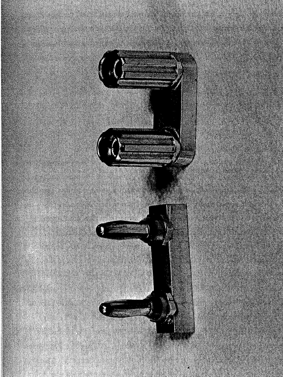
Figure 4 Shorting Bars
