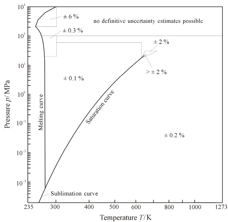
Figure B-3. Estimated uncertainties in isobaric heat capacity c_p . For the definition of the region around the critical point, see Figure B-1. The positions of the lines separating the uncertainty regions are approximate.
