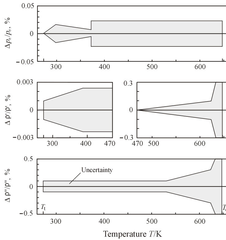
Figure B-4. Estimated uncertainties in vapor pressure p_v , saturated liquid density \rho' , and saturated vapor density \rho'' .
