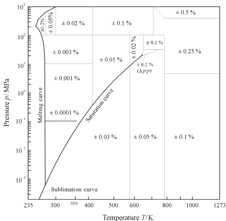
Figure B-1. Estimated uncertainties in density. In the enlarged critical region (triangle), a percent uncertainty in pressure is given. This region is bordered by the two isochores 527 \text{ kg}\cdot\text{m}^{-3} and 144 \text{ kg}\cdot\text{m}^{-3} and by the 30 MPa isobar. The positions of the lines separating the uncertainty regions are approximate.
