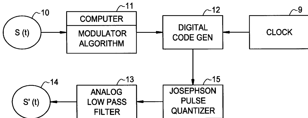
FIG. 2 PRIOR ART
