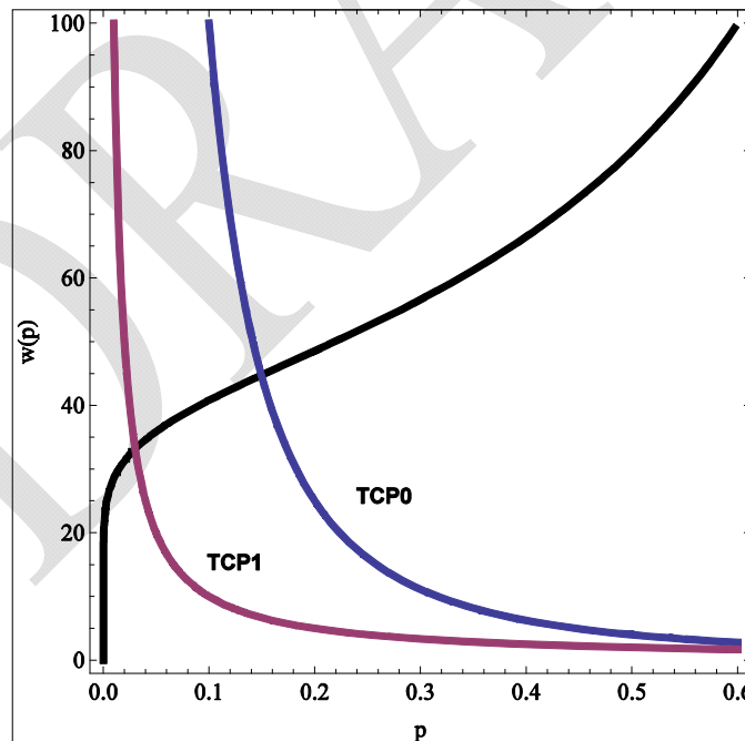
Figure A-1. Response curves of two hypothetical TCP variants TCP0 and TCP1 (blue and red) and the graph of a hypothetical packet loss function (black).
