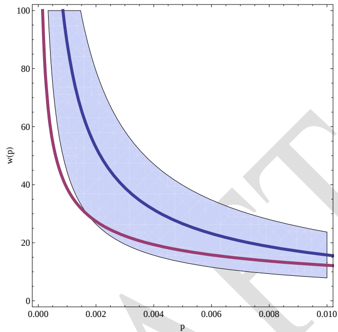
Figure A-2. CUBIC response curve and a \pm 50\% error region (blue) and TCP Reno response curve (red).
