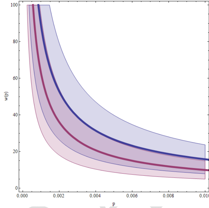
Figure A-4. CUBIC (thick blue) and CTCP (thick red) response curves and corresponding error regions.
