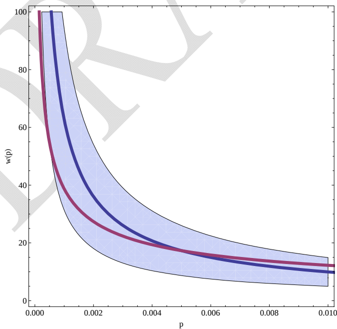
Figure A-3. CTCP response curve and a \pm 50\% error region (blue) and TCP Reno response curve (red).
