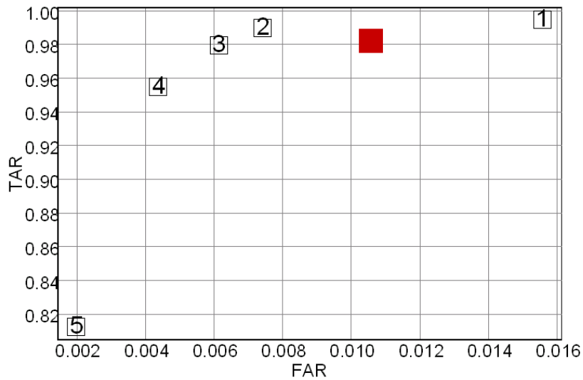
Figure 3. The effect of quality on ROC - Vendor N - Dataset VISIT_POE_BVA - Left Index
