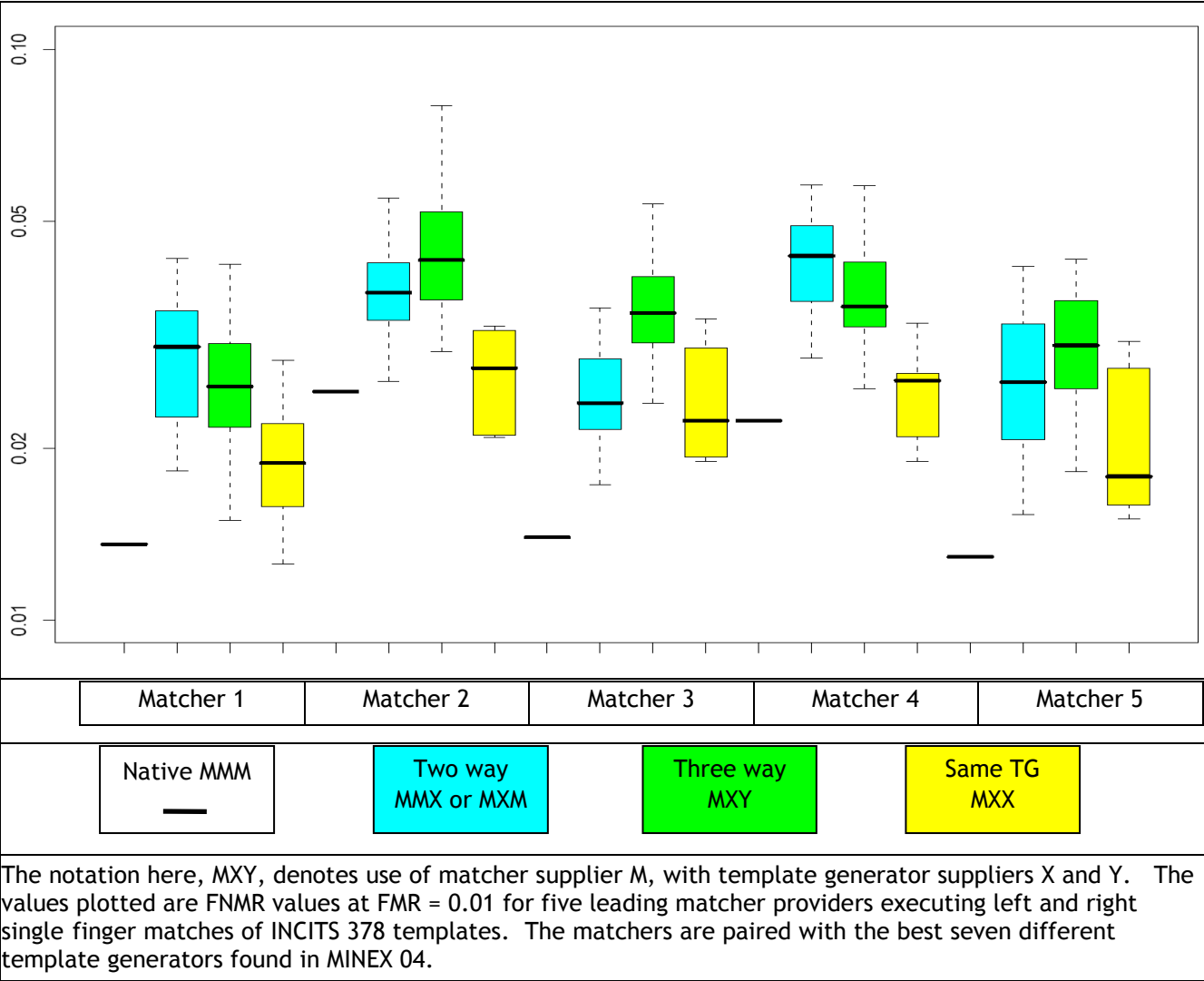
Figure 4 - Native vs. Two-way vs. Three-way Interoperability
