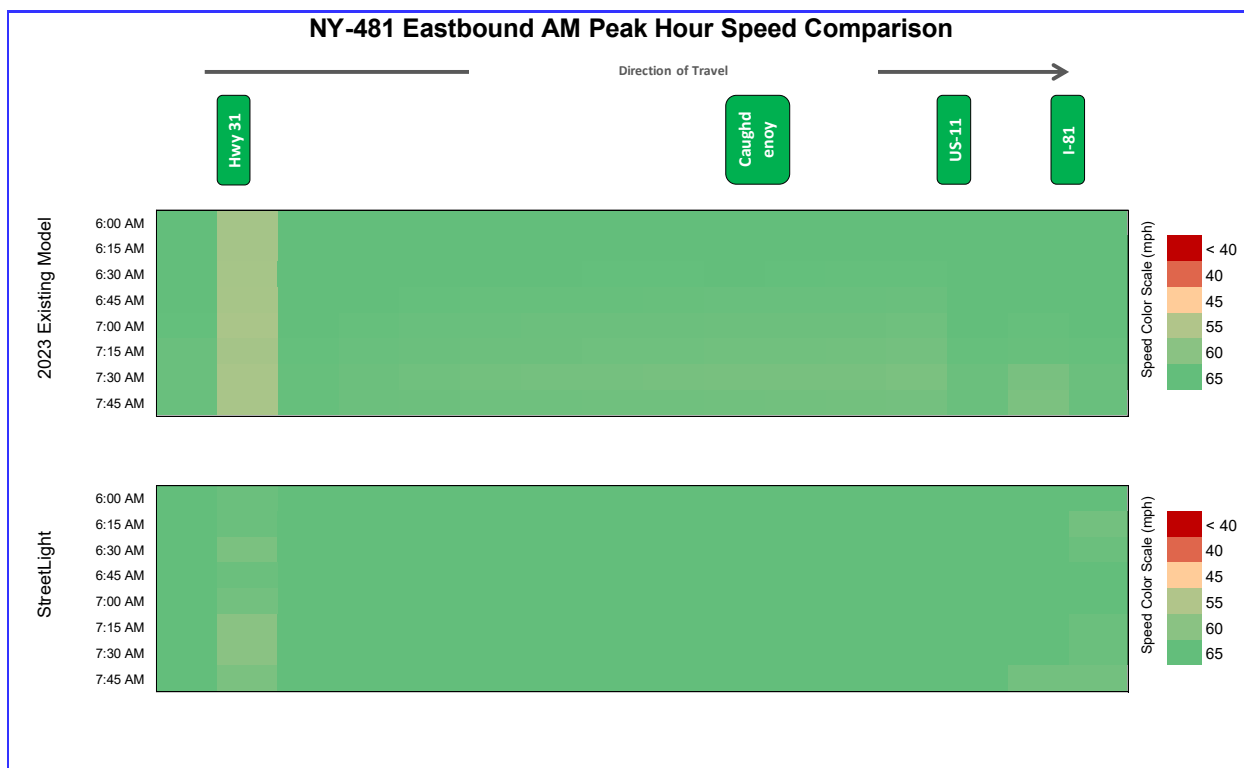
Figure 5-7. NY-481 Eastbound Speed Congestion Diagram, AM Peak Hour
