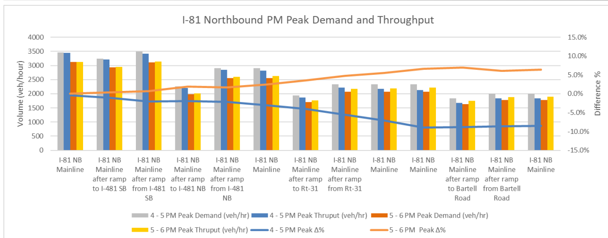
Figure 6-2. Existing I-81 Northbound PM Peak Hour Demand and Throughput
