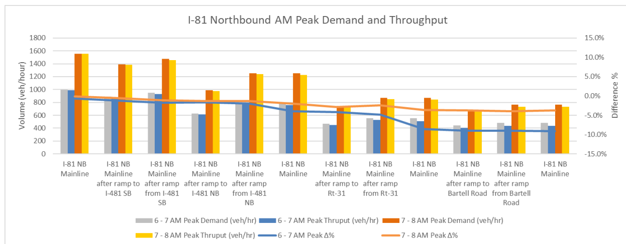
Figure 5-2. Existing I-81 Northbound AM Peak Hour Demand and Throughput
