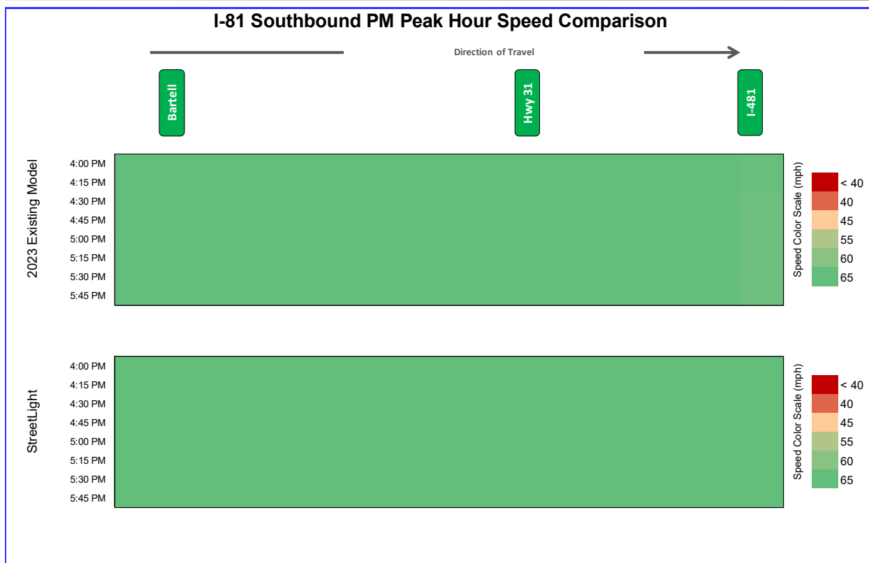
Figure 6-9. I-81 Southbound Speed Congestion Diagram, PM Peak Period
