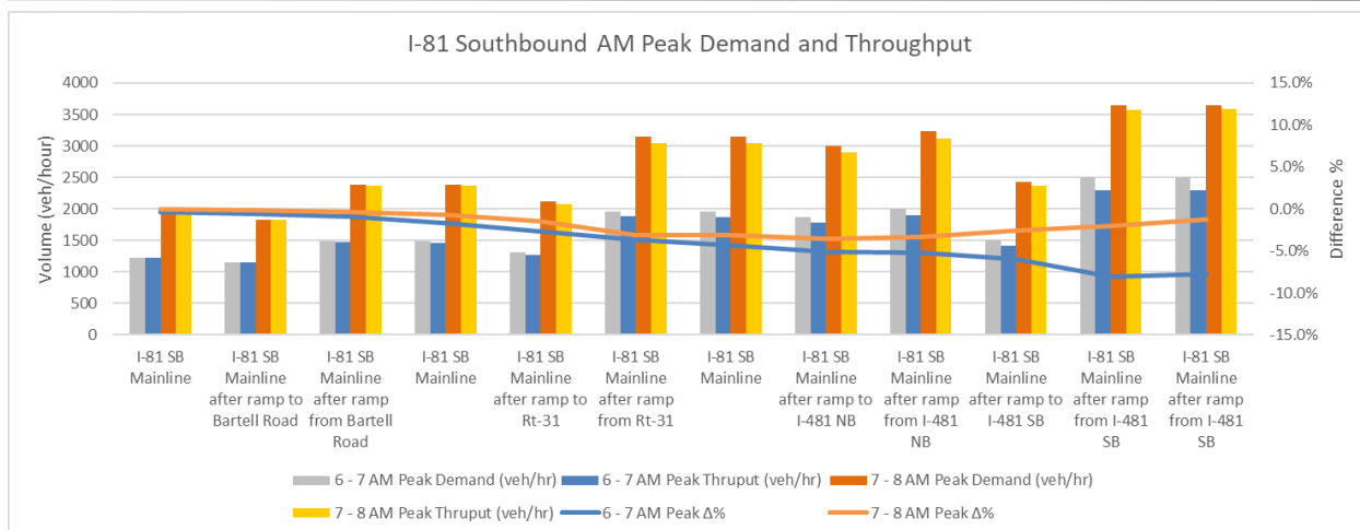
Figure 5-3. Existing I-81 Southbound AM Peak Hour Demand and Throughput
