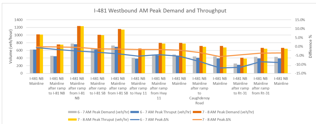
Figure 5-4. Existing NY-481 Westbound AM Peak Hour Demand and Throughput
