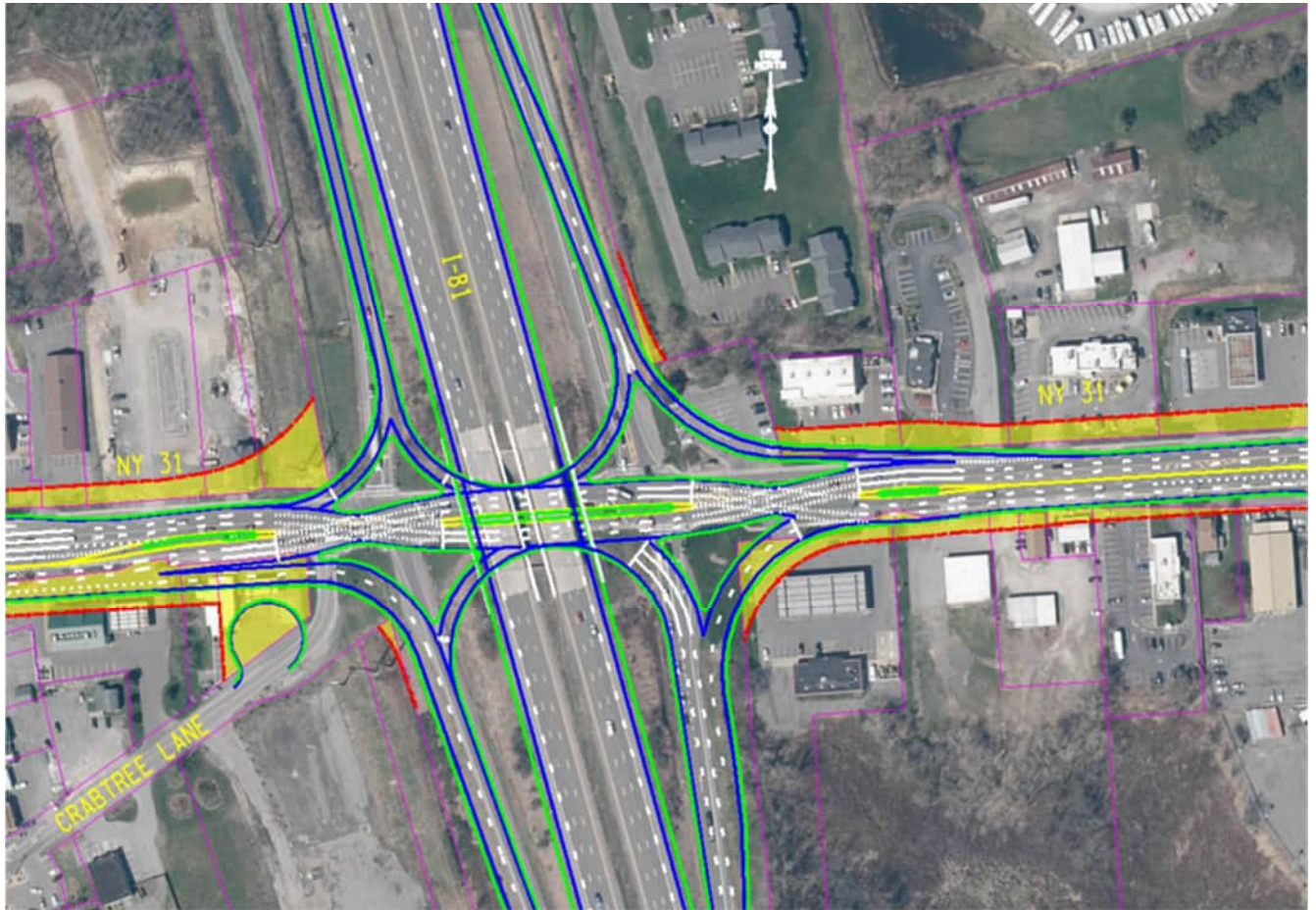
Figure 3: I-81 &amp; NY 31 DDI Concept
