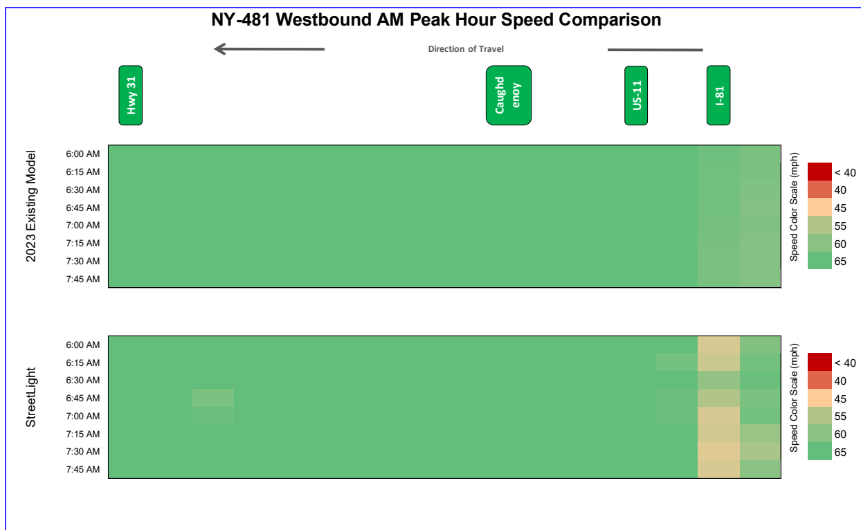
Figure 5-6. NY-481 Westbound Speed Congestion Diagram, AM Peak Hour
