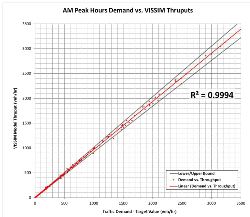
Figure 5-1. Field Volumes vs. VISSIM Throughputs – AM Peak Hour
