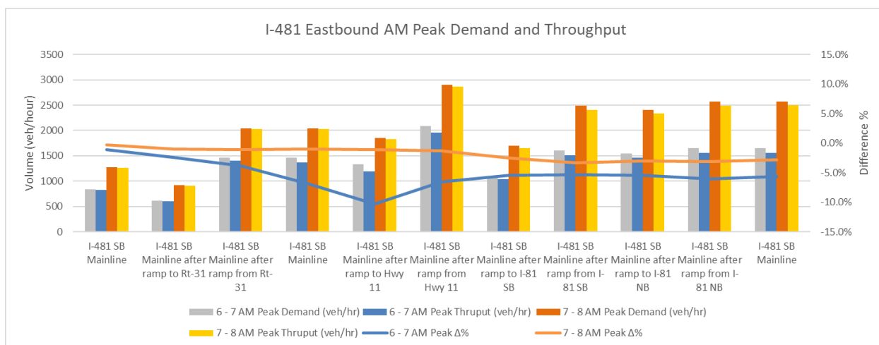
Figure 5-5. Existing NY-481 Eastbound AM Peak Hour Demand and Throughput
