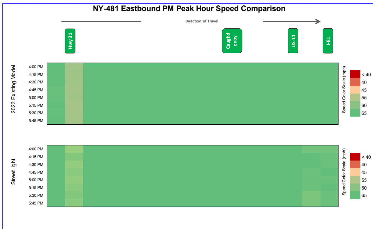
Figure 6-7. NY-481 Eastbound Speed Congestion Diagram, PM Peak Period
