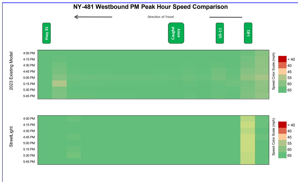
Figure 6-6. NY-481 Westbound Speed Congestion Diagram, PM Peak Period
