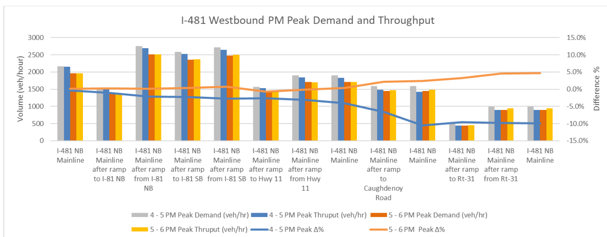
Figure 6-4. Existing NY-481 Westbound PM Peak Hour Demand and Throughput
