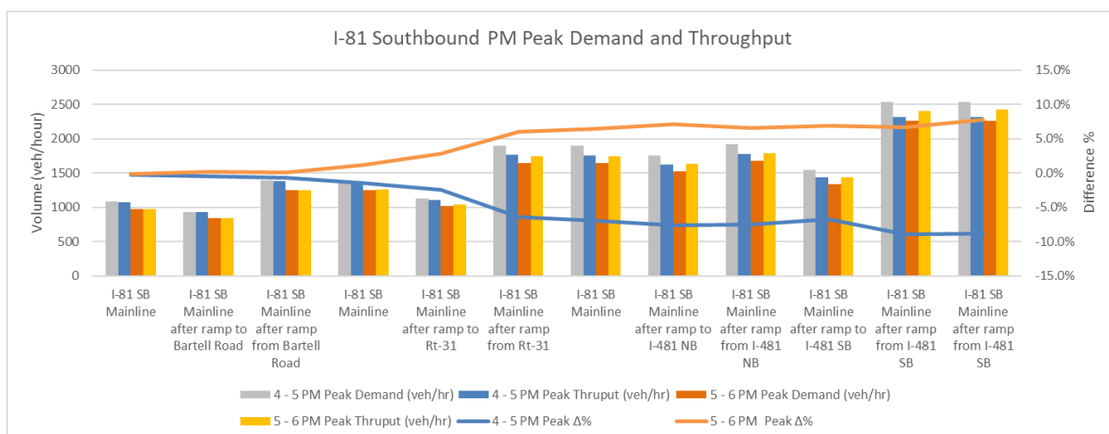
Figure 6-3. Existing I-81 Southbound PM Peak Hour Demand and Throughput
