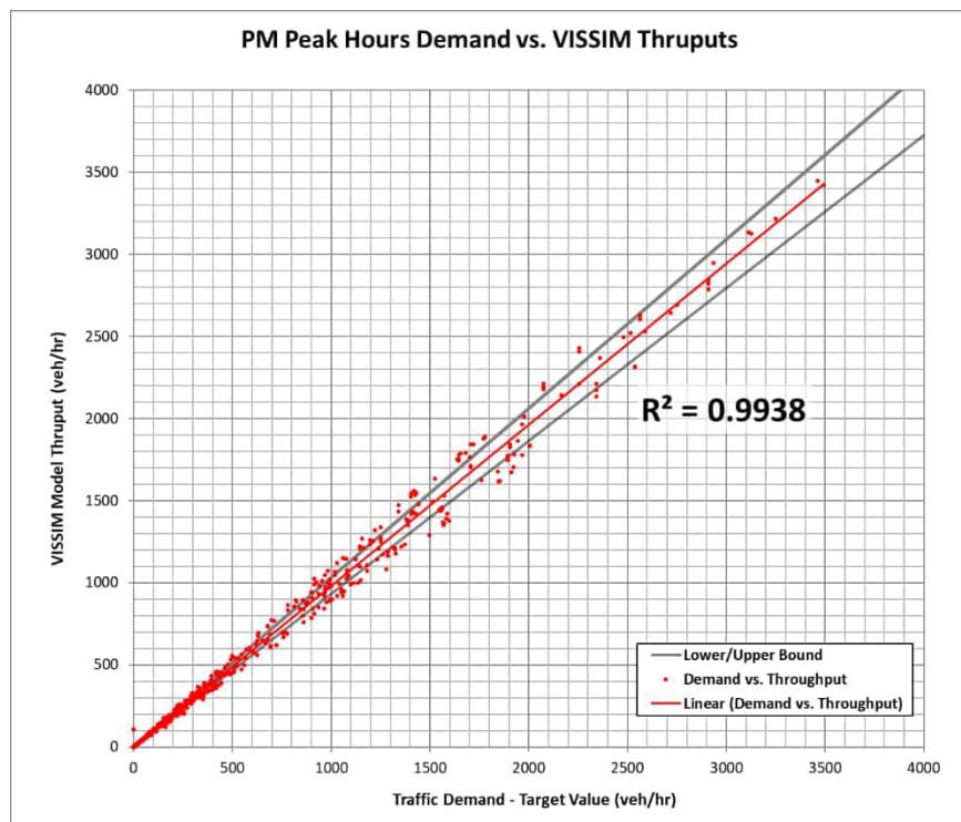
Figure 6-1. Field Volumes vs. VISSIM Throughputs – PM Peak Hour
