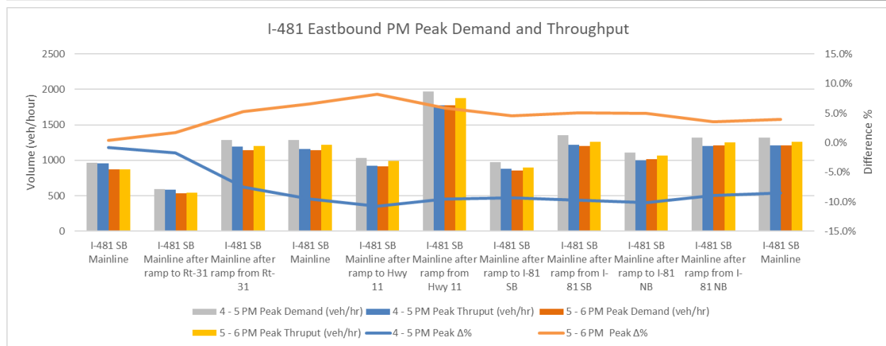
Figure 6-5. Existing NY-481 Eastbound PM Peak Hour Demand and Throughput
