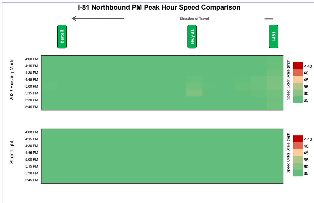
Figure 6-8. I-81 Northbound Speed Congestion Diagram, PM Peak Period
