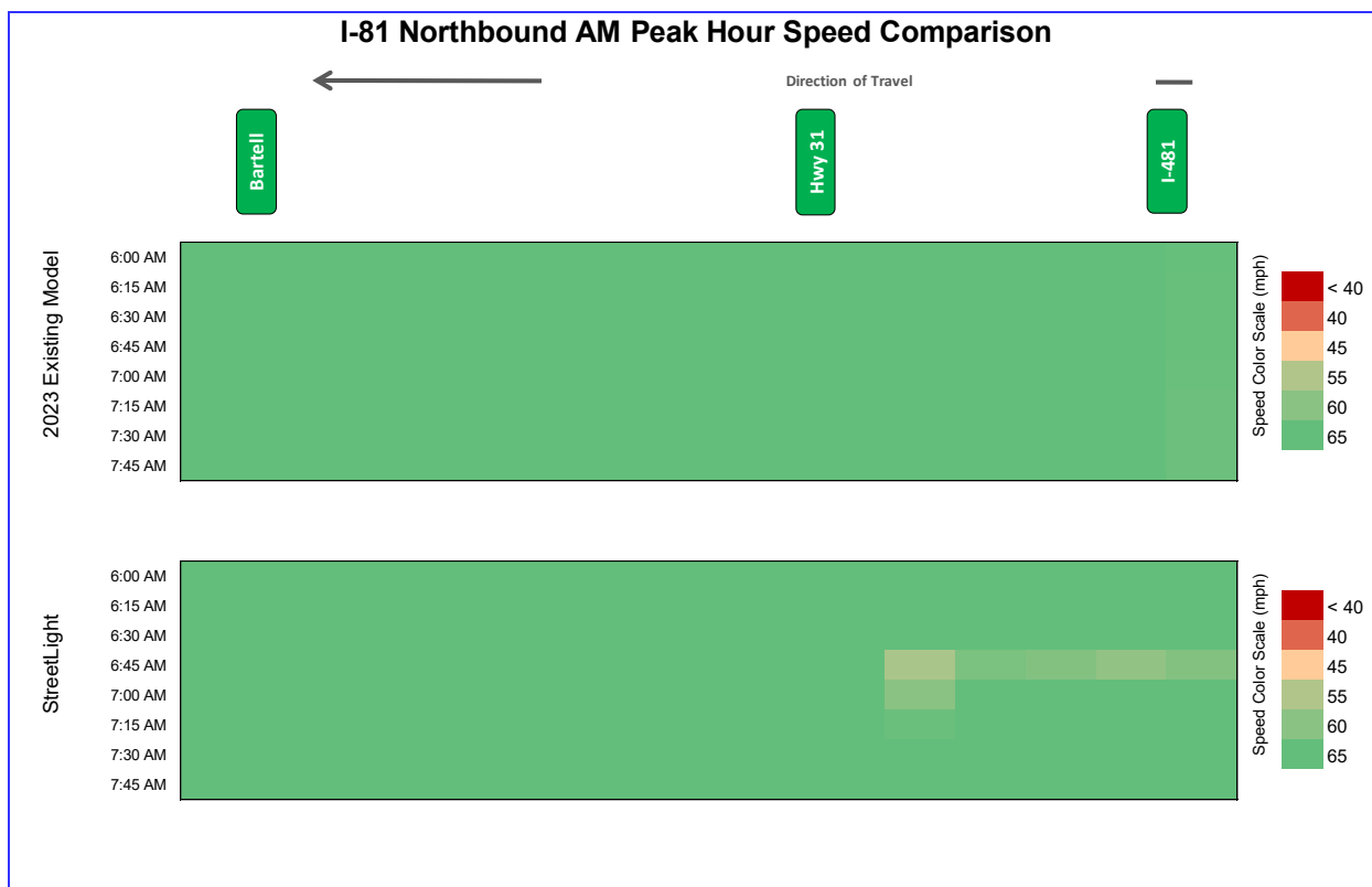
Figure 5-8. I-81 Northbound Speed Congestion Diagram, AM Peak Hour
