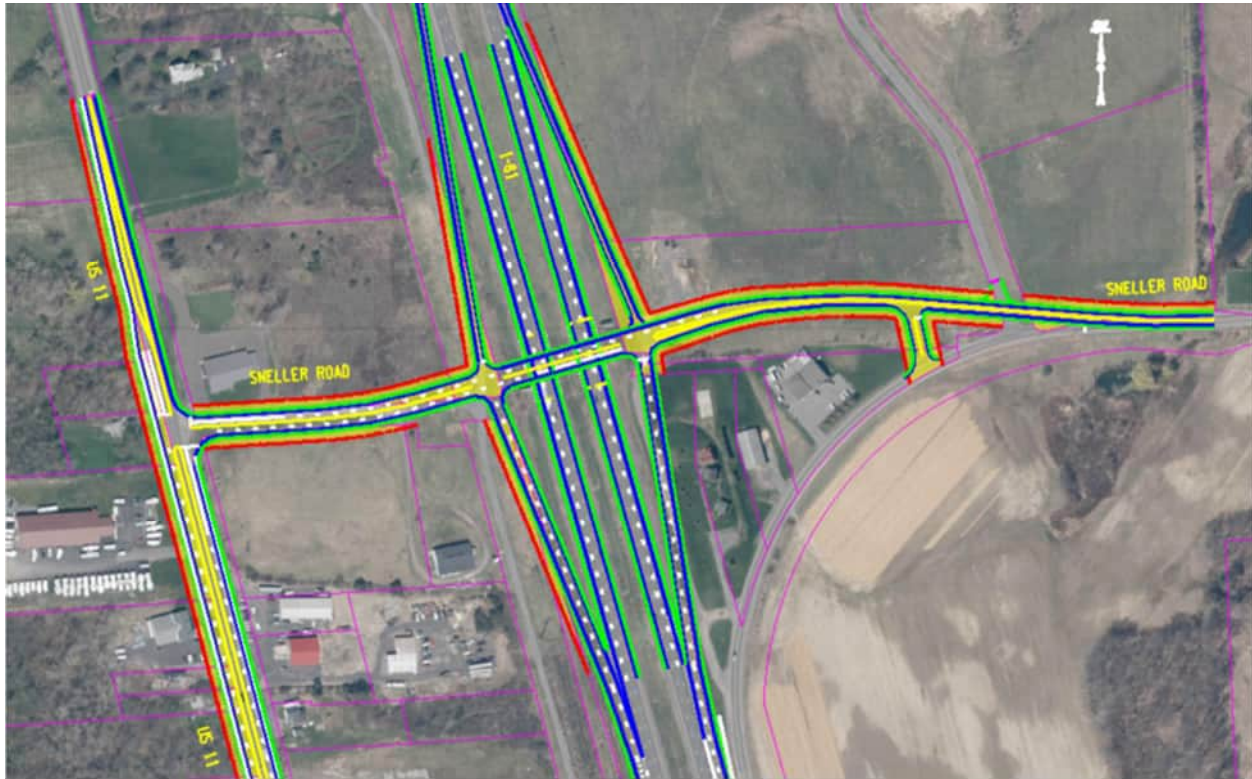
Figure 12: New Sneller Road Interchange Concept
