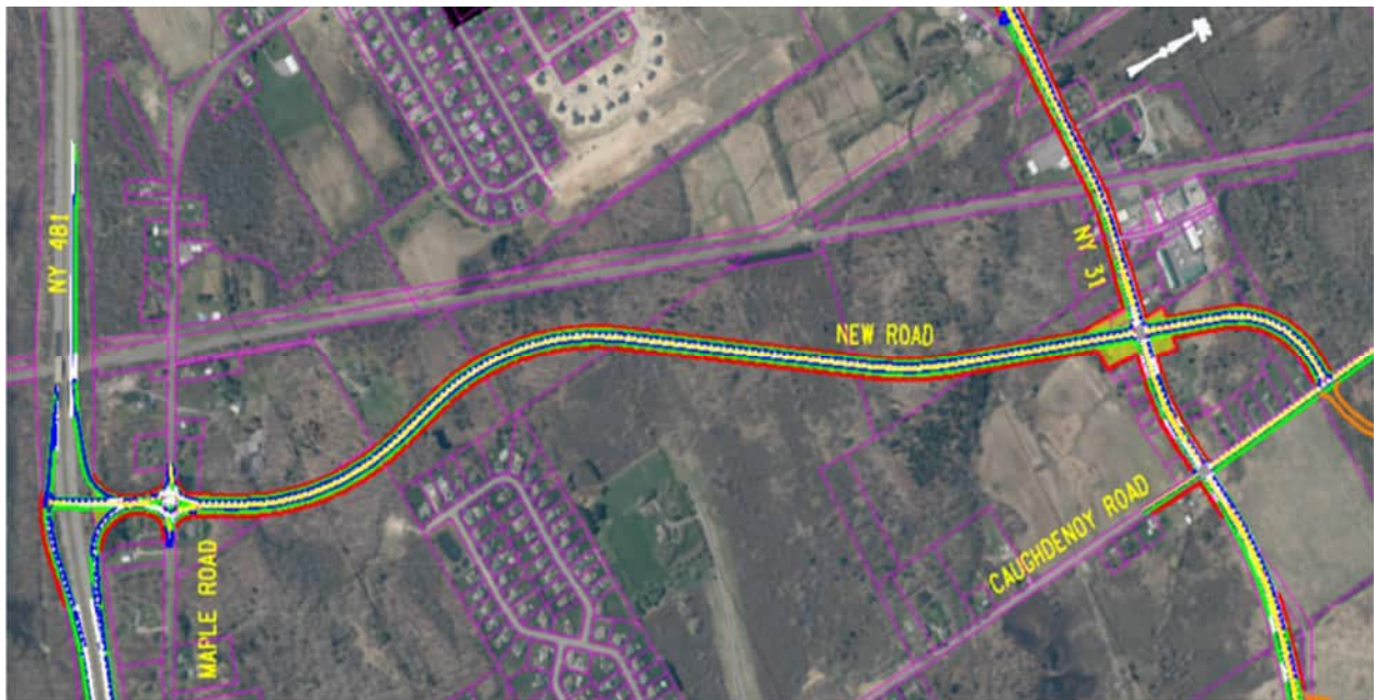
Figure 18: New NY 481 Interchange Roadway Concept
