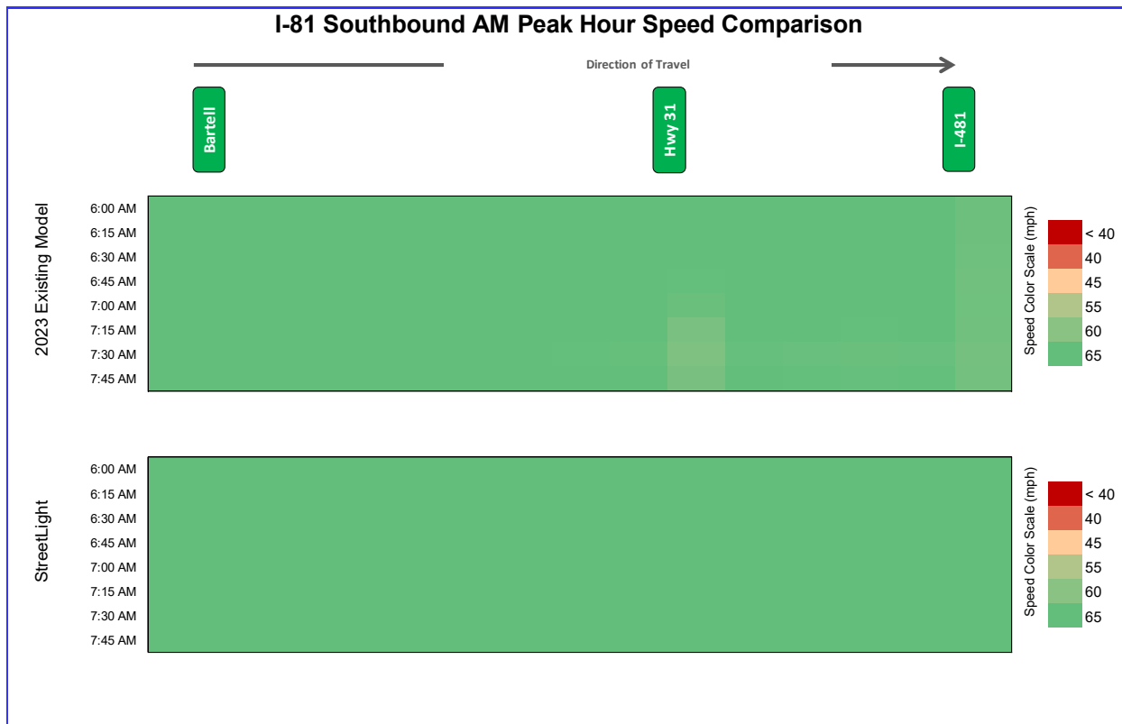
Figure 5-9. I-81 Southbound Speed Congestion Diagram, AM Peak Hour
