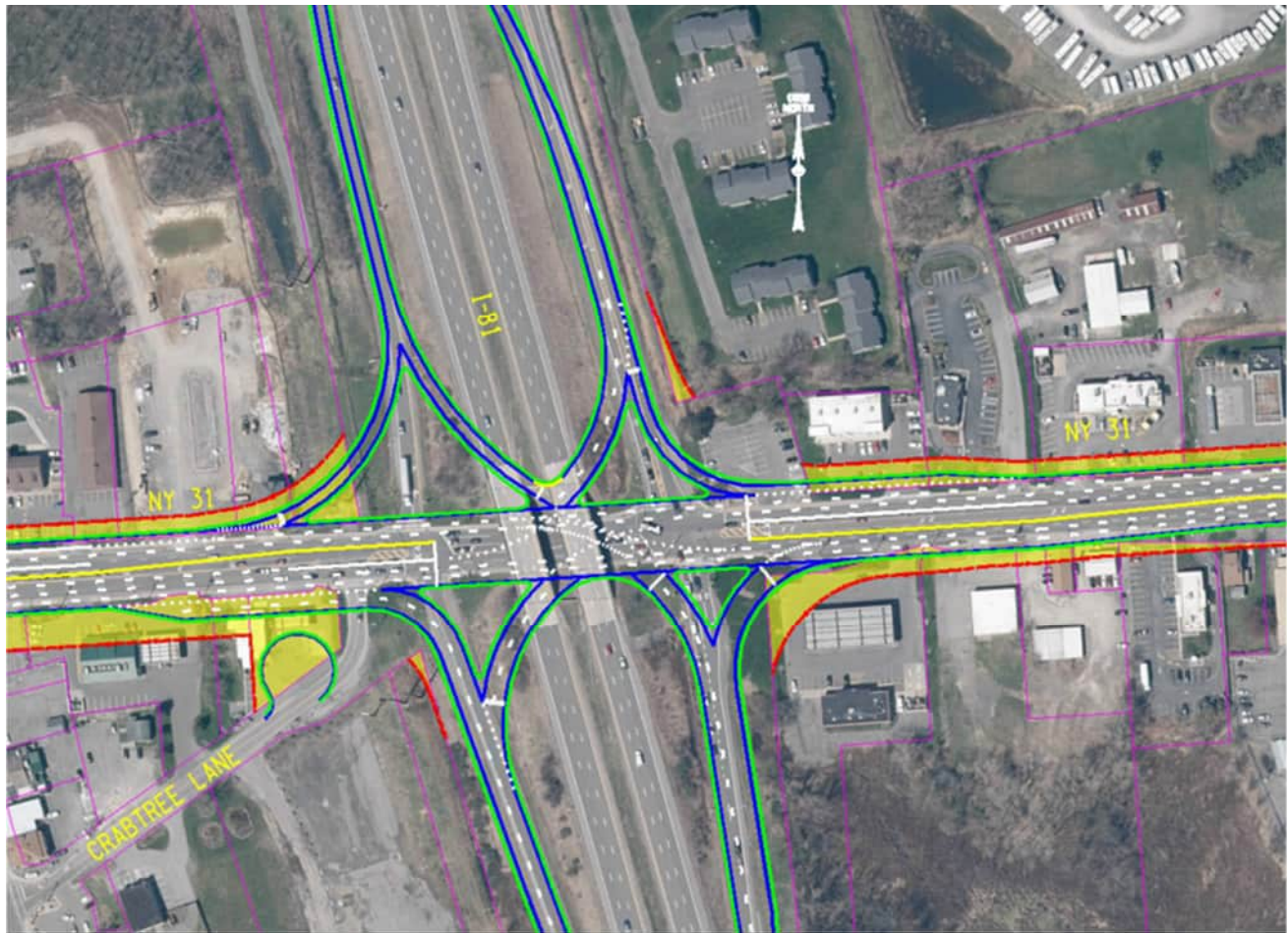
Figure 4: I-81 &amp; NY 31 SPUI Concept
