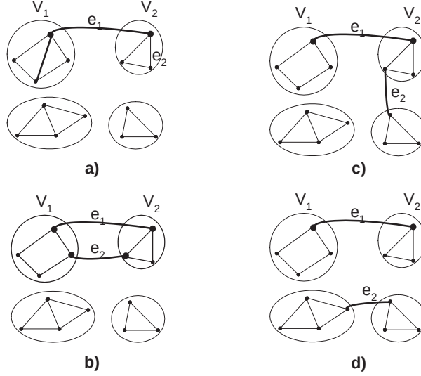
Figure 7: Illustrative proof of the submodularity: possible scenarios when e_1 is a bridge in G \setminus (E + e_2) .
