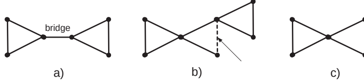
Figure 9: Examples of simple graphs that are not 2-vertex connected.
