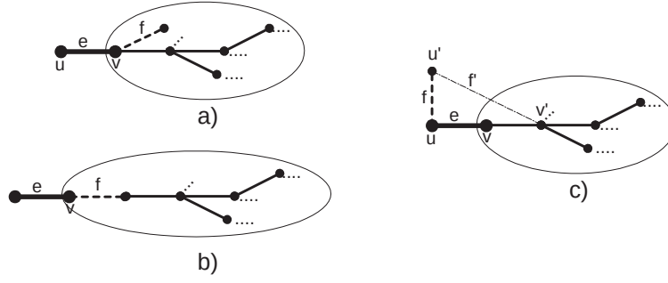
Figure 10: Illustrative figures for the proof of Lemma 6: building a spanning tree T such that T - \{e\} = T_1 \cup T_{n-1} .
