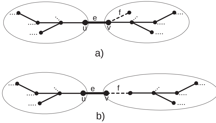
Figure 11: Illustrative figures for the proof of Lemma 6: building a spanning tree T such that T - \{e\} = T_{n_1} \cup T_{n_2} .
