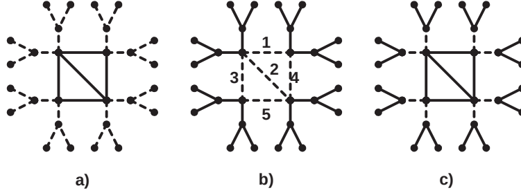
Figure 2: Example of critical subsets for different value models. a) GWA model b) OBT, Walrand, and Metcalfe's models. c) Reed's model.
