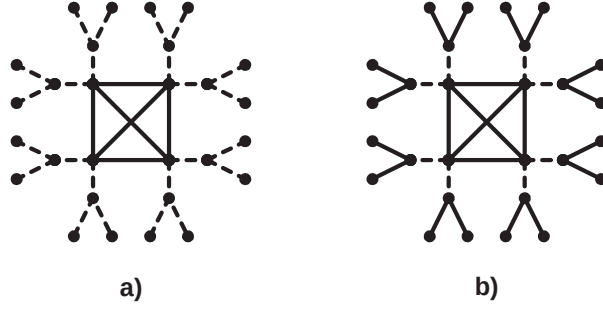
Figure 4: Example of critical subsets for different value models. a) GWA model b) OBT, Walrand, and Metcalfe's models. c) Reed's model
