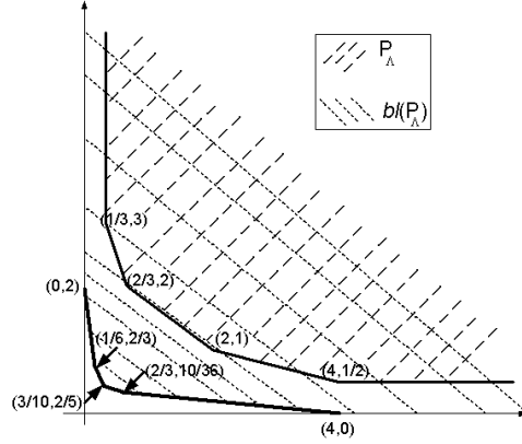
Figure 5: Example of polyhedron P_\Lambda defined by a nonnegative proper matrix \Lambda and its corresponding blocker bl(P_\Lambda) . The extreme points of the blocker define the nonnegative proper matrix \Omega .
