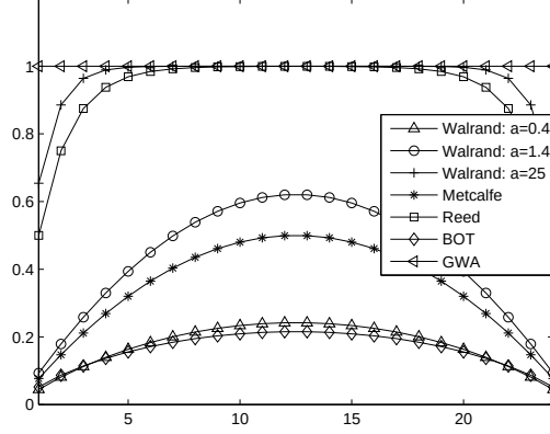
Figure 3: Comparison of the loss functions 1 - \frac{f(n_1) + f(n-n_1)}{f(n)} when a link belonging to the chosen spanning tree is cut, dividing it into 2 subtrees of n_1 and n - n_1 nodes. For GWA, since \lambda_{Te} = \mathbf{1}_{e \in T} , the loss is always 1. The models GWA, Reed, and Walrand (for large values of a ), overlap in a wide region of values of n_1 .
