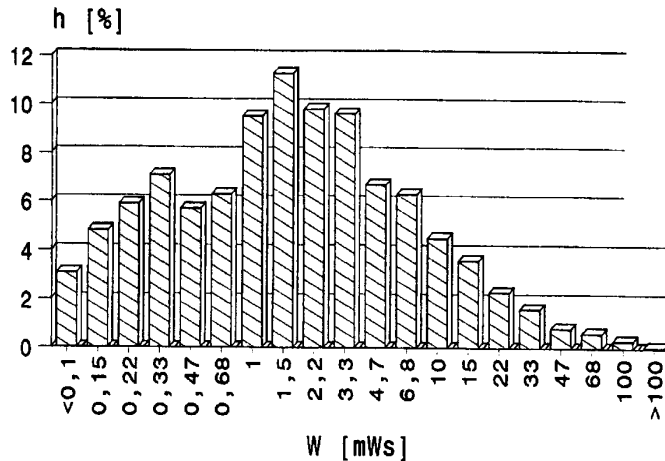
Figure 1 - Example of report of survey results 14 with number of occurrences as a function of “energy” in milliwatts-seconds
