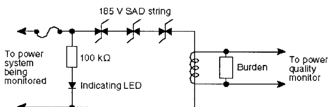
Figure 2 - Schematic of the transducer
