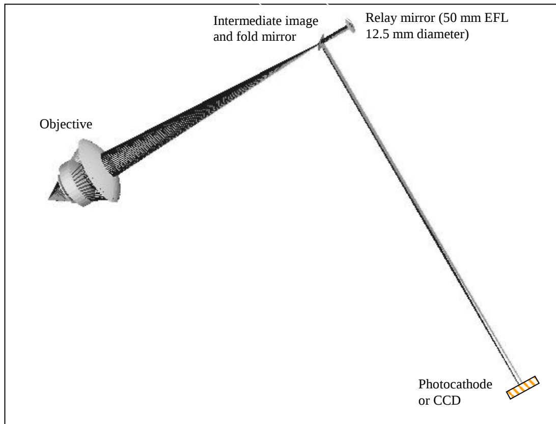
Figure 1. Imaging optics systems layout with the catadioptric objective and spherical relay mirror.
