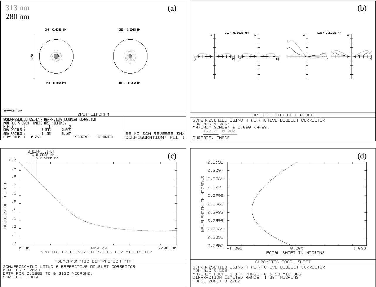
Figure 3. Predicted performance of the optimized catadioptric objective in the object space: (a) Two-wavelength spot diagrams for center and edge of FOV. (b) Two-wavelength OPD fan diagrams for center and edge of FOV. (c) Two-wavelength diffraction modulated transfer functions for center and edge of FOV in comparison to the diffraction limit. (d) Chromatic focal shift.
