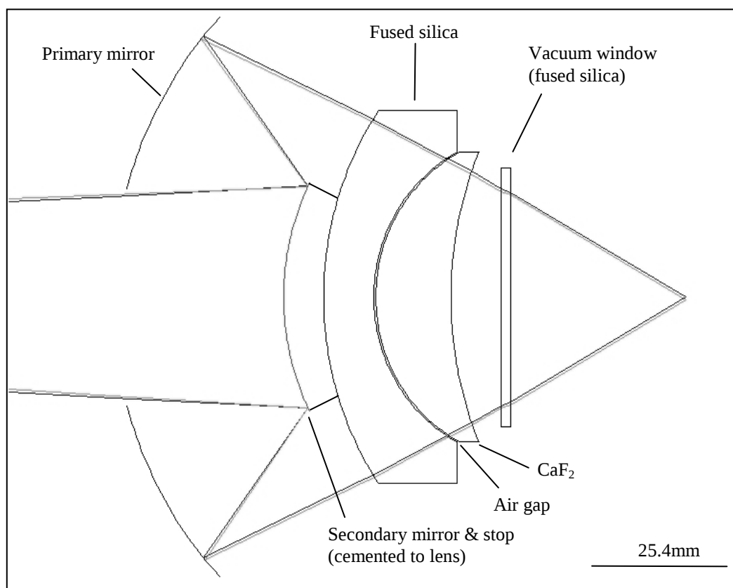
Figure 2. Optimized catadioptric design form of the achromatic microscope objective.
