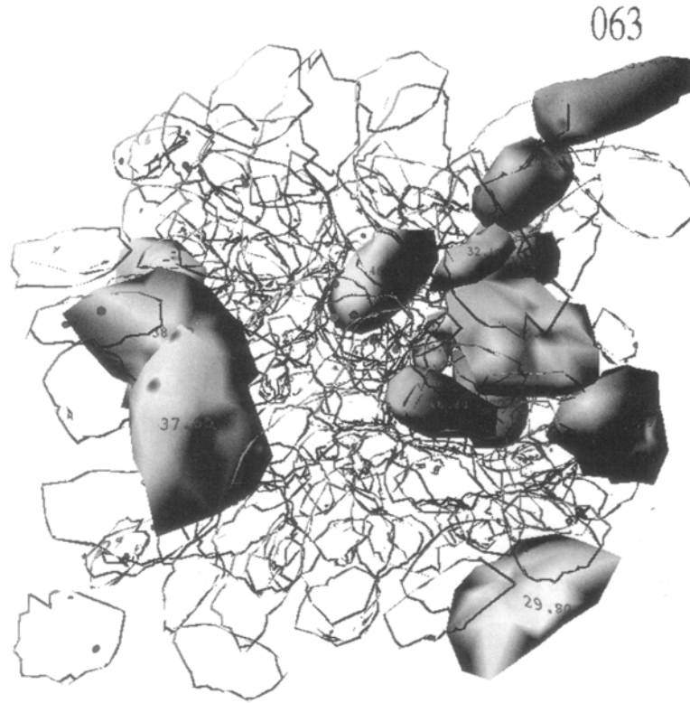
Fig. 13.4 Frame 63 in a simulation of the flow of rocks in a suspension. Lower stress rocks are shown in sketch mode
