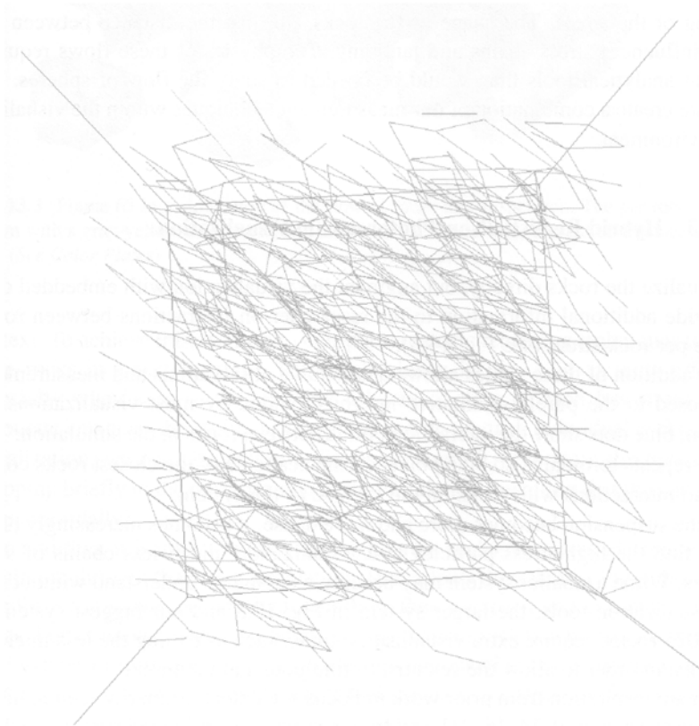
Fig. 13.2 Stress in flows of spherical objects. The spheres are not shown, but are centered at the endpoints of each line segment. Stress chains show the structure of the stress field
