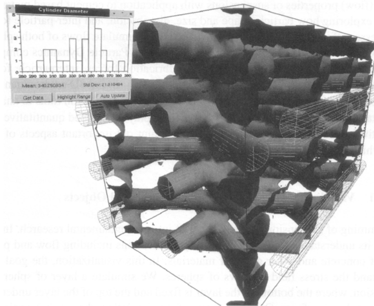
Fig. 13.1 Cylinder measurement and analysis tool used on rendered objects derived from measured data taken from a tissue engineering scaffold (See Color Plates)
