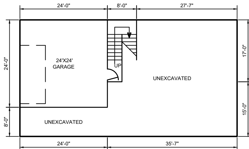
GARAGE
