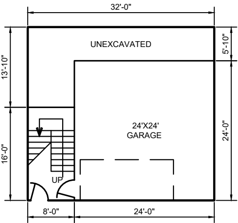
GARAGE
