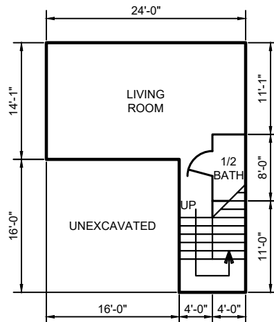
BASEMENT/FIRST FLOOR
