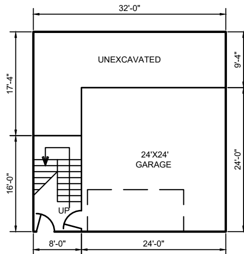
GARAGE
