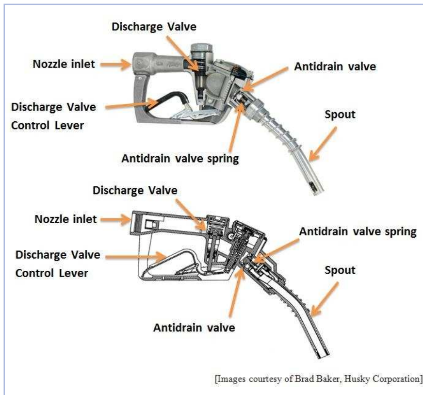
Figure 2. Internal Components of a Typical Fuel Dispenser Nozzle
