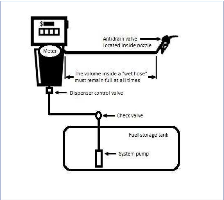
Figure 1. Fuel Dispenser System with Wet Hose
