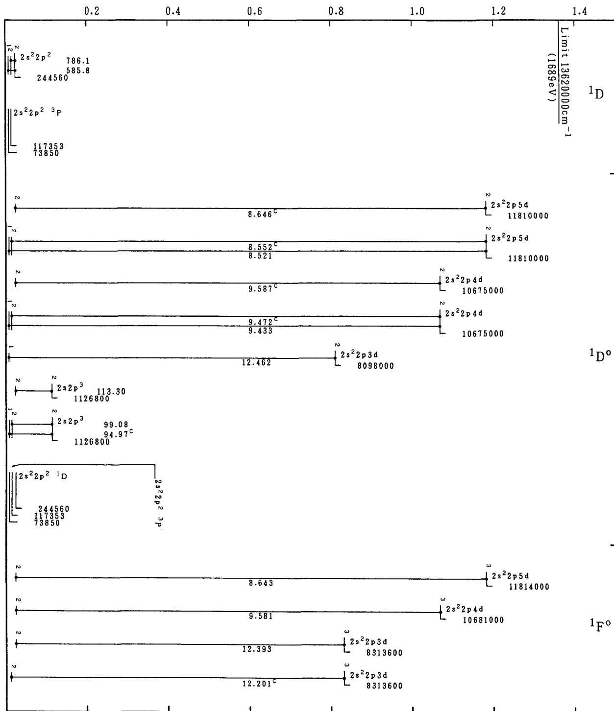
Grotrian Diagrams for Fe XXI (C-Sequence)-Continued
