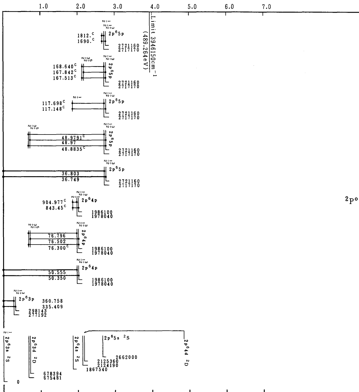
Grotrian Diagrams for Fe XVI (Na-Sequence)-Continued
