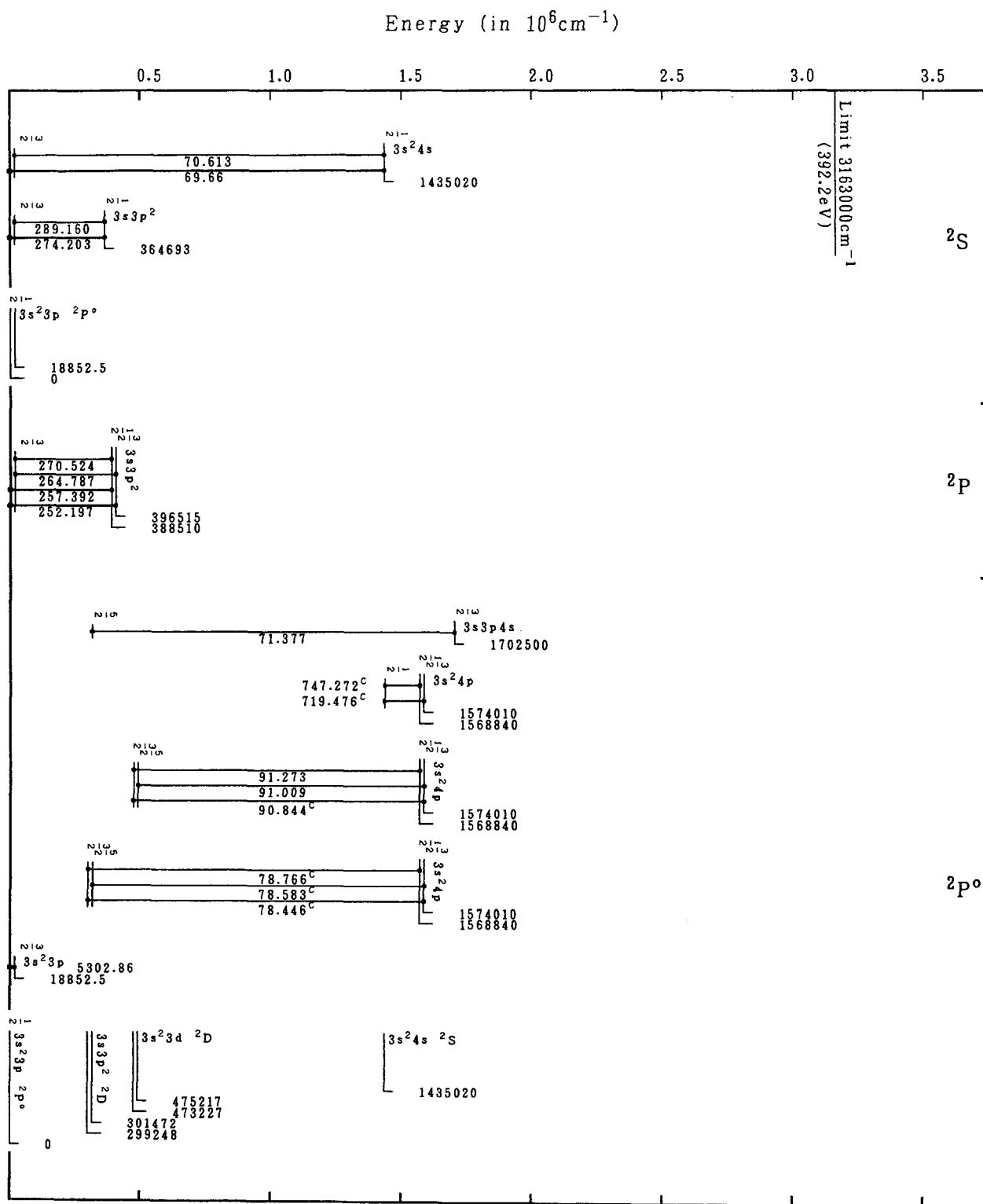
Grotrian Diagrams for Fe XIV (Al-Sequence)
