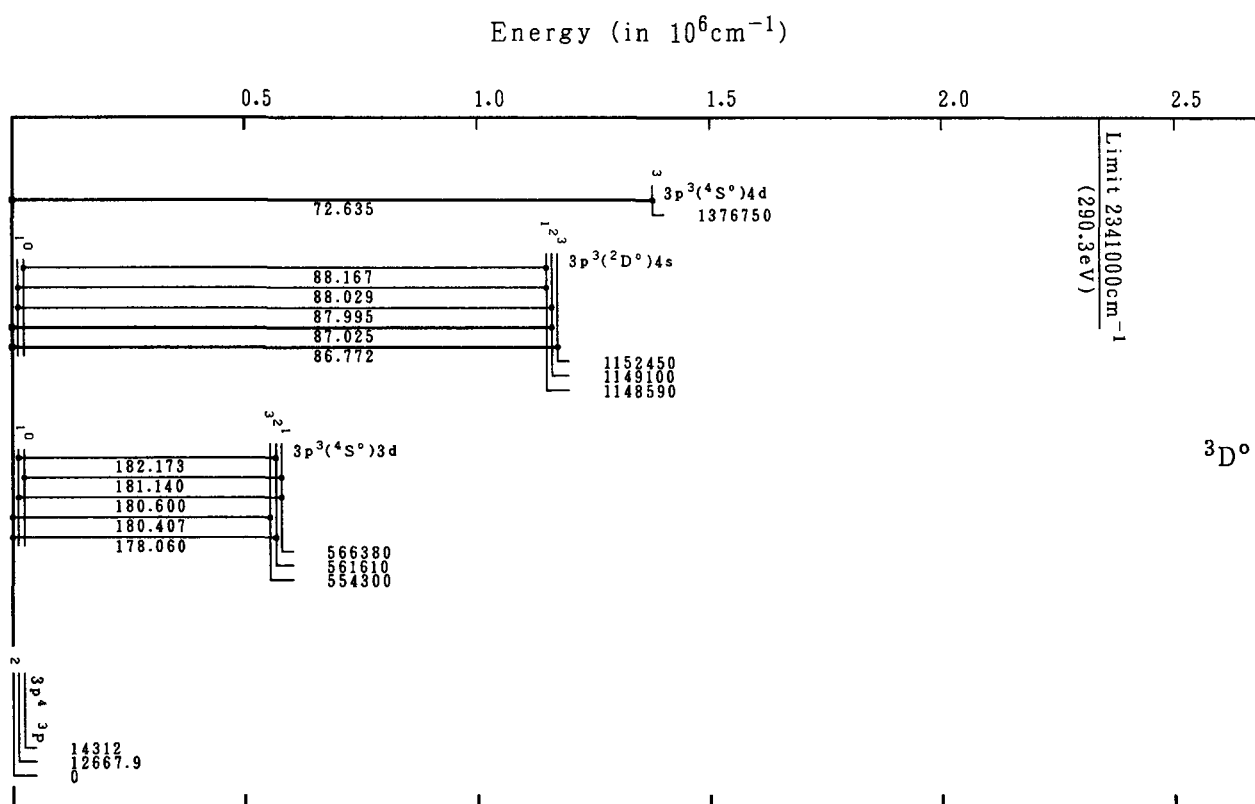
Grotrian Diagrams for Fe XI (S-Sequence)-Continued
