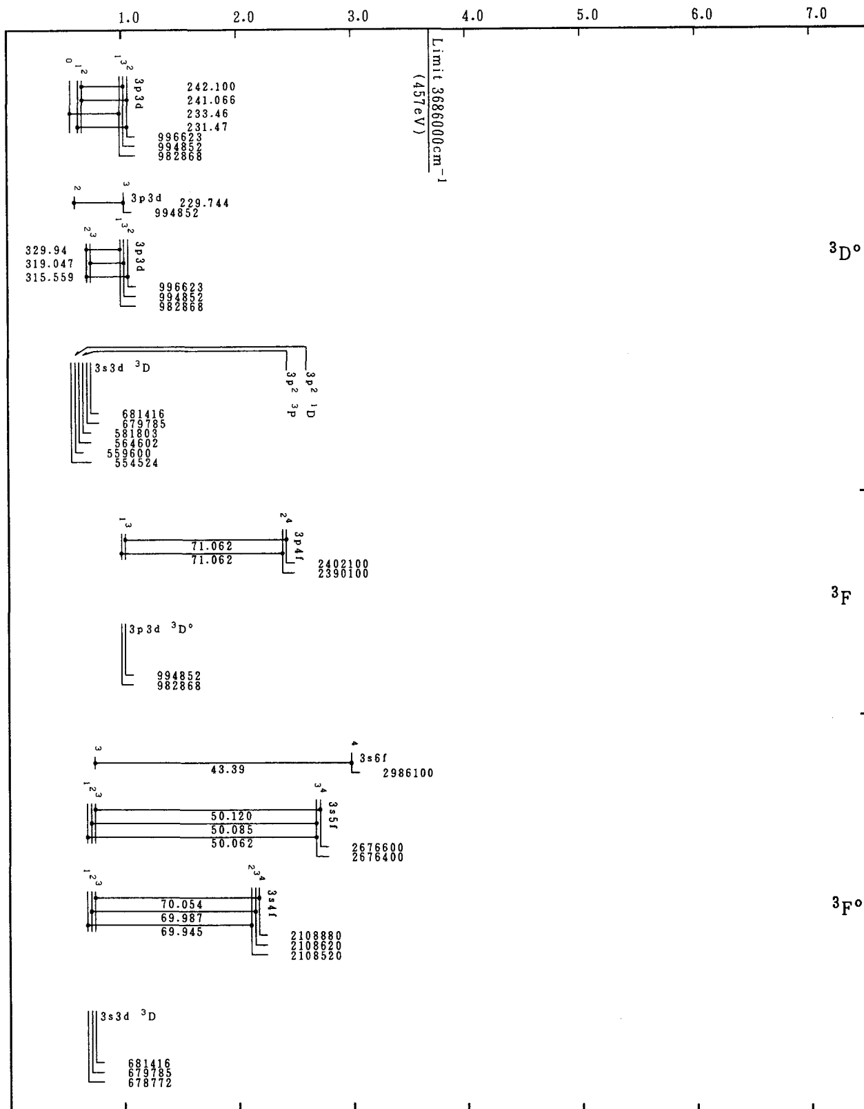
Grotrian Diagrams for Fe XV (Mg-Sequence)-Continued
