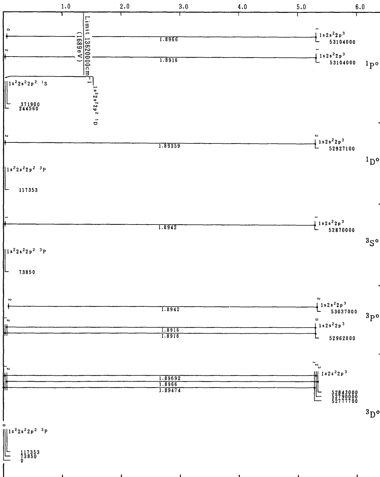
Grotrian Diagrams for Fe XXI (C-Sequence)-Continued
