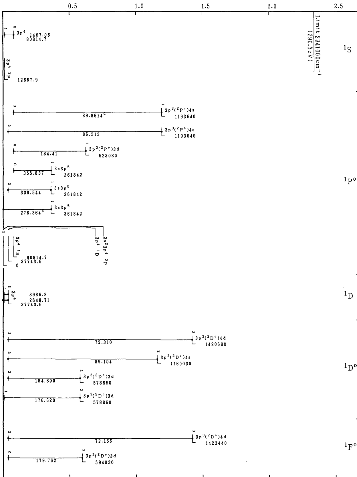
Grotrian Diagrams for Fe XI (S-Sequence)
