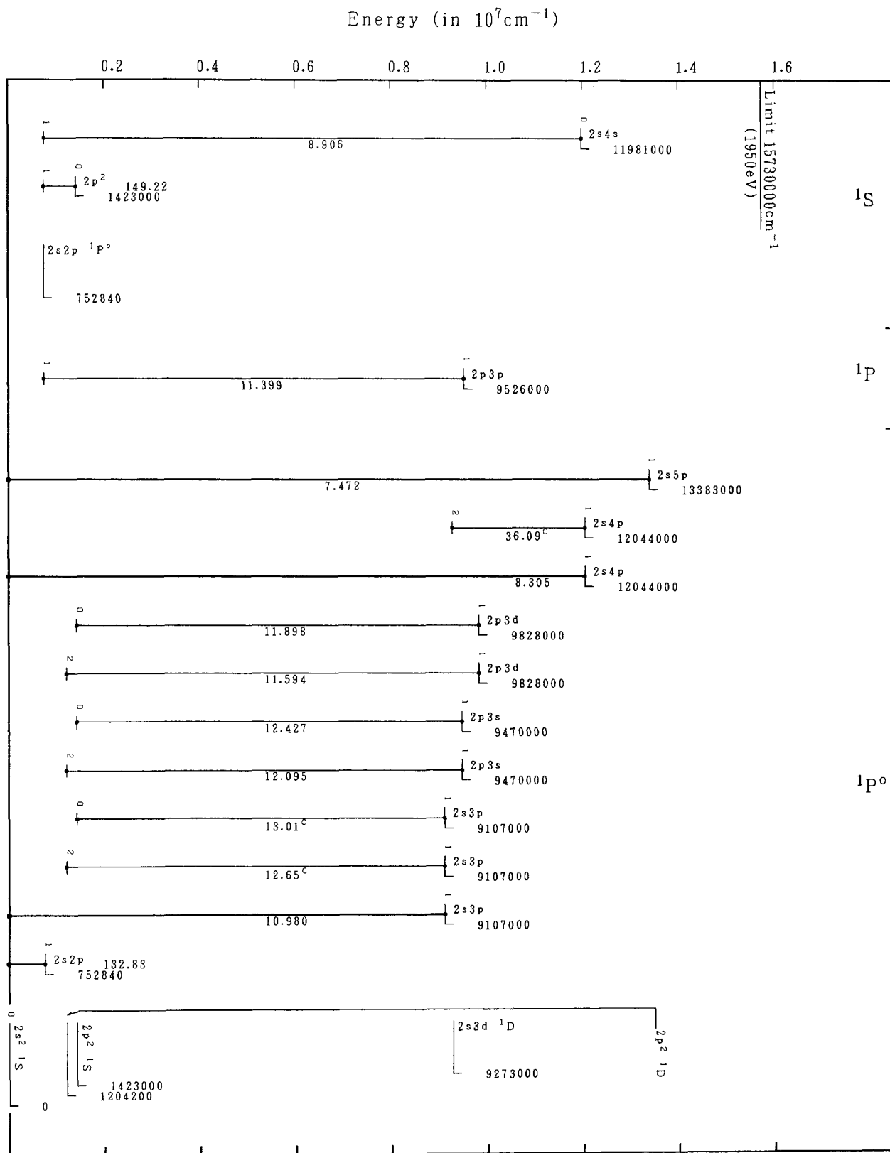
Grotrian Diagrams for Fe XXIII (Be-Sequence)
