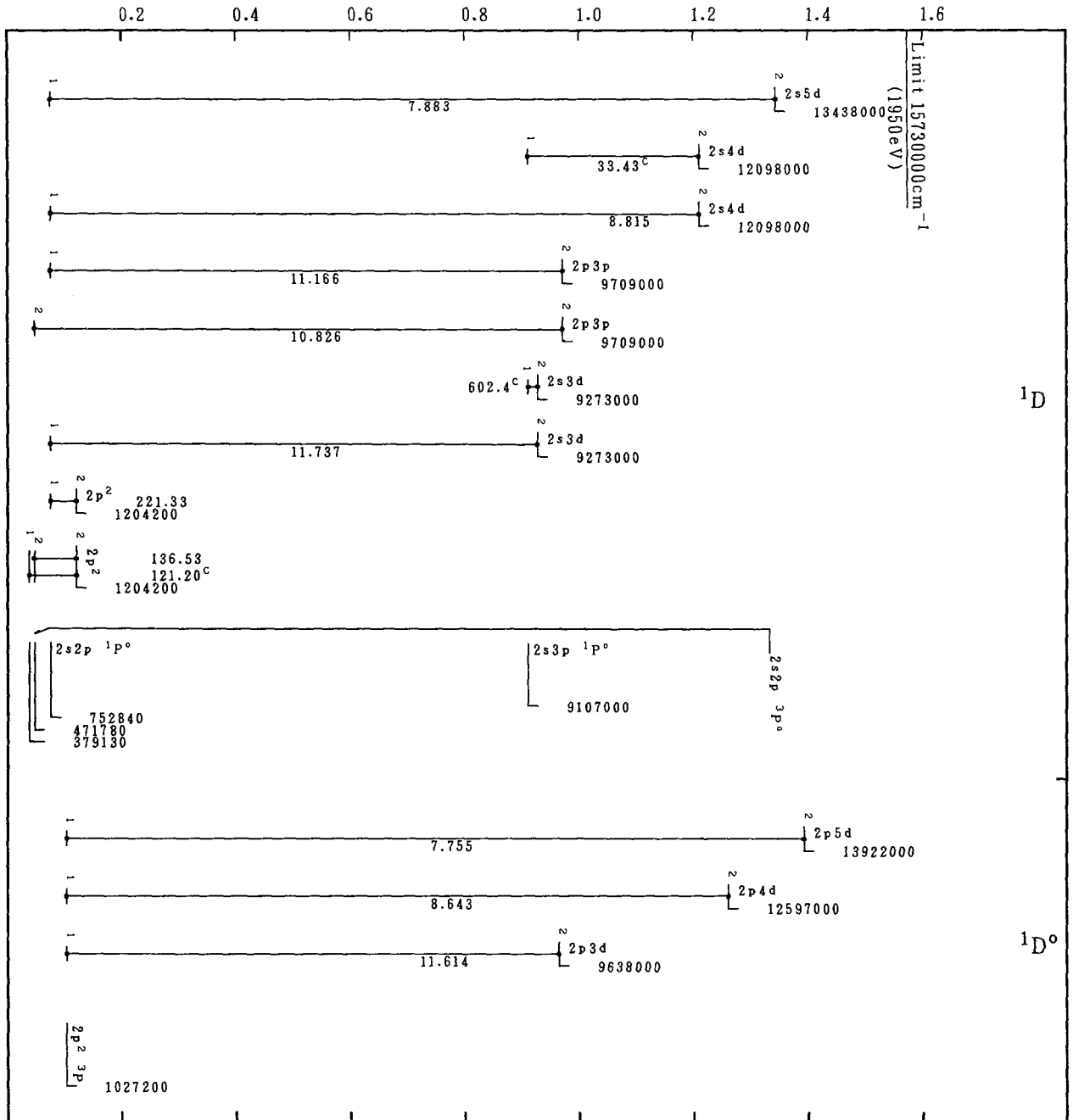
Grotrian Diagrams for Fe XXIII (Be-Sequence)-Continued
