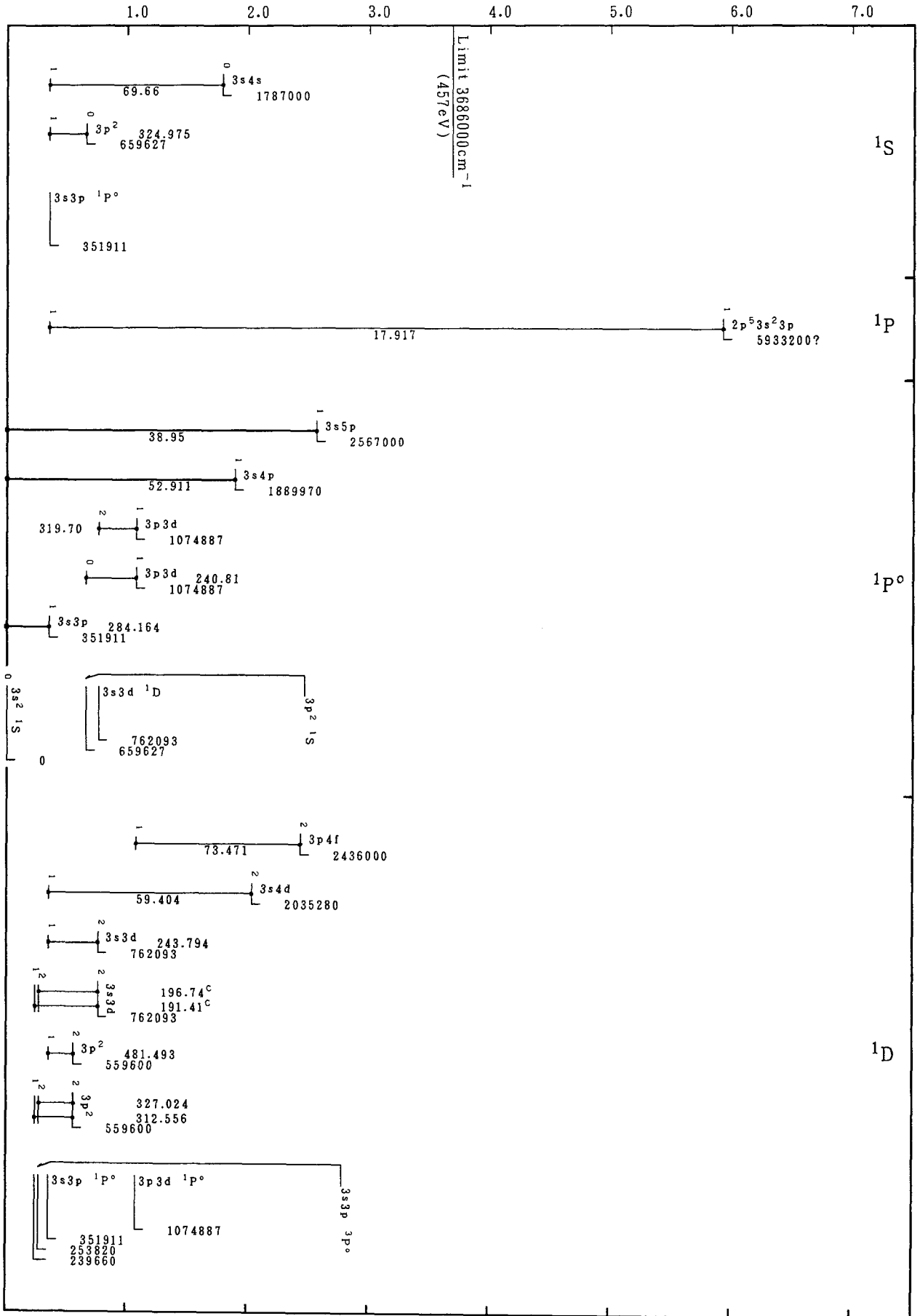
Grotrian Diagrams for Fe XV (Mg-Sequence)
