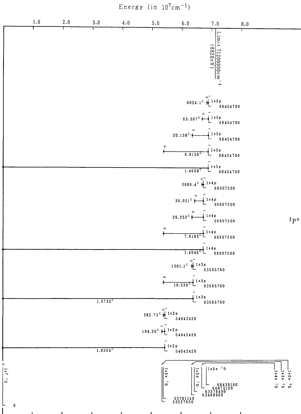
Grotrian Diagrams for Fe XXV (He-Sequence)-Continued
