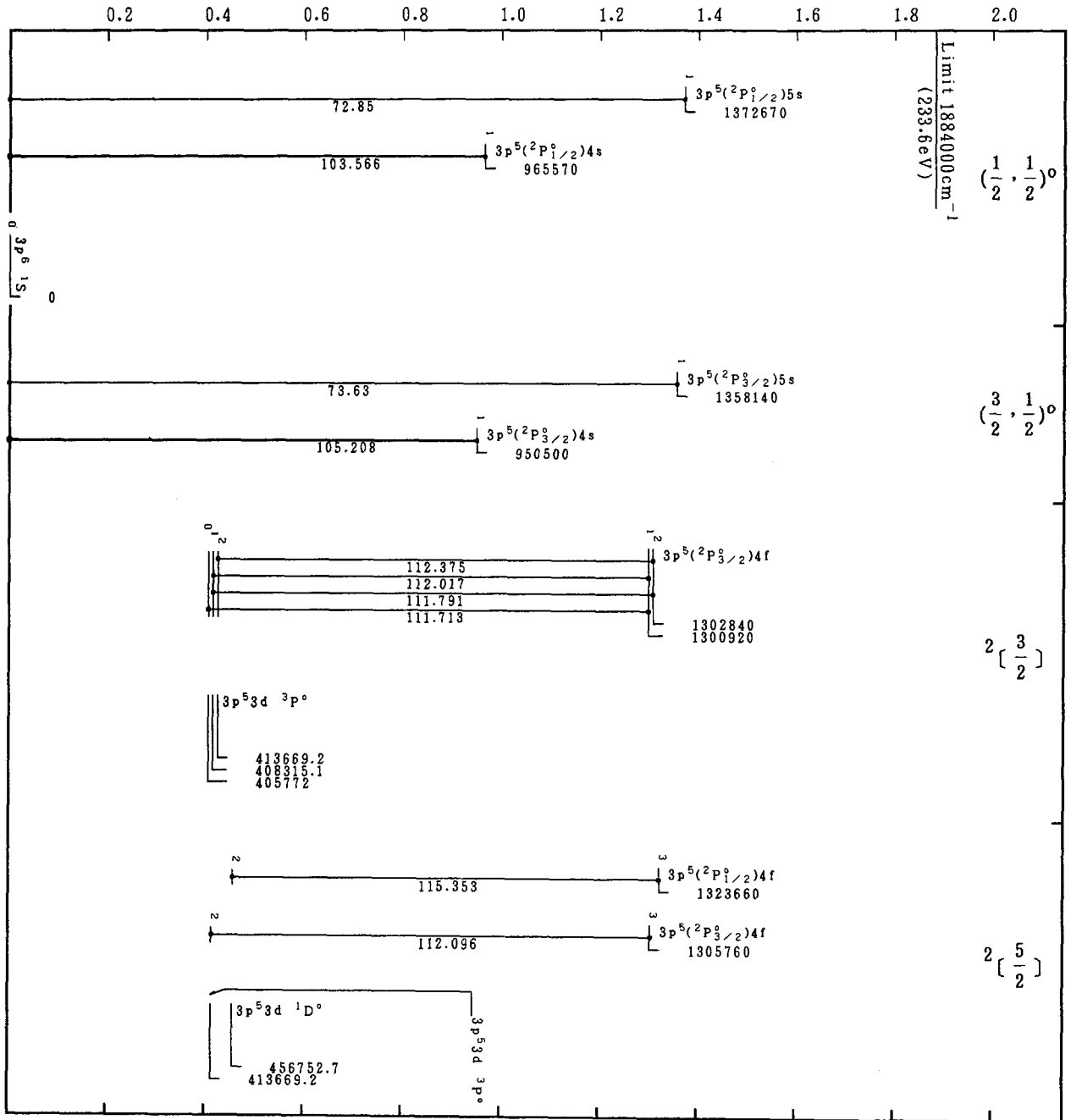
Grotrian Diagrams for Fe IX (Ar-Sequence)-Continued
