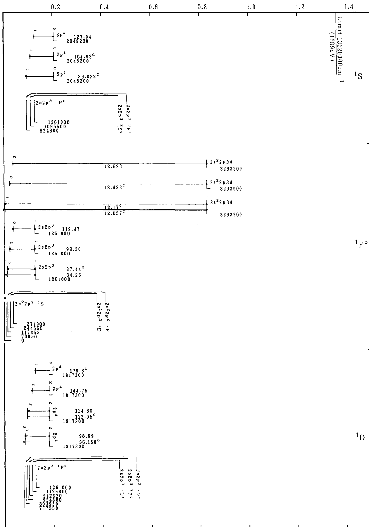
Grotrian Diagrams for Fe XXI (C-Sequence)
