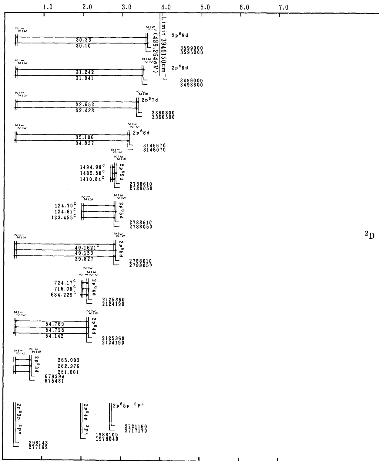
Grotrian Diagrams for Fe XVI (Na-Sequence)-Continued
