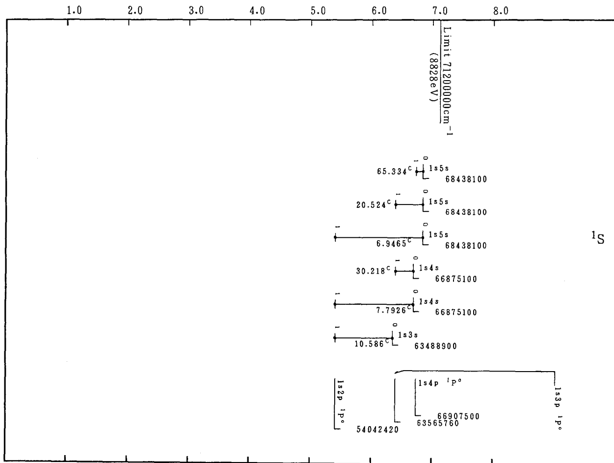
Grotrian Diagrams for Fe XXV (He-Sequence)
