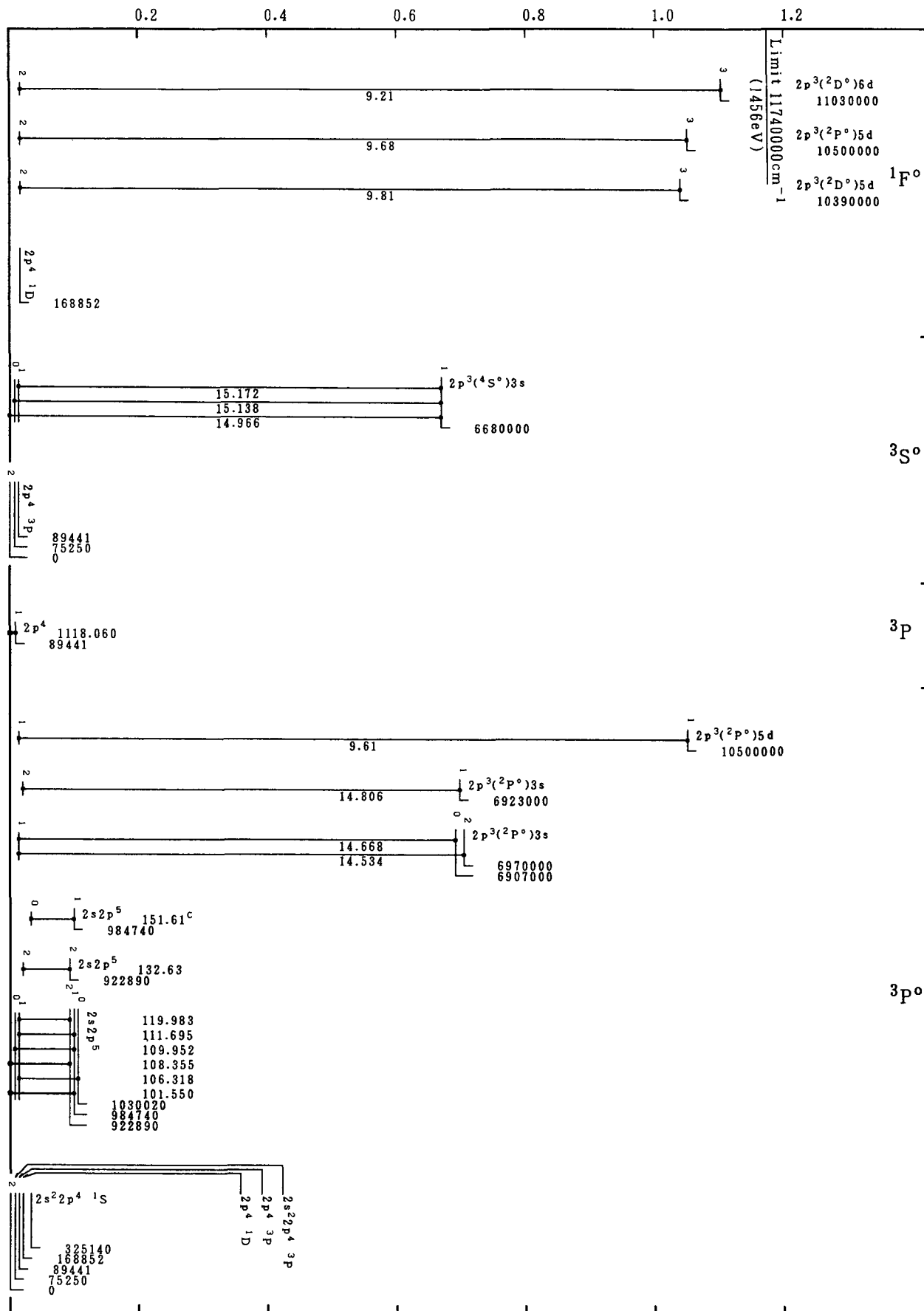
Grotrian Diagrams for Fe XIX (O-Sequence)-Continued
