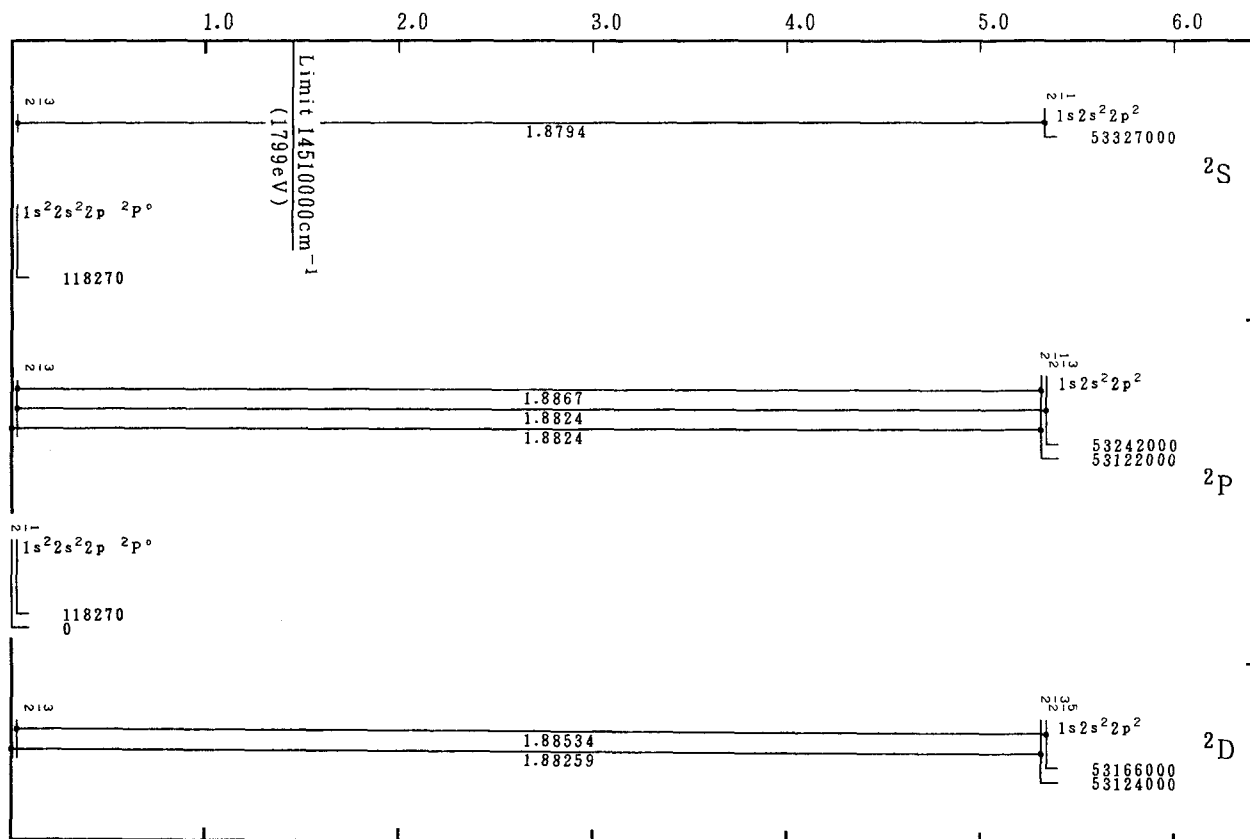
Grotrian Diagrams for Fe XXII (B-Sequence)-Continued
