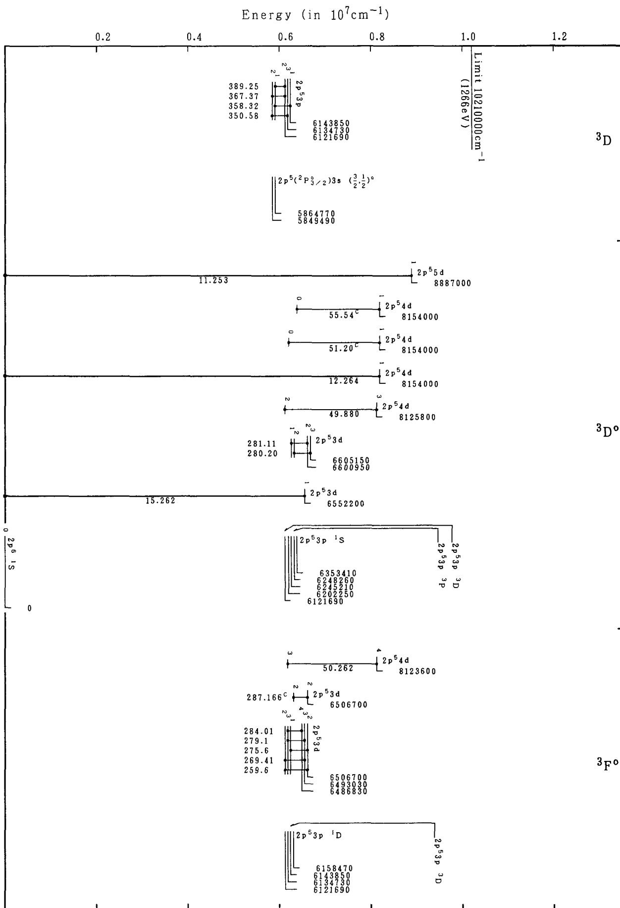
Grotrian Diagrams for Fe XVII (Ne-Sequence)-Continued
