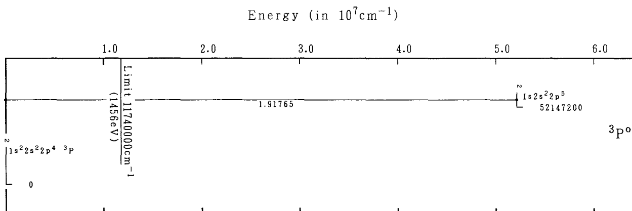
Grotrian Diagrams for Fe XIX (O-Sequence)-Continued
