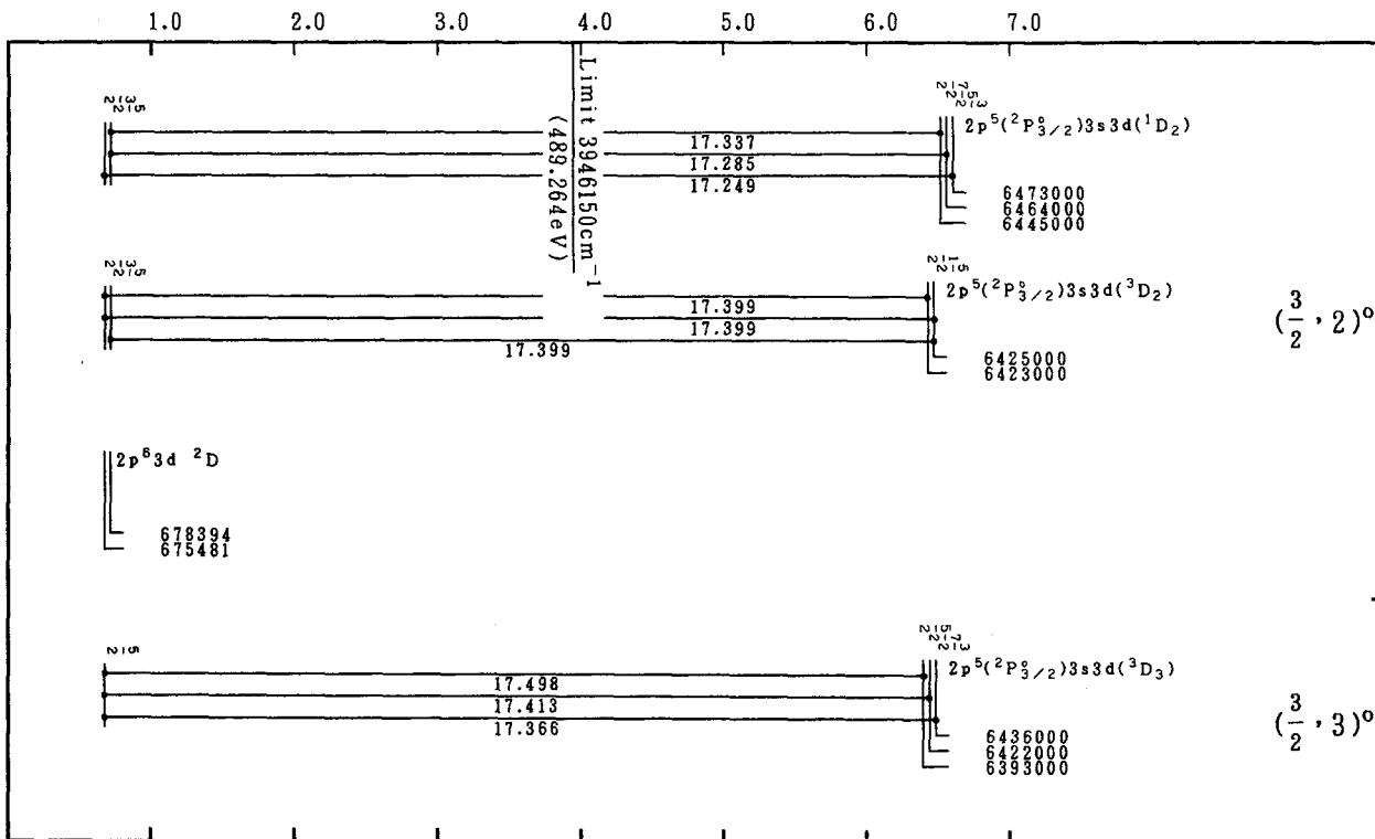
Grotrian Diagrams for Fe XVI (Na-Sequence)-Continued
