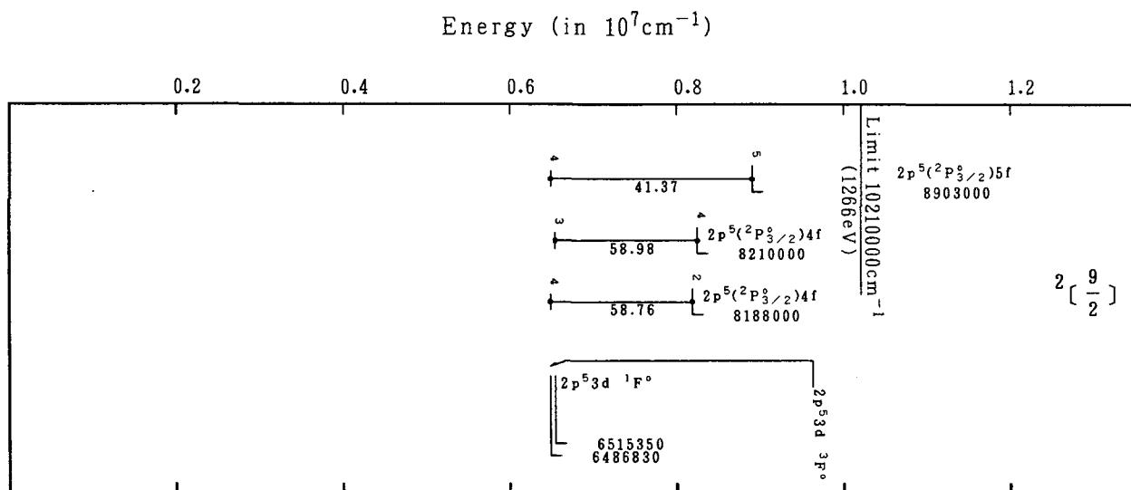
Grotrian Diagrams for Fe XVII (Ne-Sequence)-Continued
