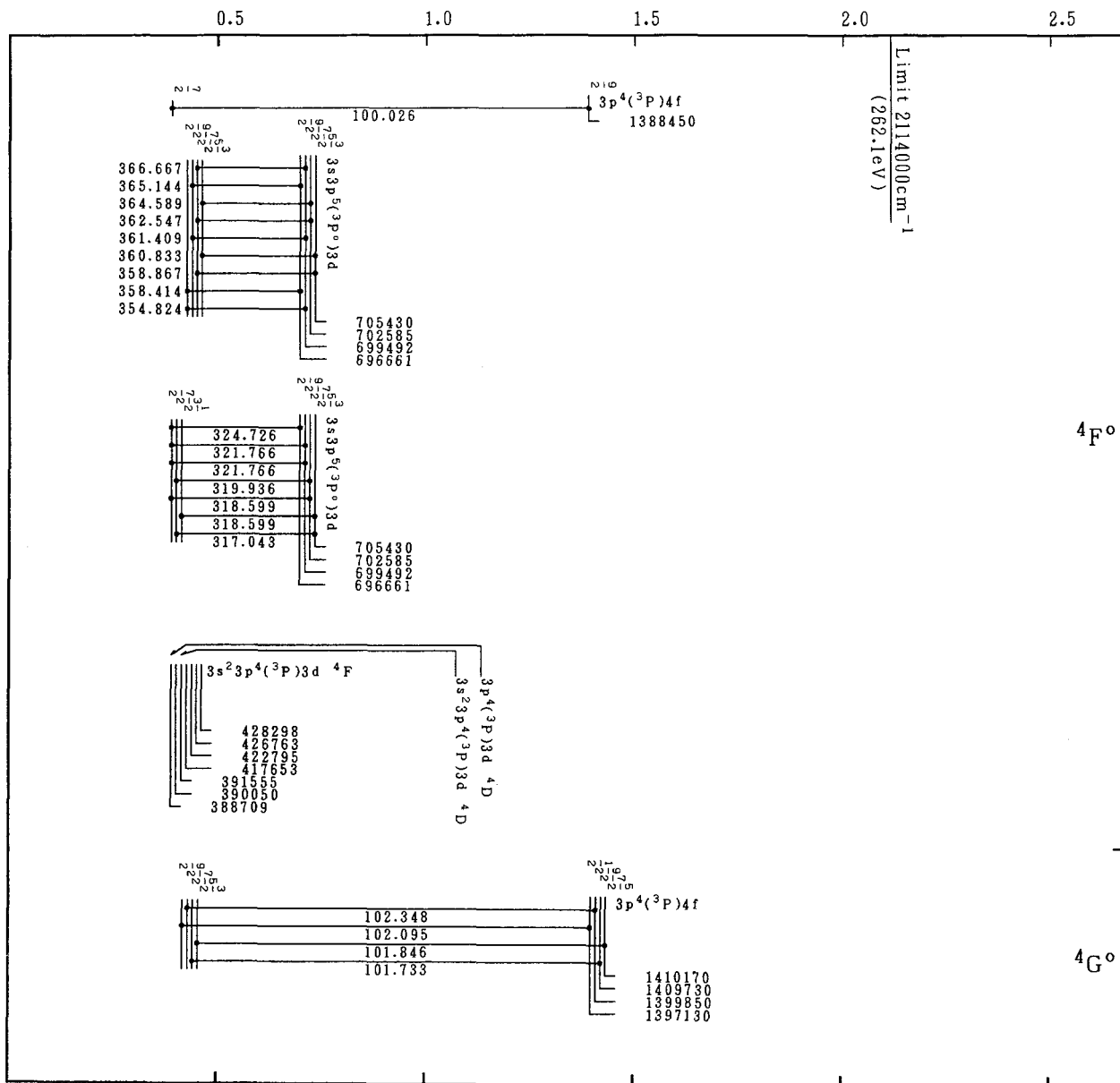
Grotrian Diagrams for Fe X (Cl-Sequence)-Continued
