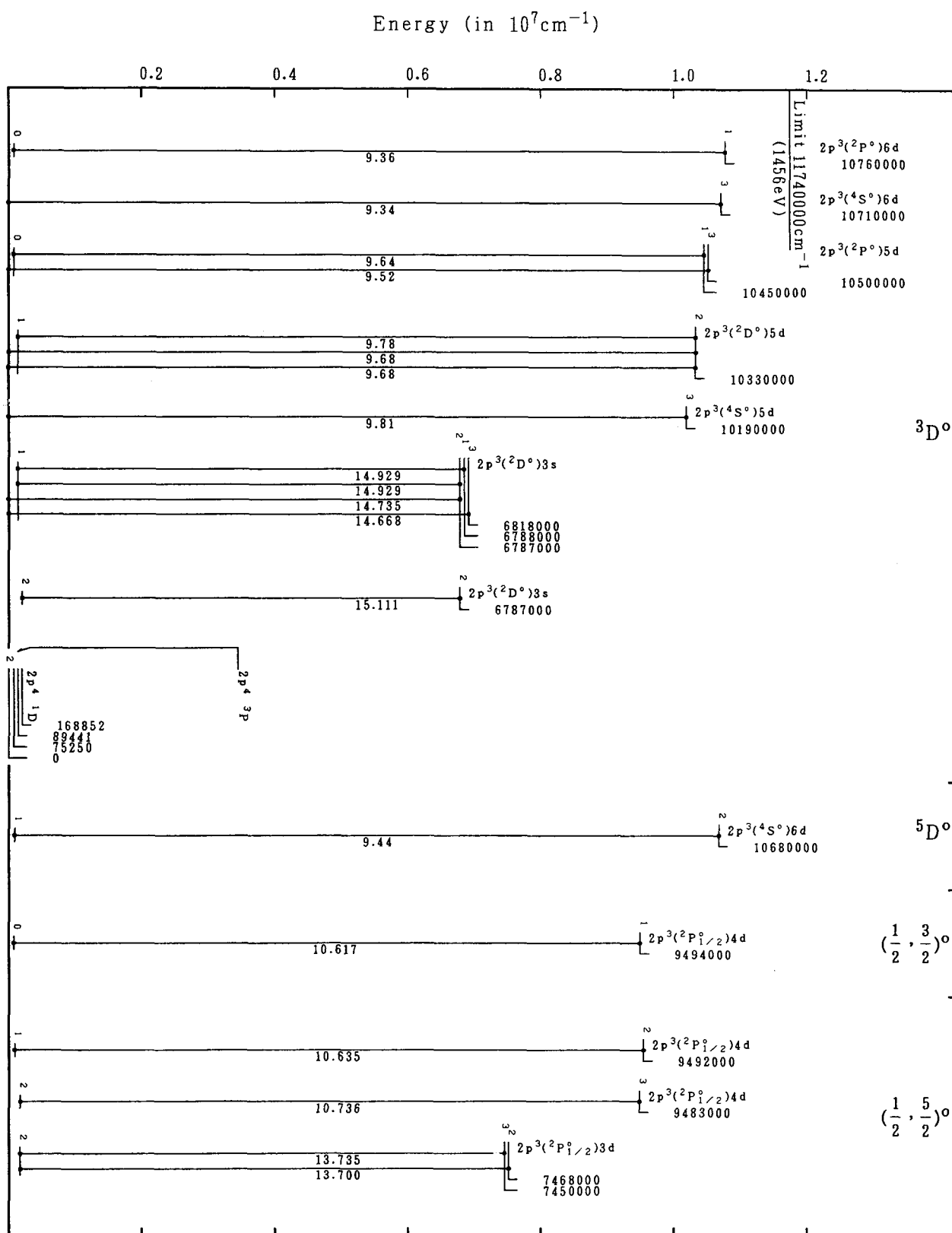
Grotrian Diagrams for Fe XIX (O-Sequence)-Continued
