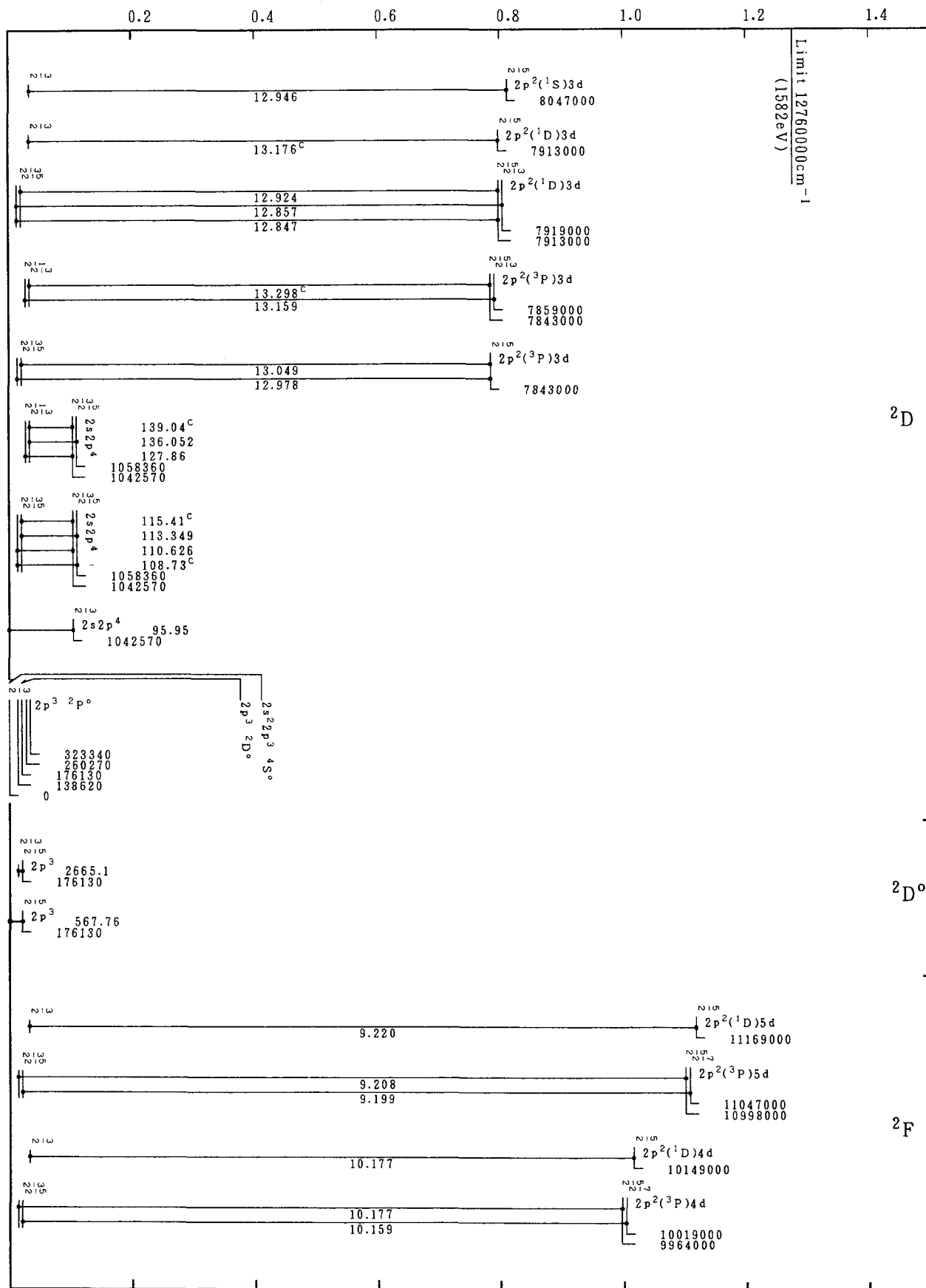
Grotrian Diagrams for Fe XX (N-Sequence)-Continued
