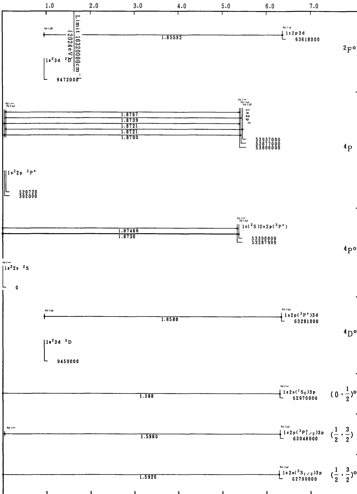
Grotrian Diagrams for Fe XXIV (Li-Sequence)
