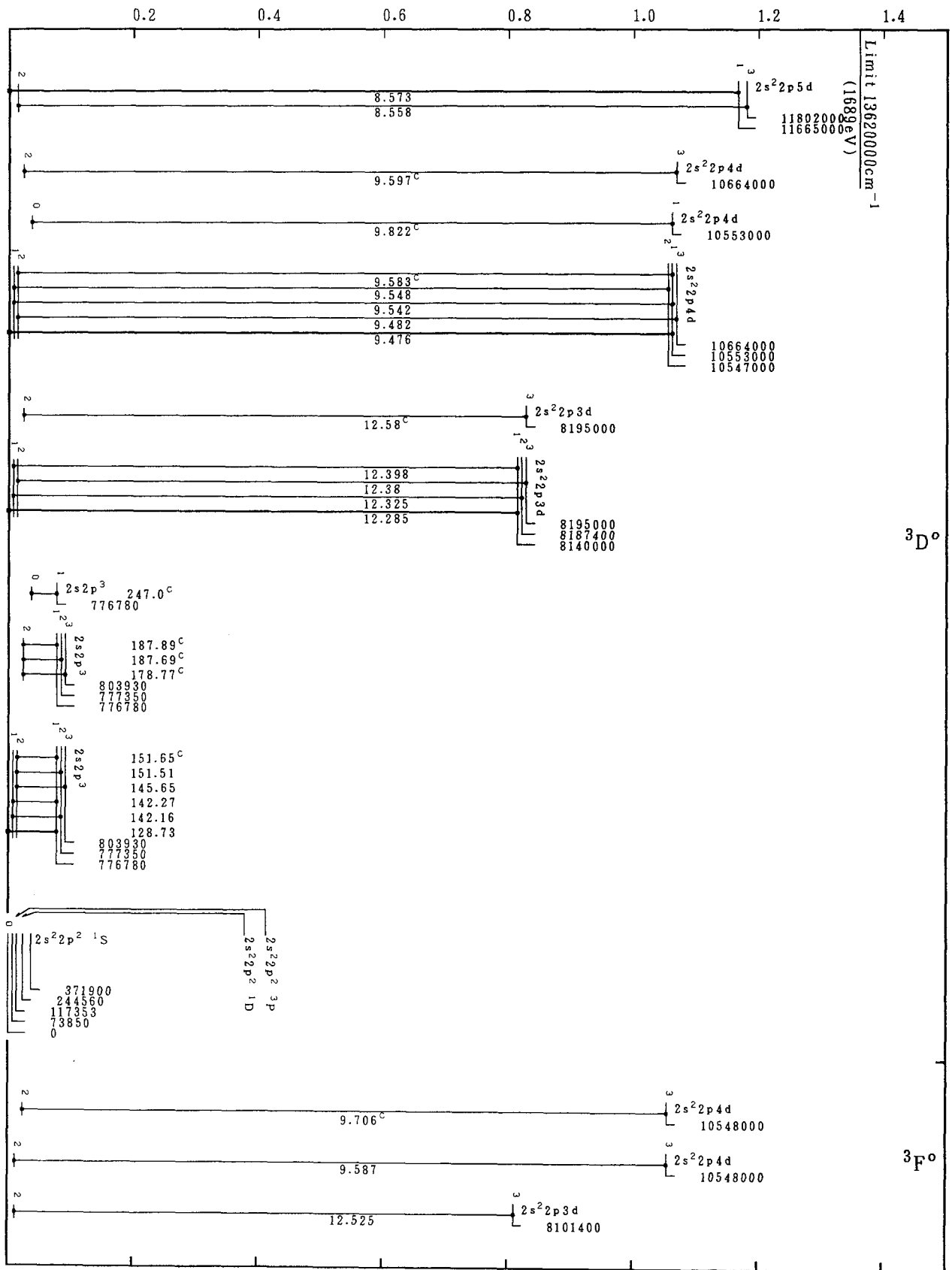
Grotrian Diagrams for Fe XXI (C-Sequence)-Continued
