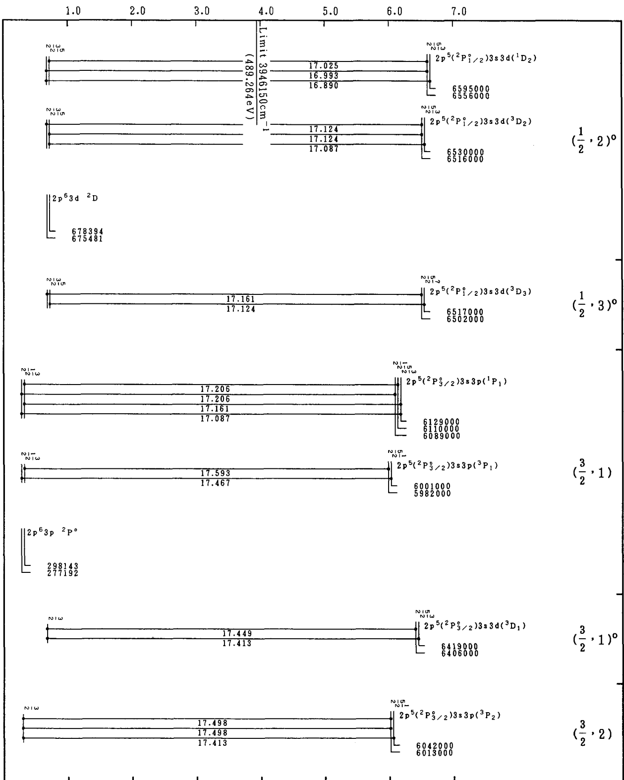
Grotrian Diagrams for Fe XVI (Na-Sequence)-Continued
