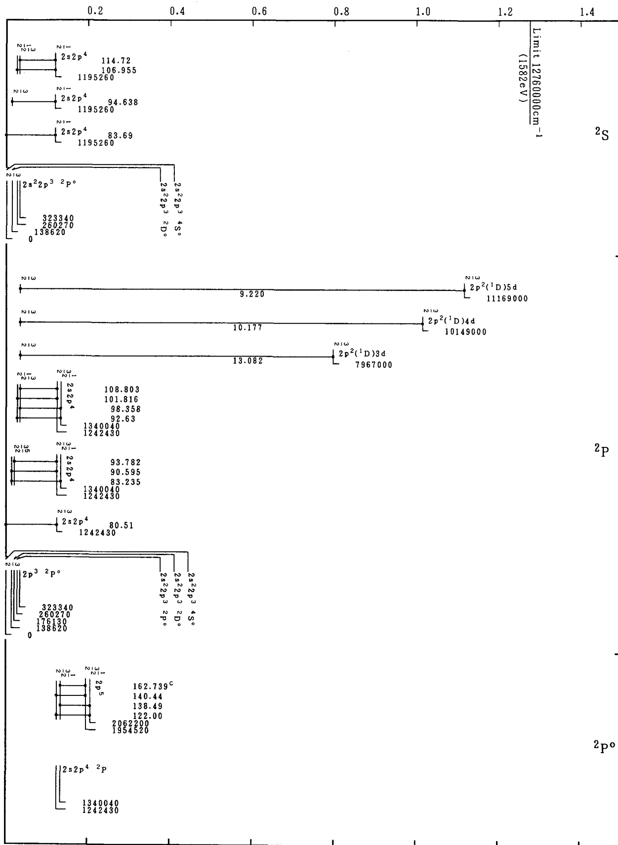
Grotrian Diagrams for Fe XX (N-Sequence)
