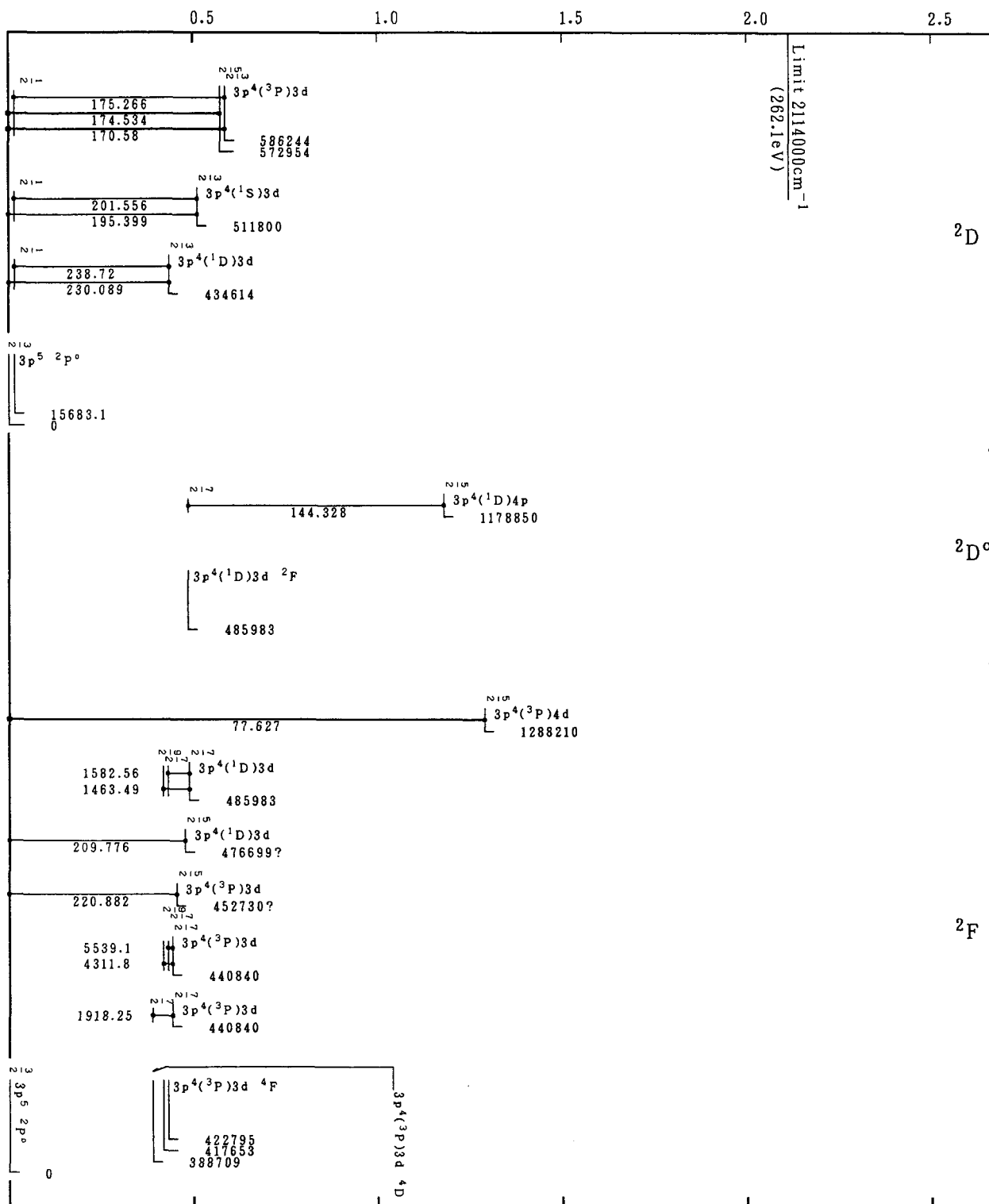
Grotrian Diagrams for Fe X (Cl-Sequence)-Continued
