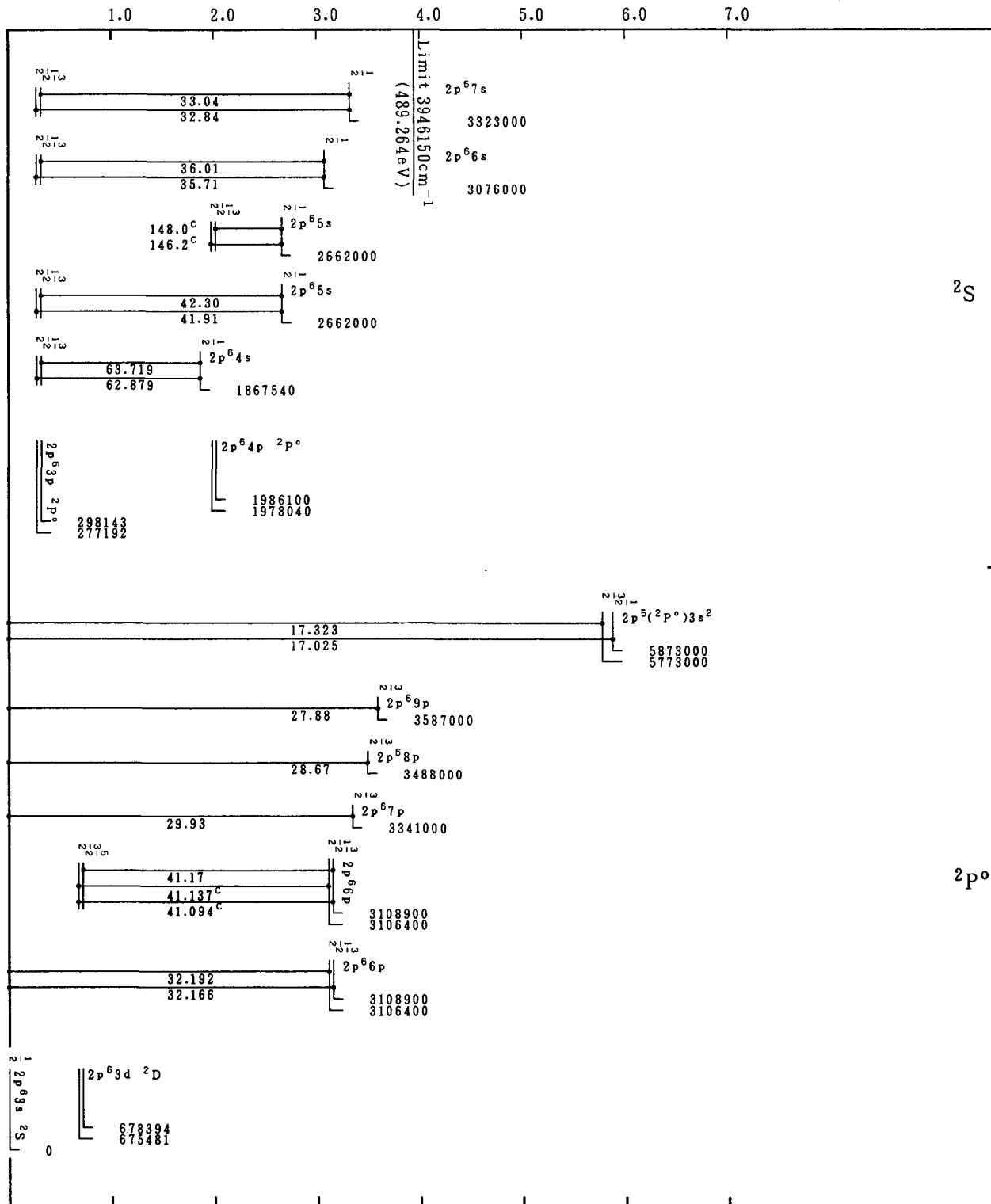
Grotrian Diagrams for Fe XVI (Na-Sequence)
