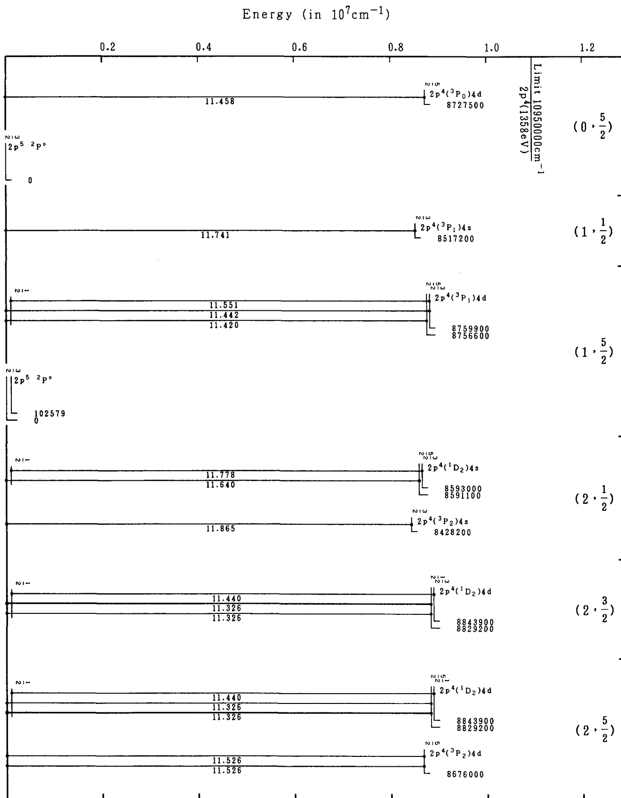
Grotrian Diagrams for Fe XVIII (F-Sequence)-Continued
