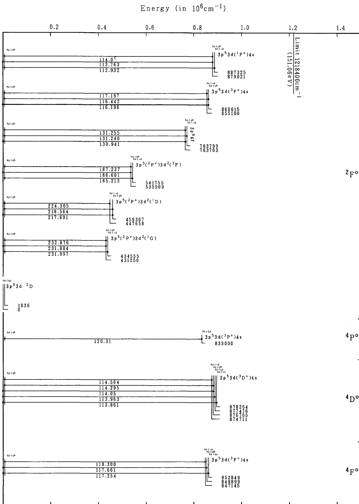
Grotrian Diagrams for Fe VIII (K-Sequence)-Continued
