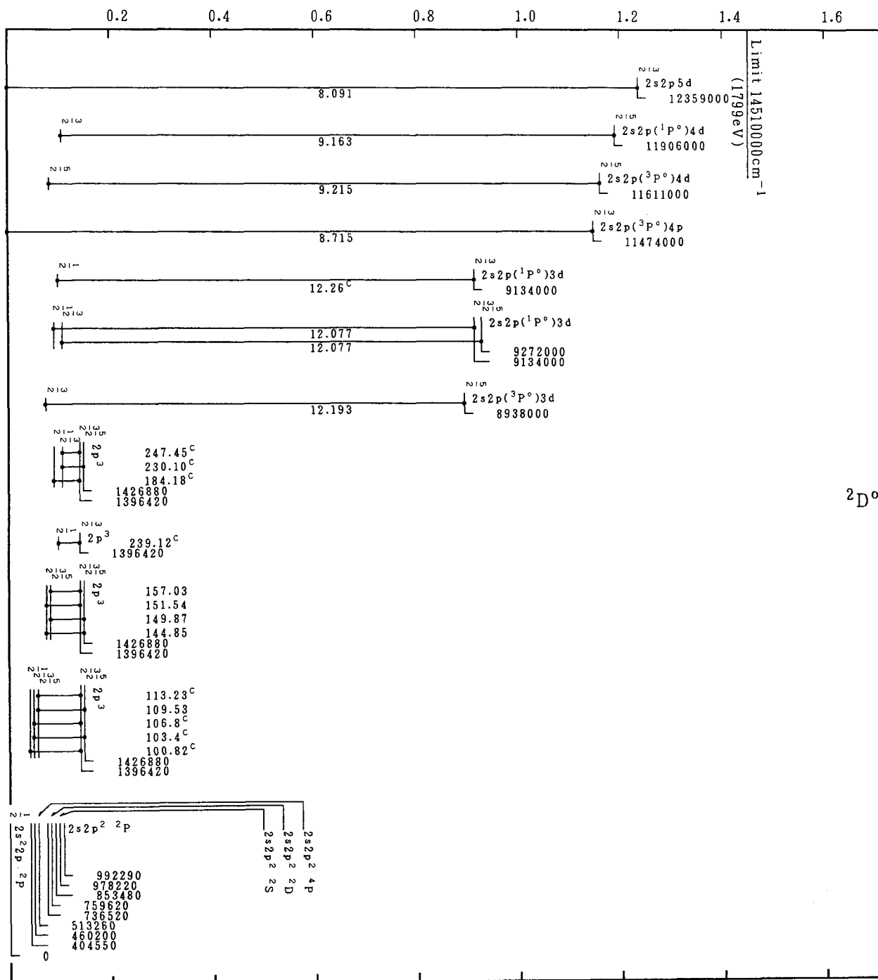
Grotrian Diagrams for Fe XXII (B-Sequence)-Continued
