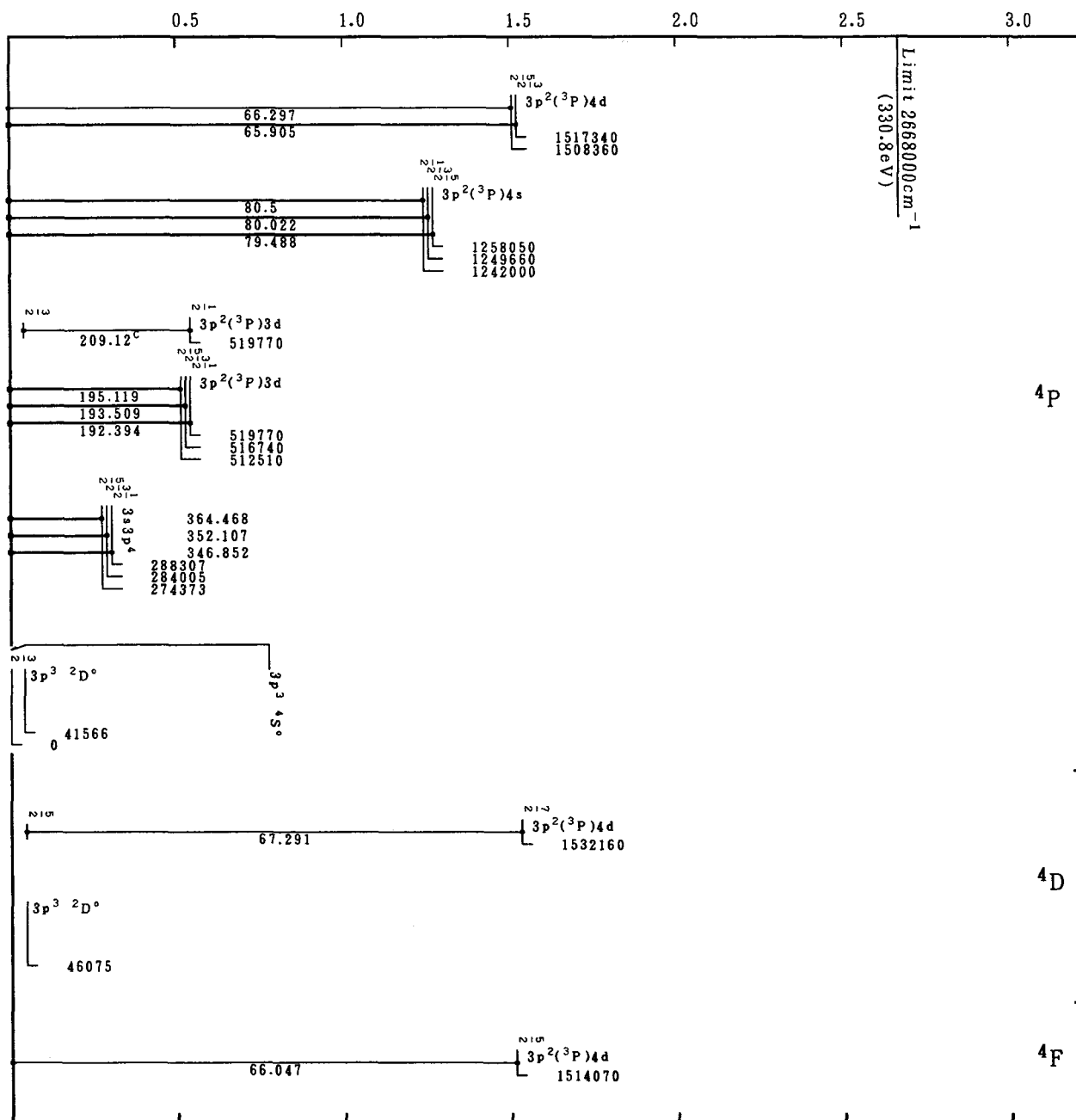
Grotrian Diagrams for Fe XII (P-Sequence)-Continued
