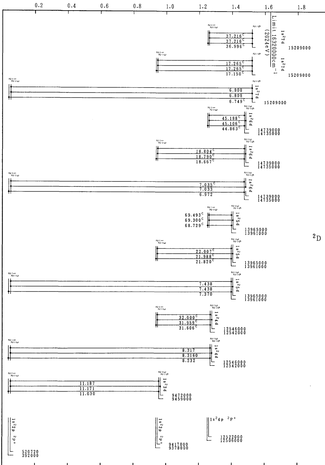
Grotrian Diagrams for Fe XXIV (Li-Sequence)-Continued
