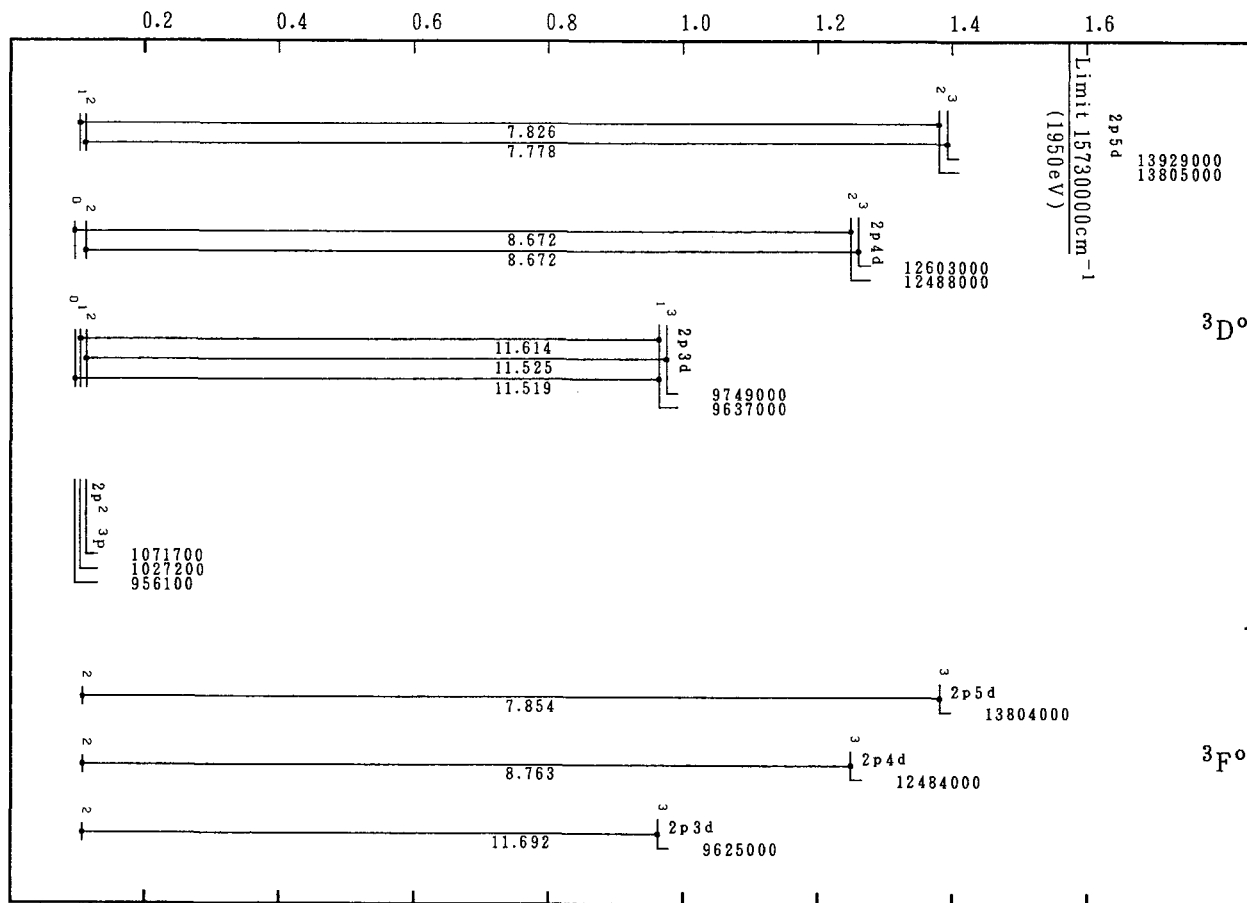
Grotrian Diagrams for Fe XXIII (Be-Sequence)-Continued
