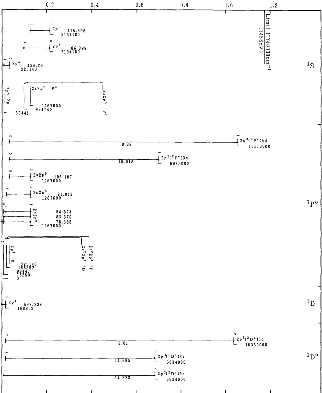
Grotrian Diagrams for Fe XIX (O-Sequence)
