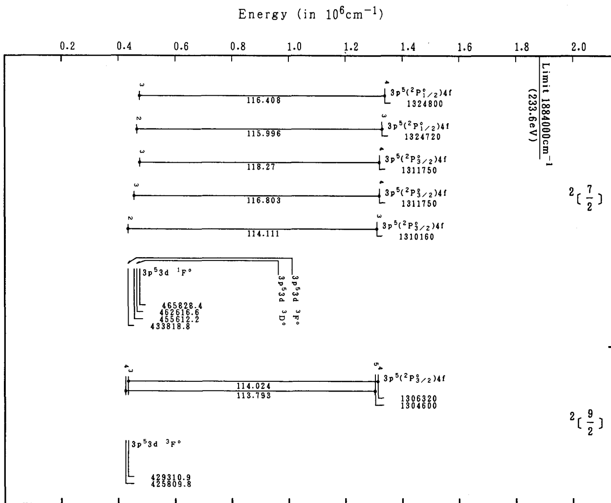
Grotrian Diagrams for Fe IX (Ar-Sequence)-Continued
