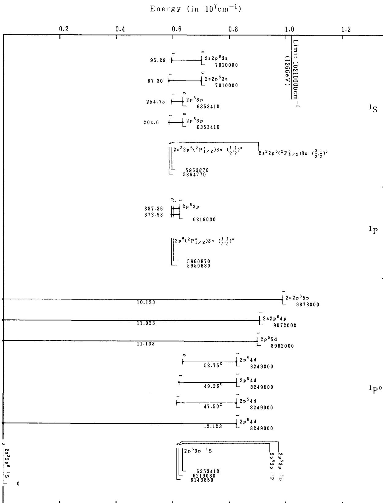
Grotrian Diagrams for Fe XVII (Ne-Sequence)
