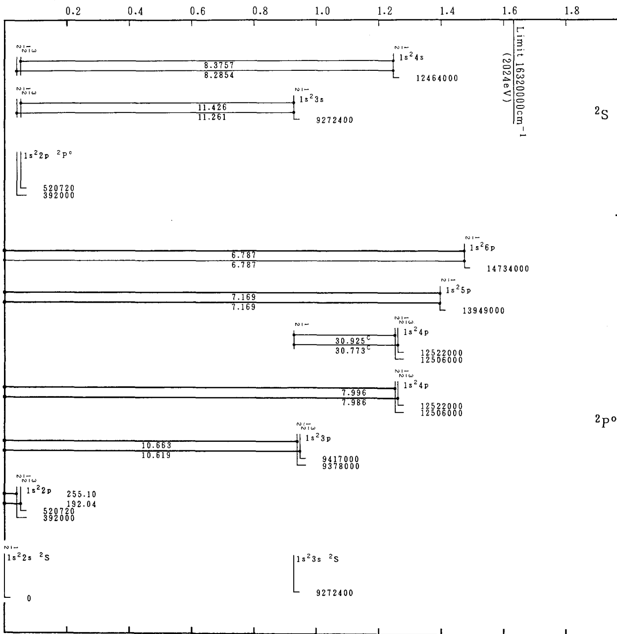
Grotrian Diagrams for Fe XXIV (Li-Sequence)
