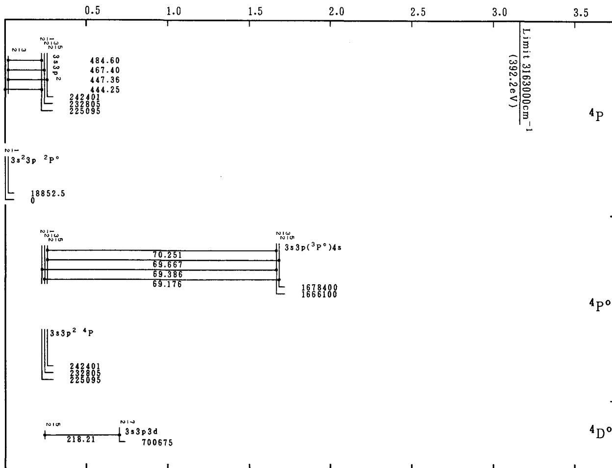
Grotrian Diagrams for Fe XIV (Al-Sequence)-Continued
