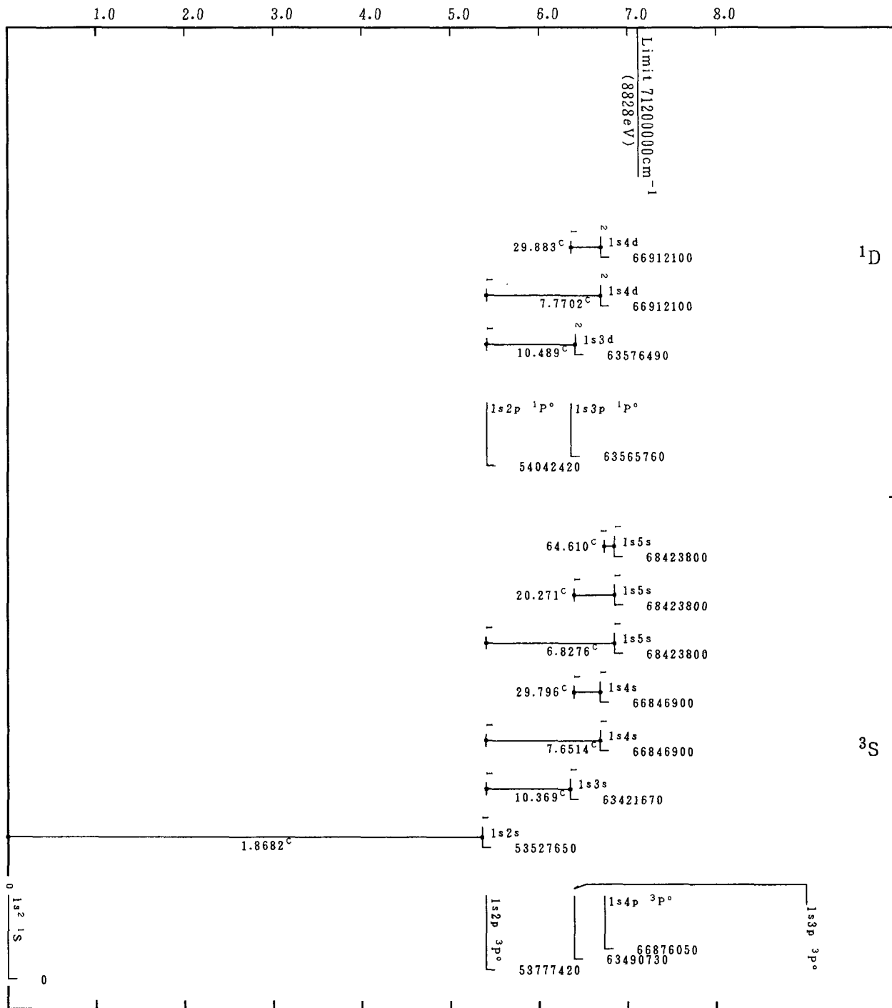
Grotrian Diagrams for Fe XXV (He-Sequence)-Continued
