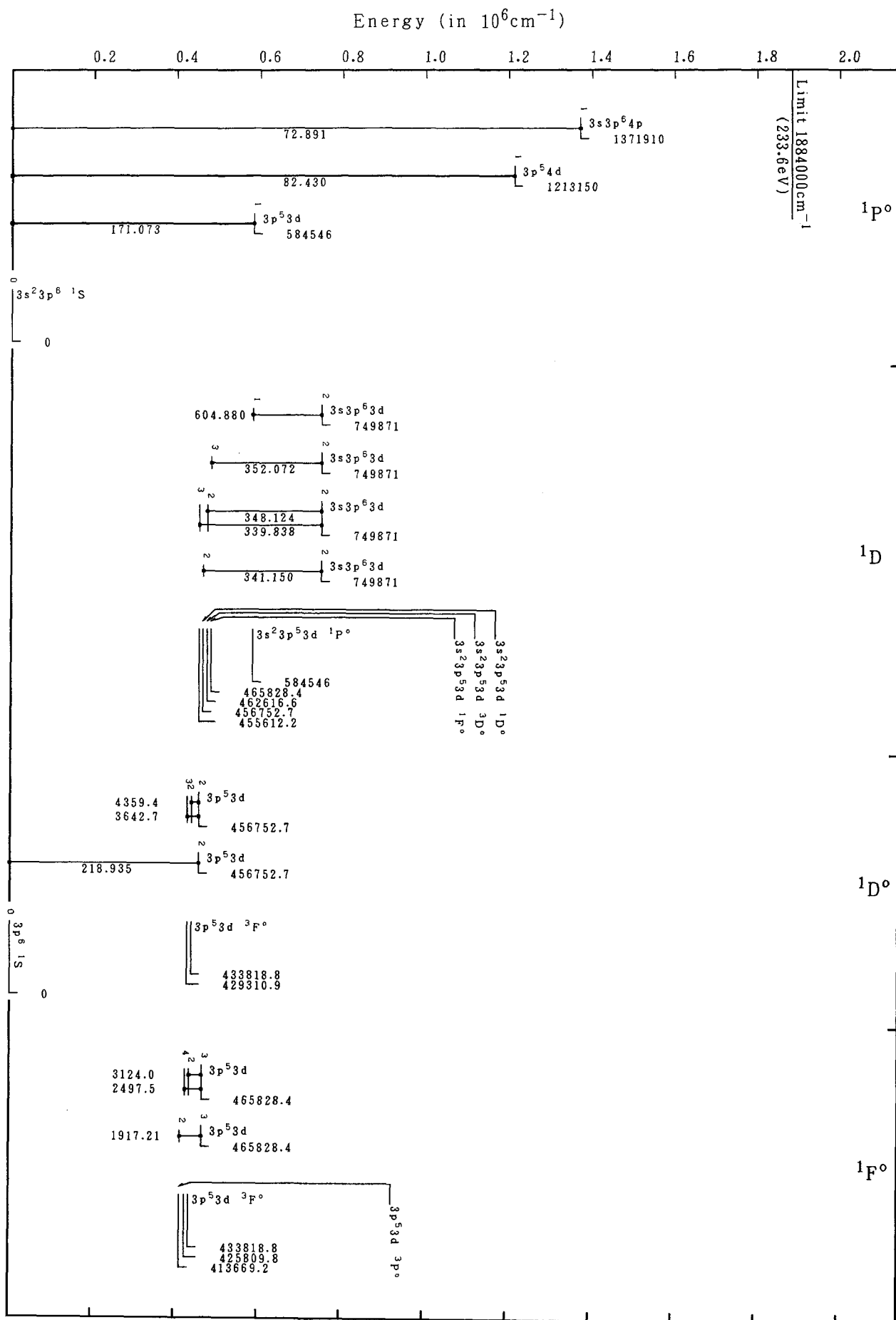
Grotrian Diagrams for Fe IX (Ar-Sequence)
