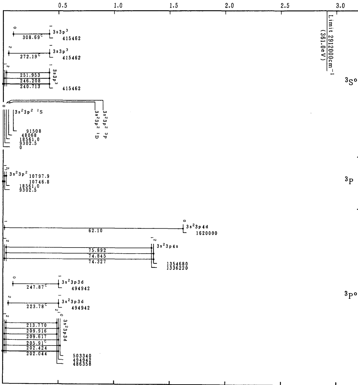
Grotrian Diagrams for Fe XIII (Si-Sequence)-Continued
