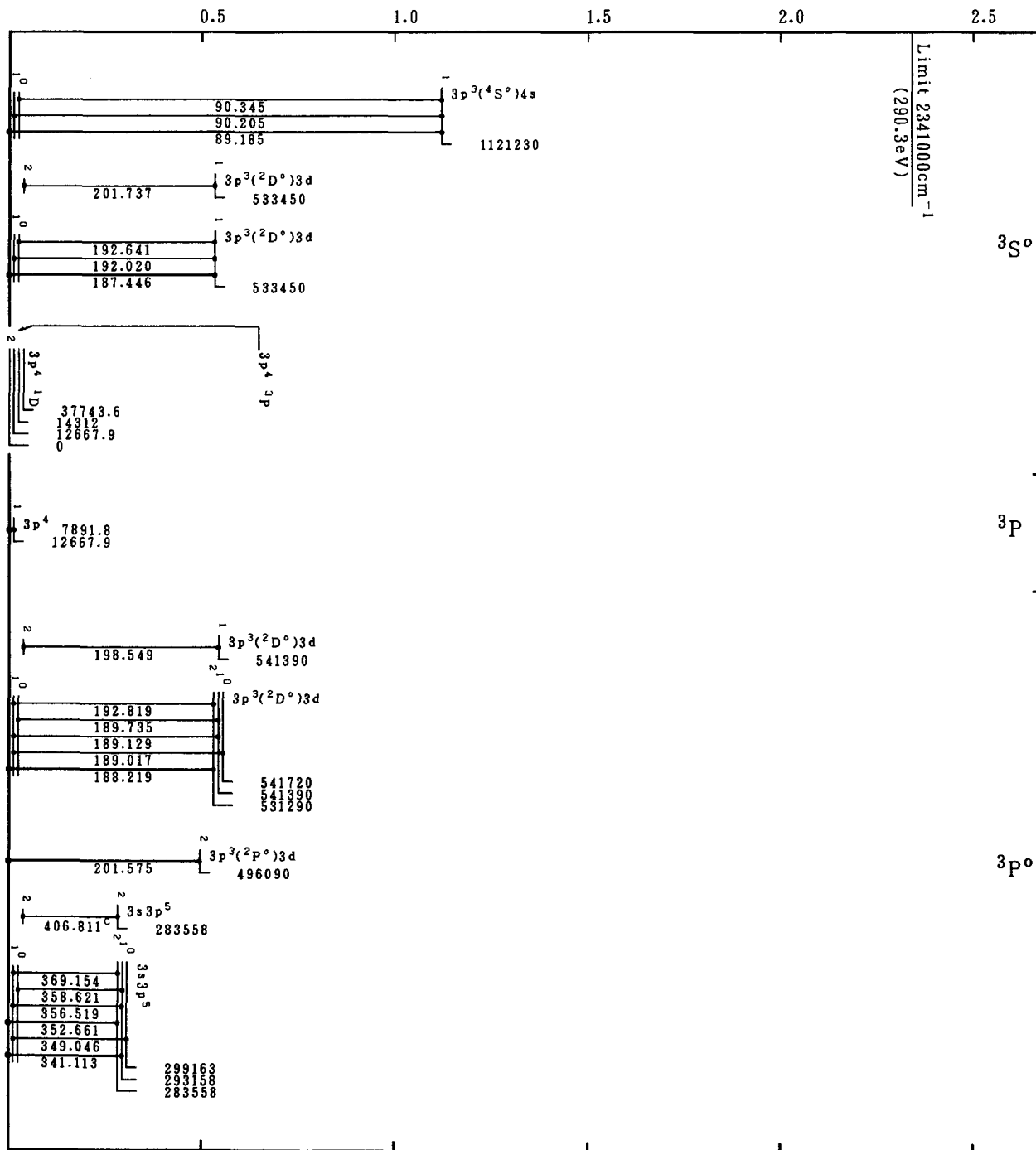
Grotrian Diagrams for Fe XI (S-Sequence)-Continued
