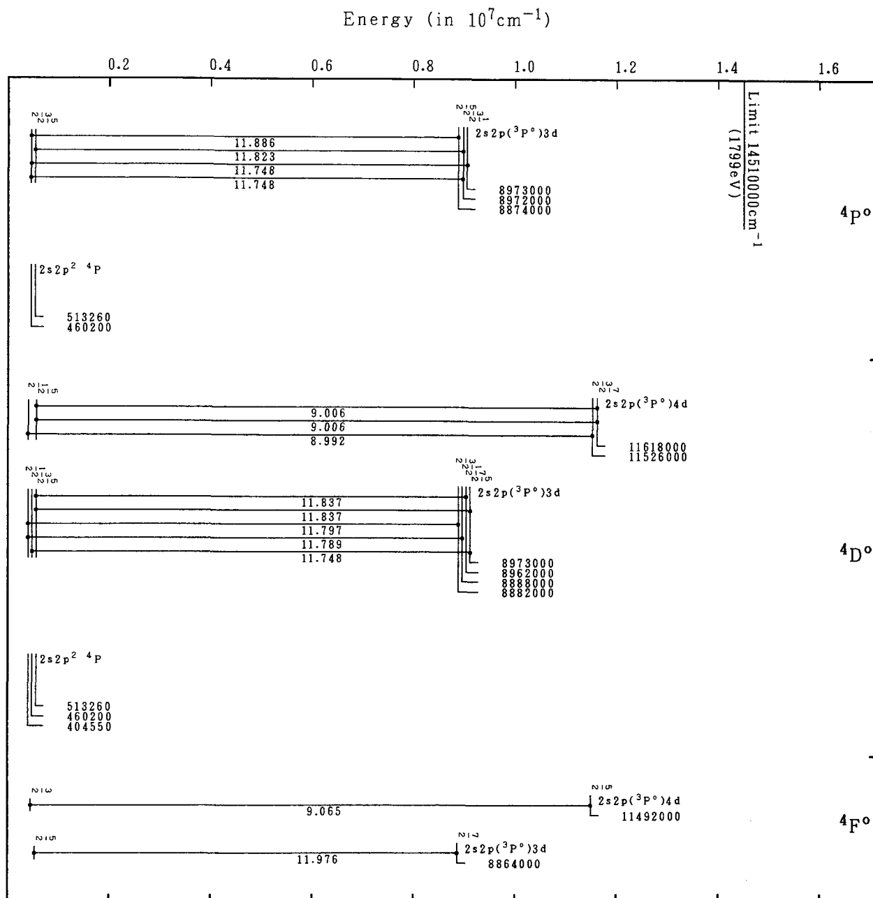
Grotrian Diagrams for Fe XXII (B-Sequence)-Continued
