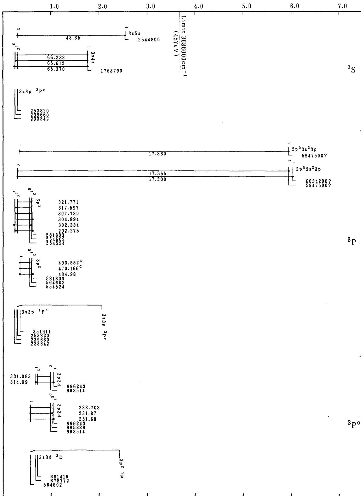
Grotrian Diagrams for Fe XV (Mg-Sequence)-Continued
