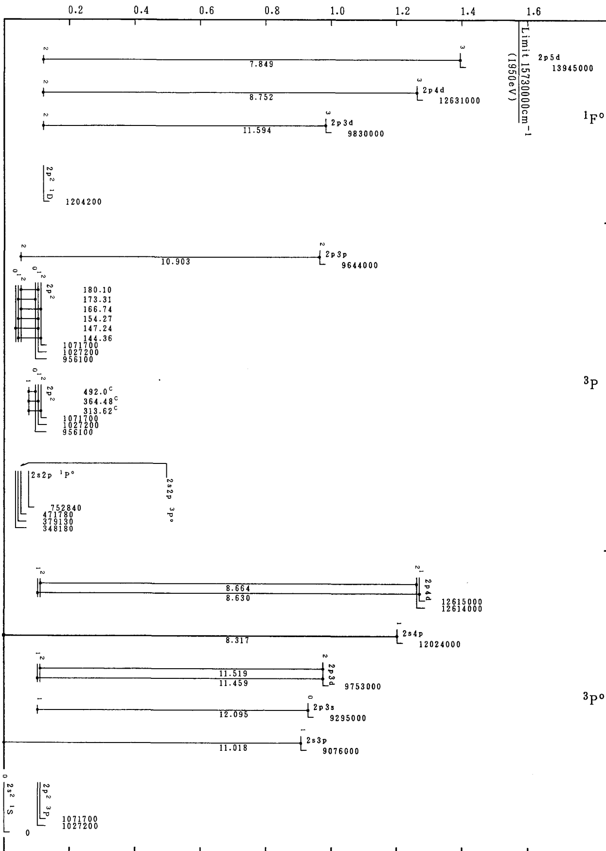
Grotrian Diagrams for Fe XXIII (Be-Sequence)-Continued
