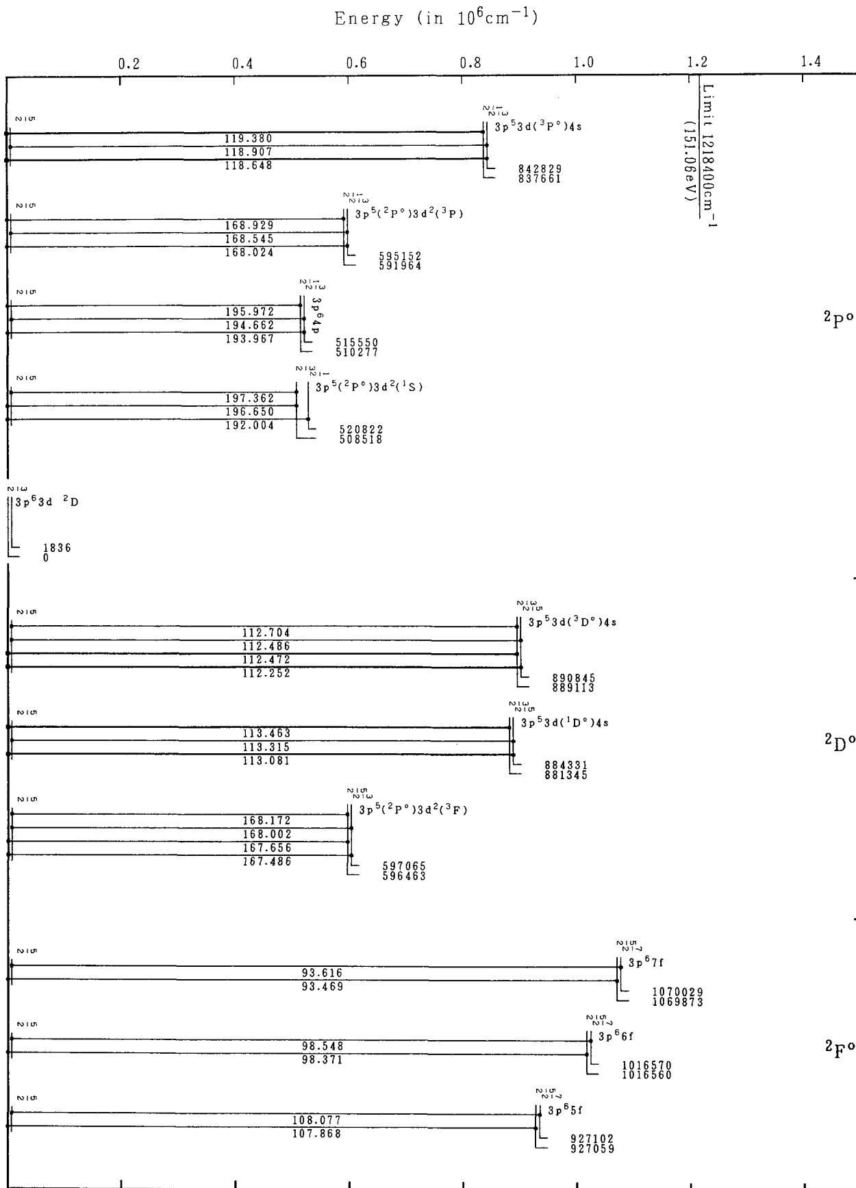
Grotrian Diagrams for Fe VIII (K-Sequence)
