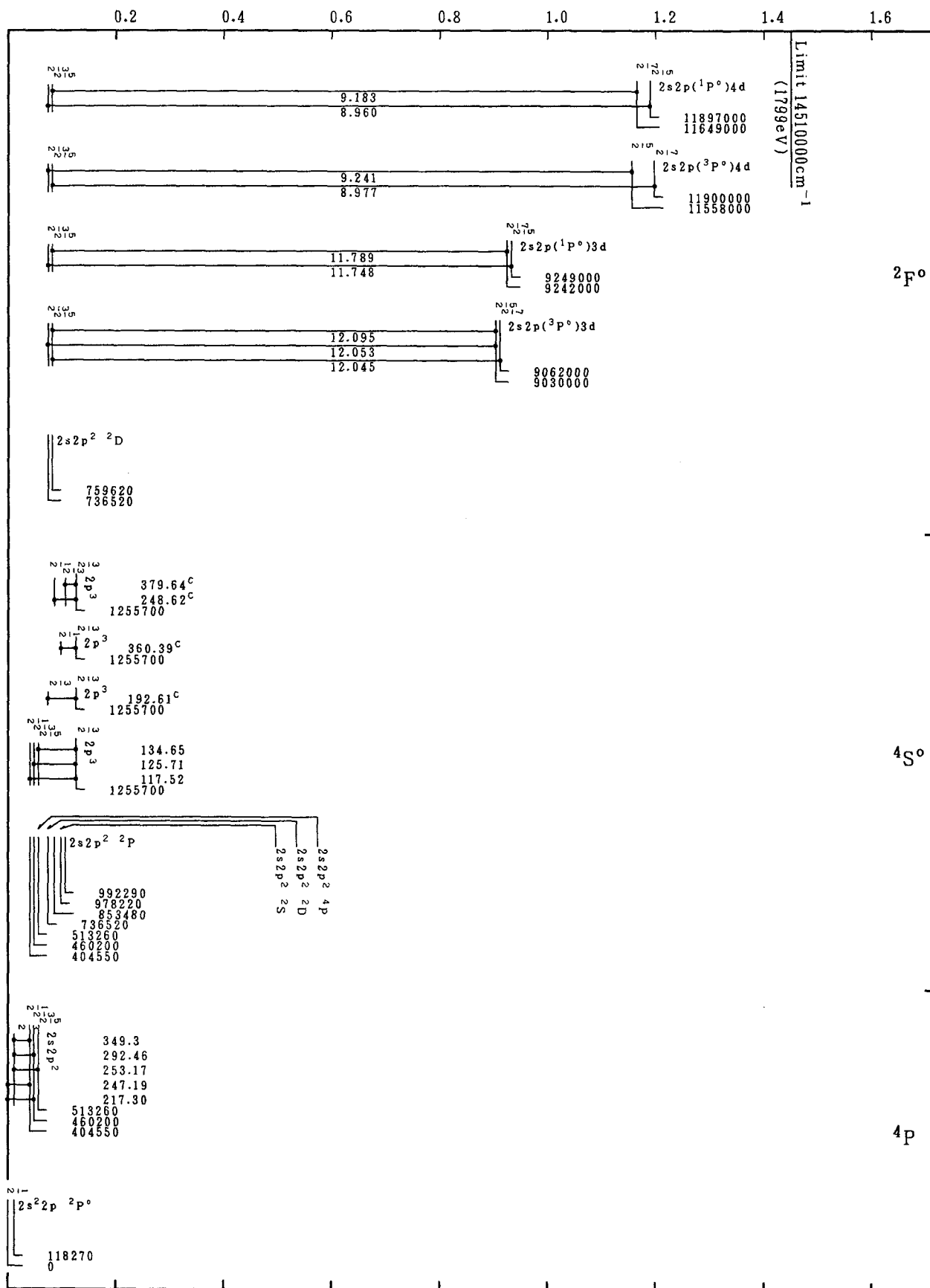
Grotrian Diagrams for Fe XXII (B-Sequence)-Continued
