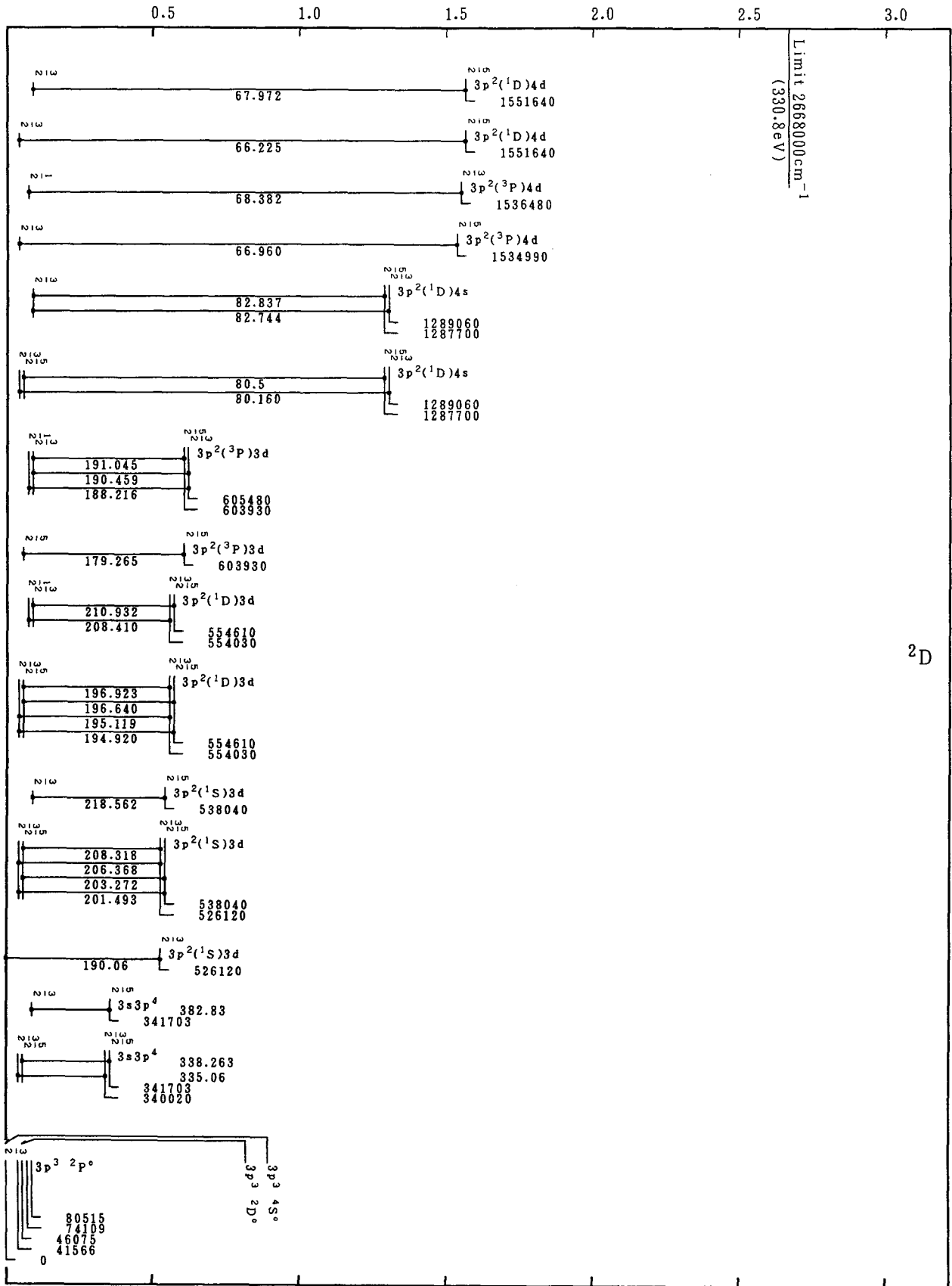
Grotrian Diagrams for Fe XII (P-Sequence)-Continued
