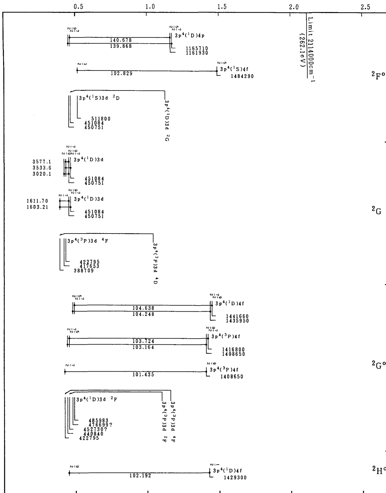
Grotrian Diagrams for Fe X (Cl-Sequence)-Continued
