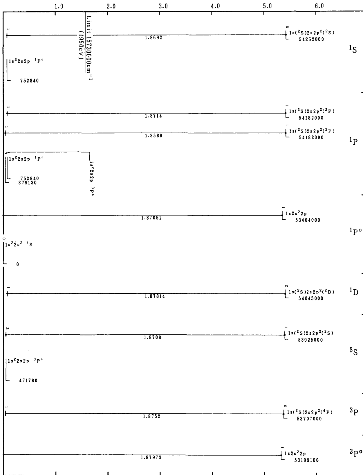
Grotrian Diagrams for Fe XXIII (Be-Sequence)-Continued
