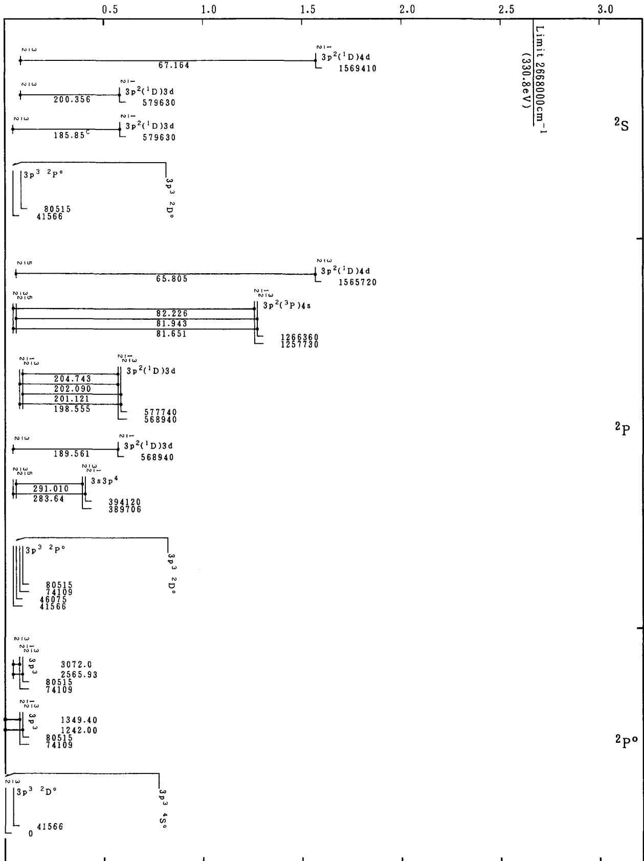
Grotrian Diagrams for Fe XII (P-Sequence)
