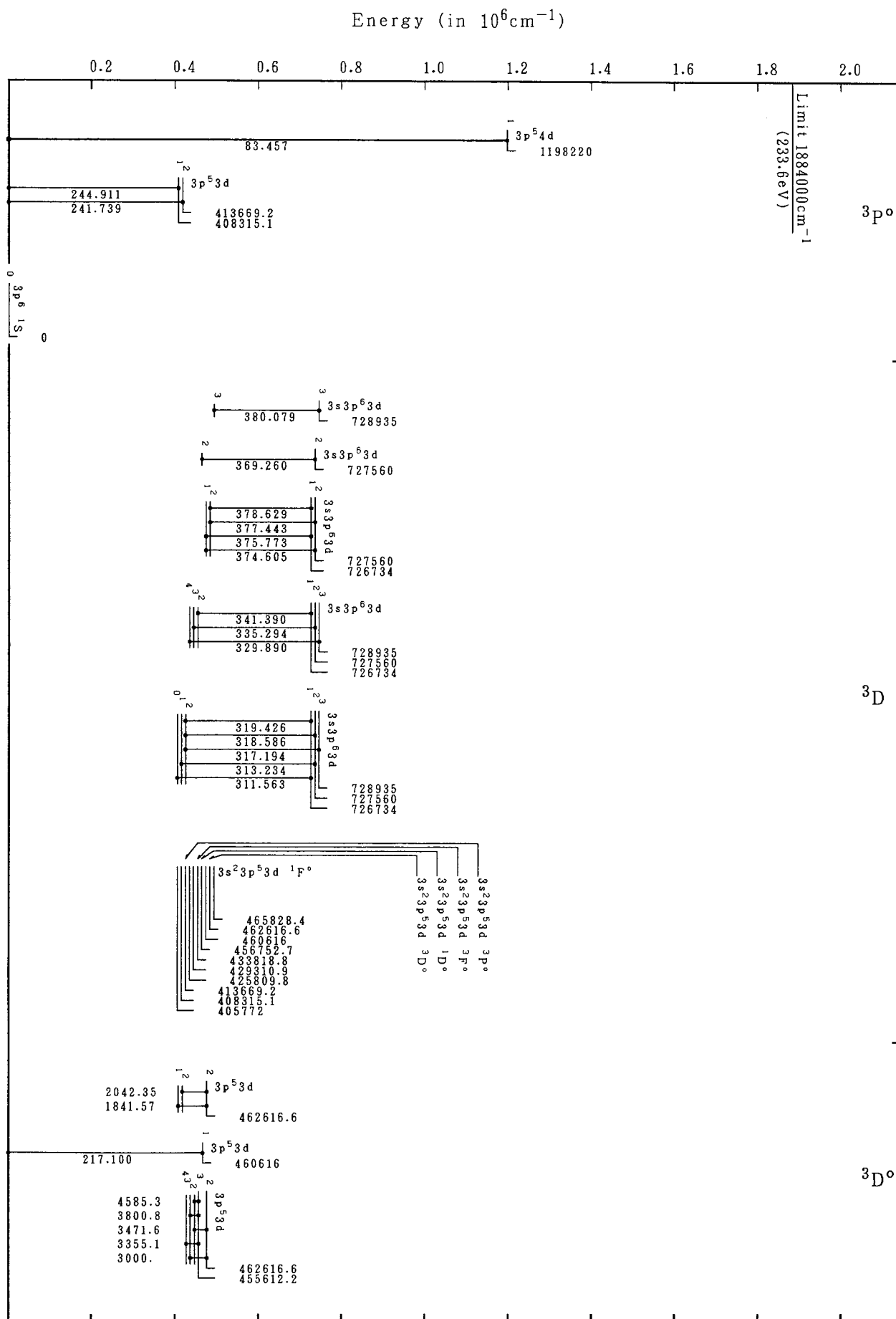
Grotrian Diagrams for Fe IX (Ar-Sequence)-Continued
