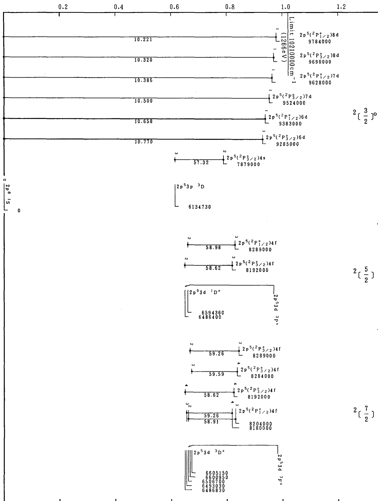
Grotrian Diagrams for Fe XVII (Ne-Sequence)-Continued
