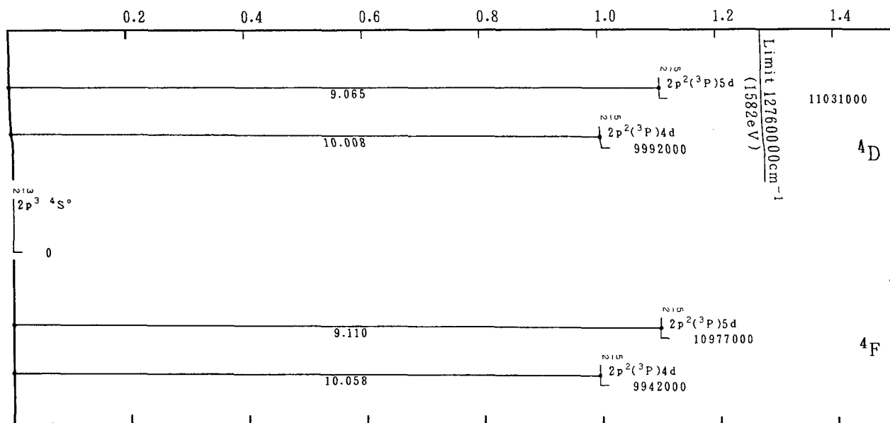
Grotrian Diagrams for Fe XX (N-Sequence)-Continued
