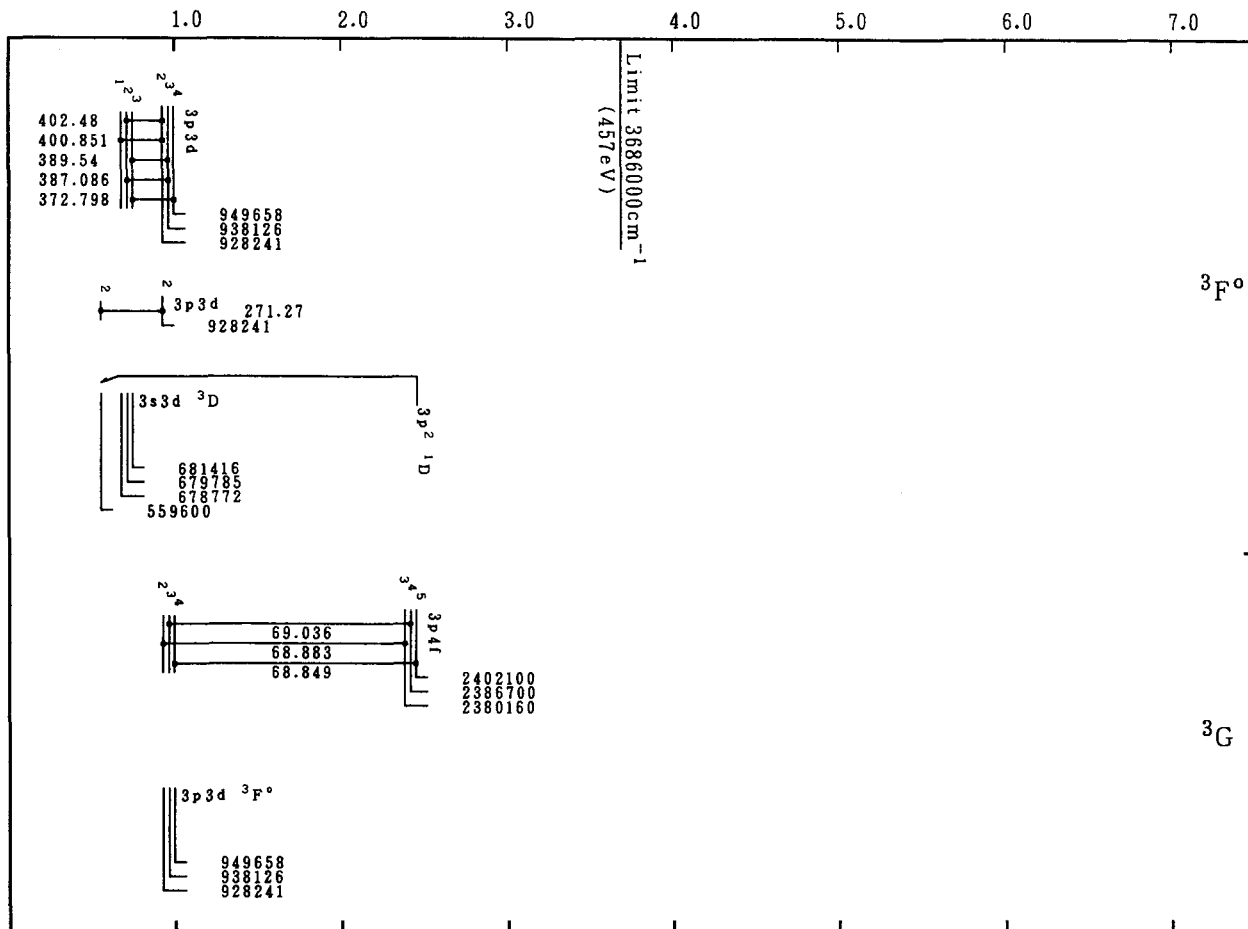
Grotrian Diagrams for Fe XV (Mg-Sequence)-Continued
