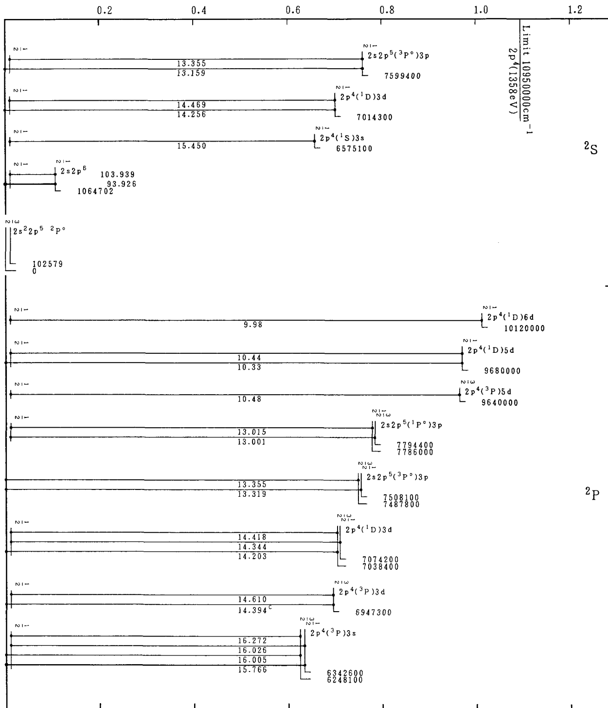
Grotrian Diagrams for Fe XVIII (F-Sequence)
