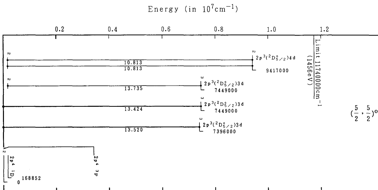
Grotrian Diagrams for Fe XIX (O-Sequence)-Continued
