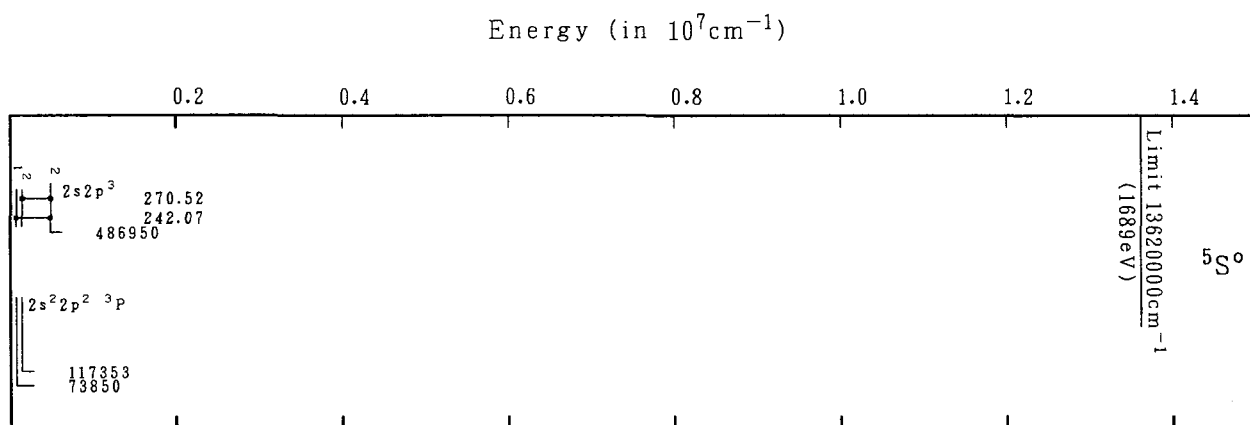
Grotrian Diagrams for Fe XXI (C-Sequence)-Continued
