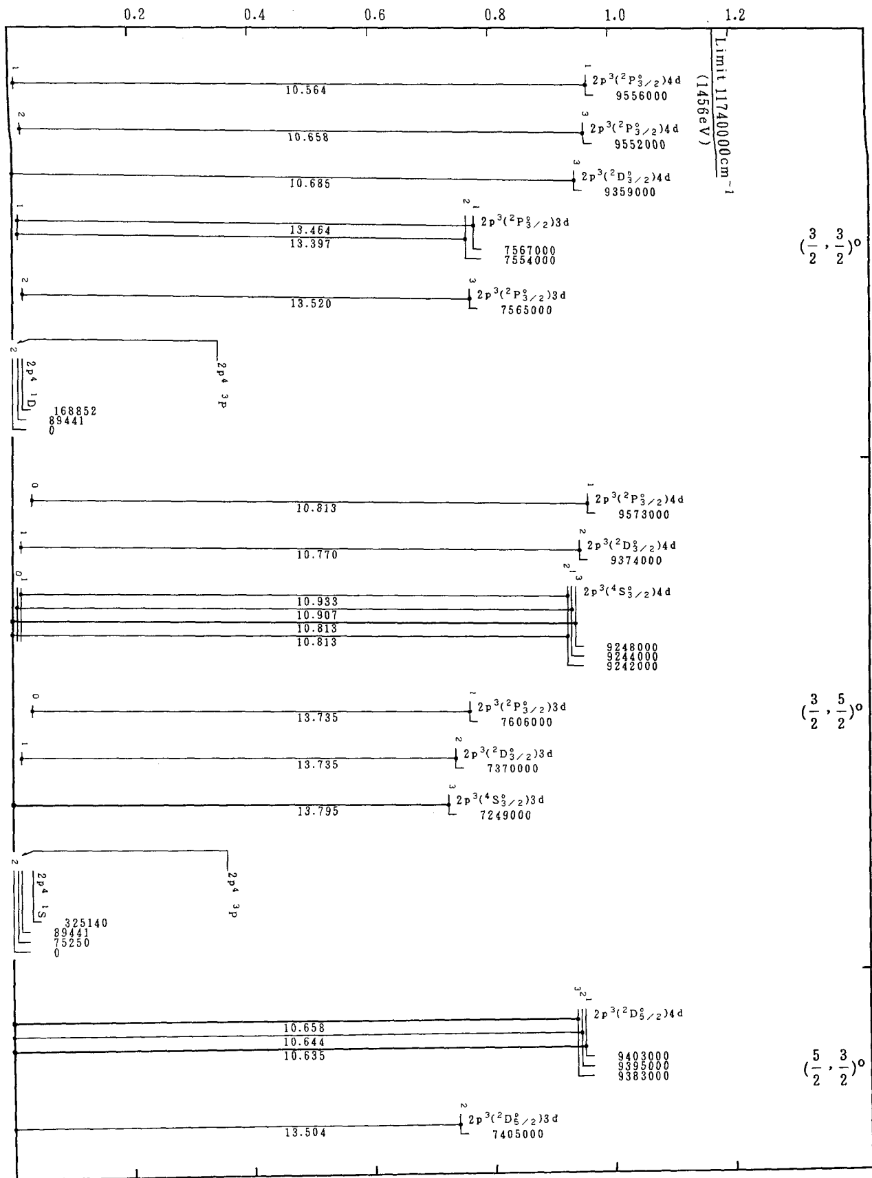
Grotrian Diagrams for Fe XIX (O-Sequence)-Continued
