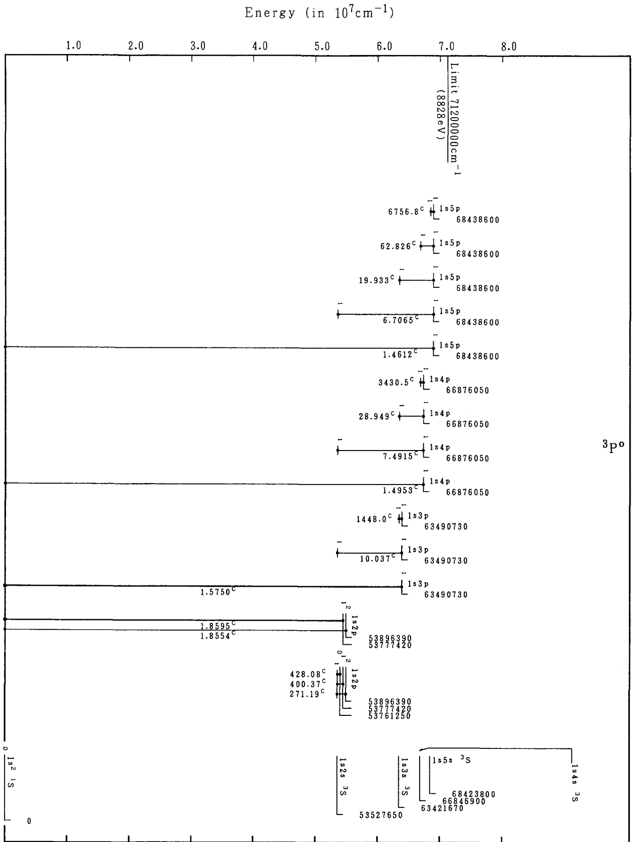
Grotrian Diagrams for Fe XXV (He-Sequence)-Continued
