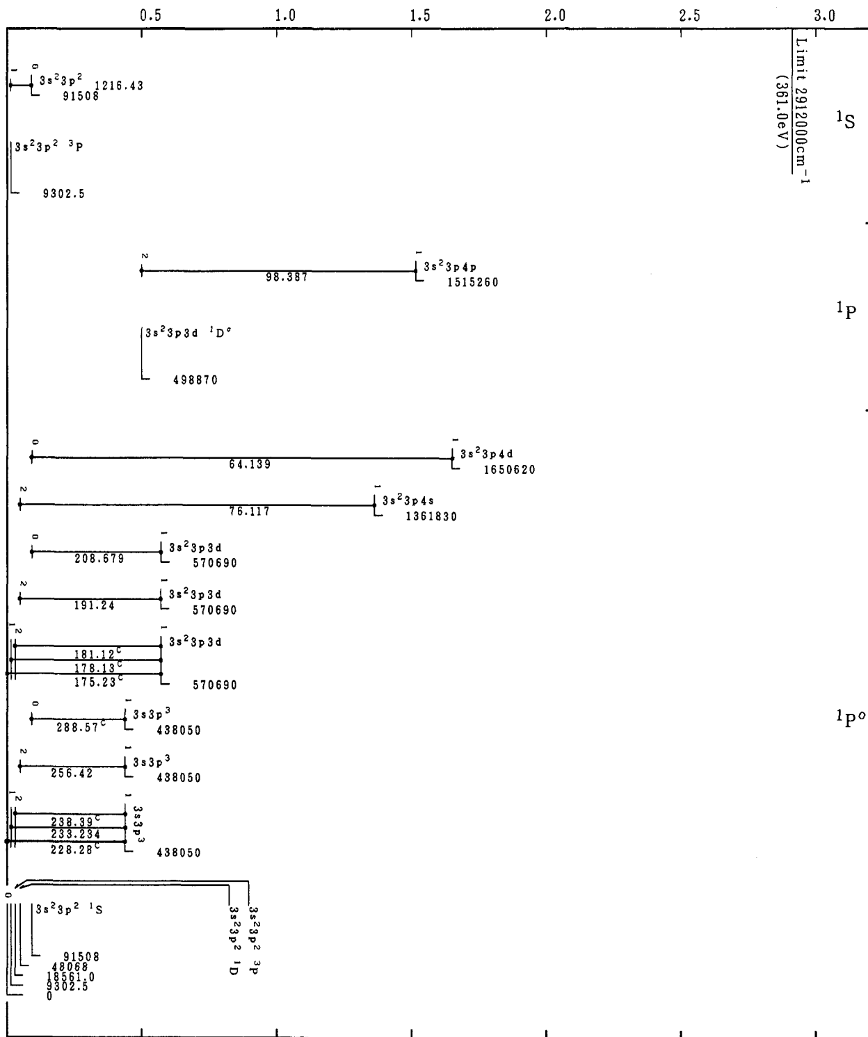
Grotrian Diagrams for Fe XIII (Si-Sequence)
