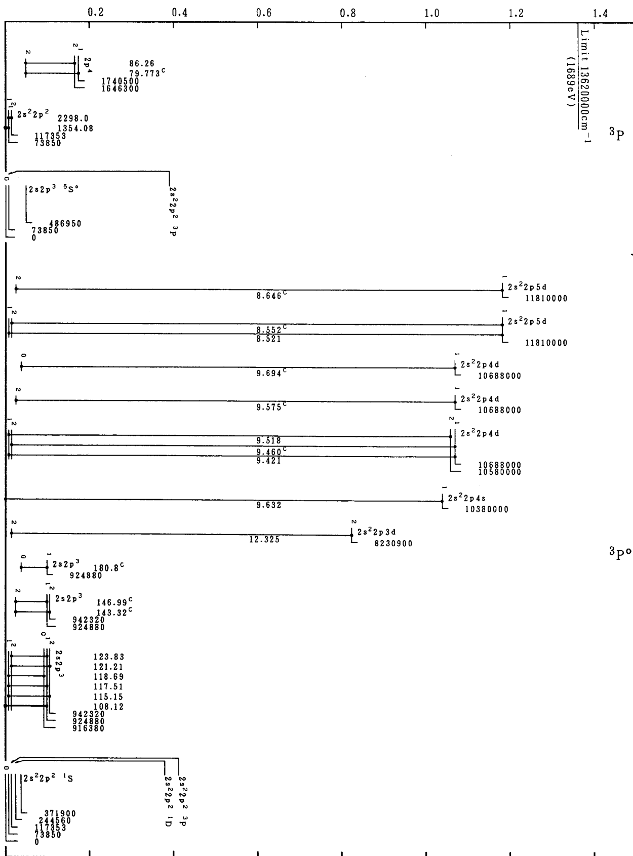
Grotrian Diagrams for Fe XXI (C-Sequence)-Continued
