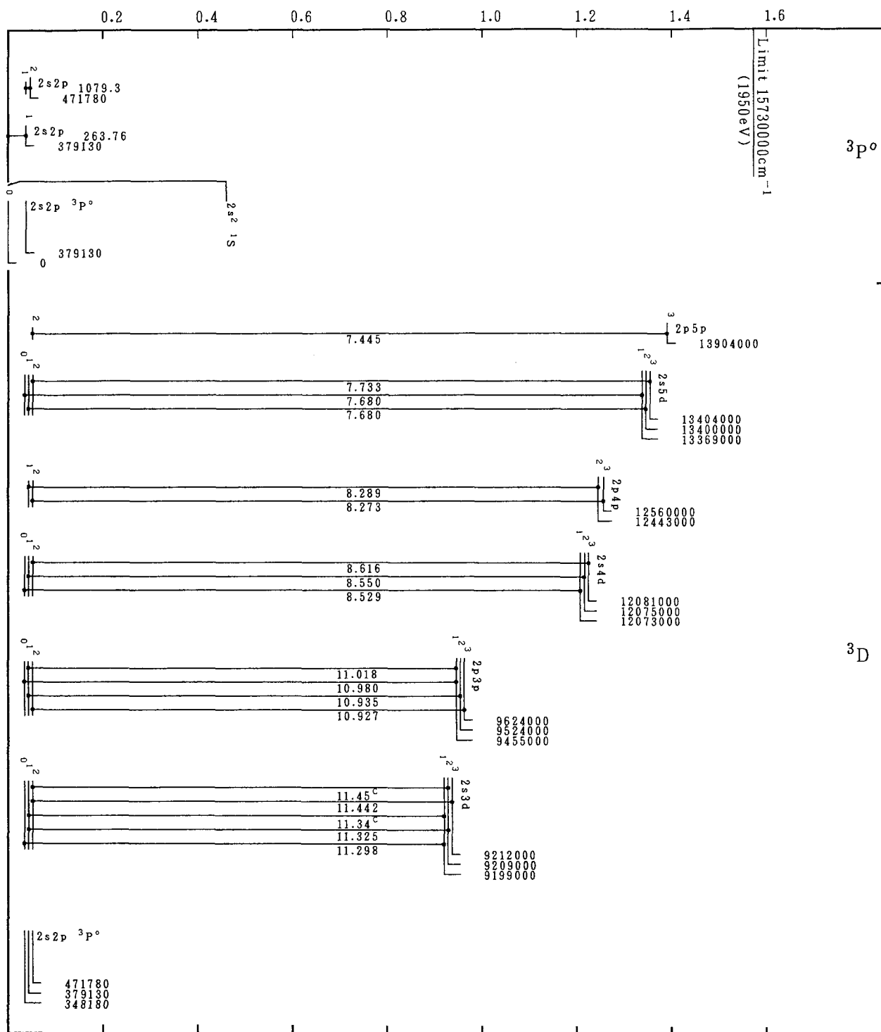
Grotrian Diagrams for Fe XXIII (Be-Sequence)-Continued
