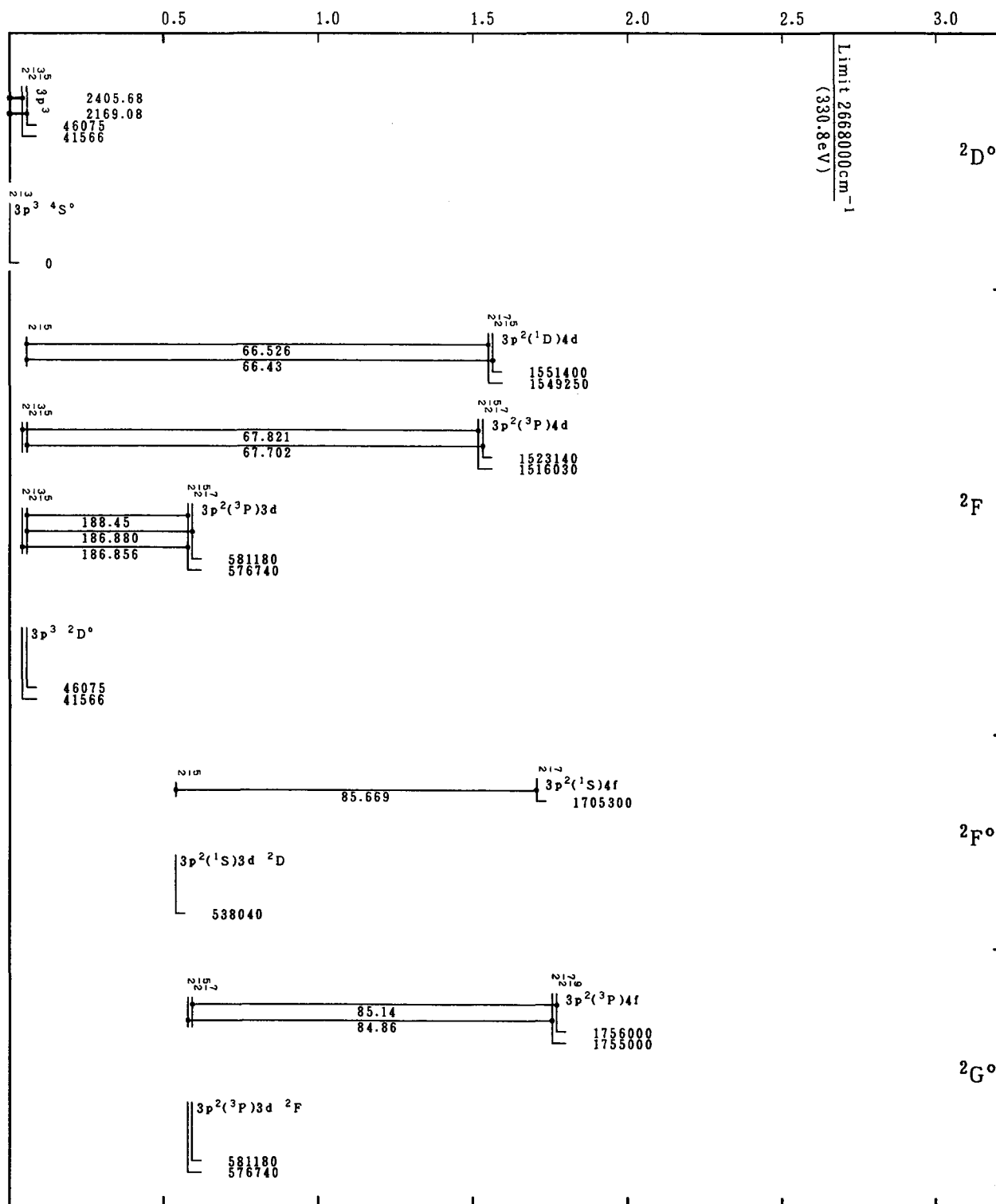
Grotrian Diagrams for Fe XII (P-Sequence)-Continued
