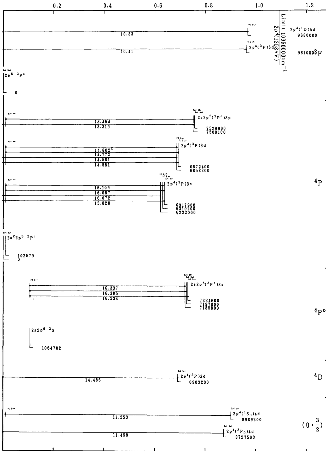
Grotrian Diagrams for Fe XVIII (F-Sequence)-Continued
