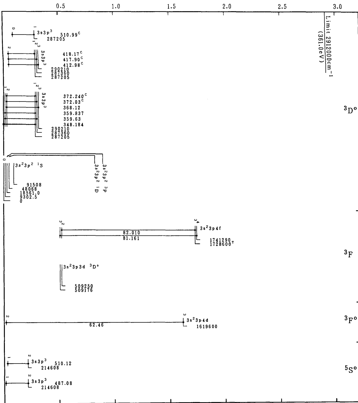
Grotrian Diagrams for Fe XIII (Si-Sequence)-Continued
