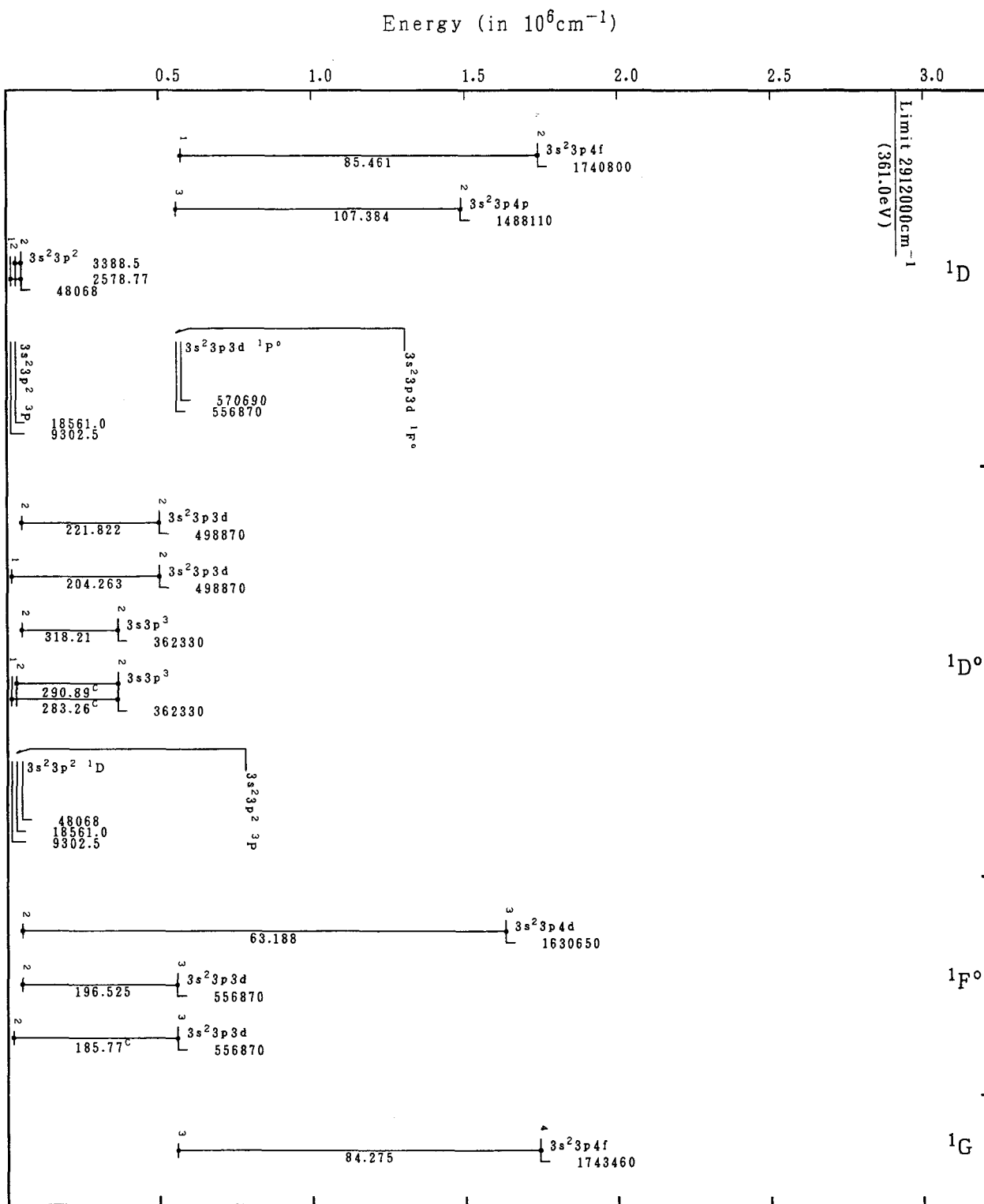
Grotrian Diagrams for Fe XIII (Si-Sequence)-Continued
