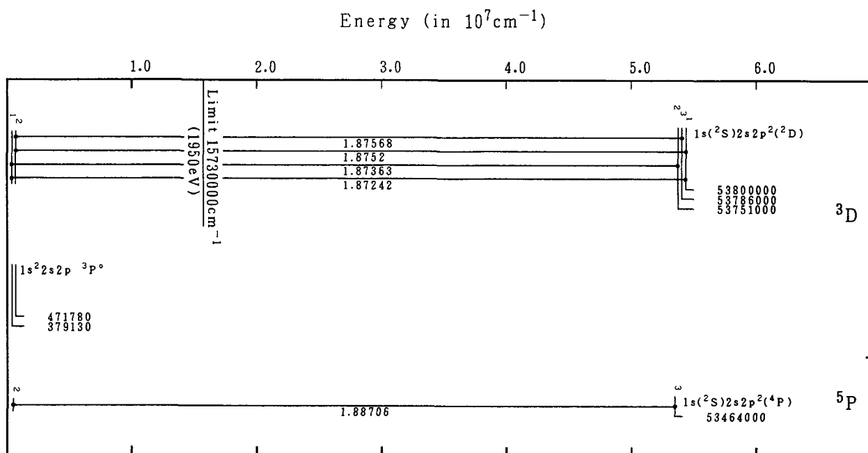
Grotrian Diagrams for Fe XXIII (Be-Sequence)-Continued
