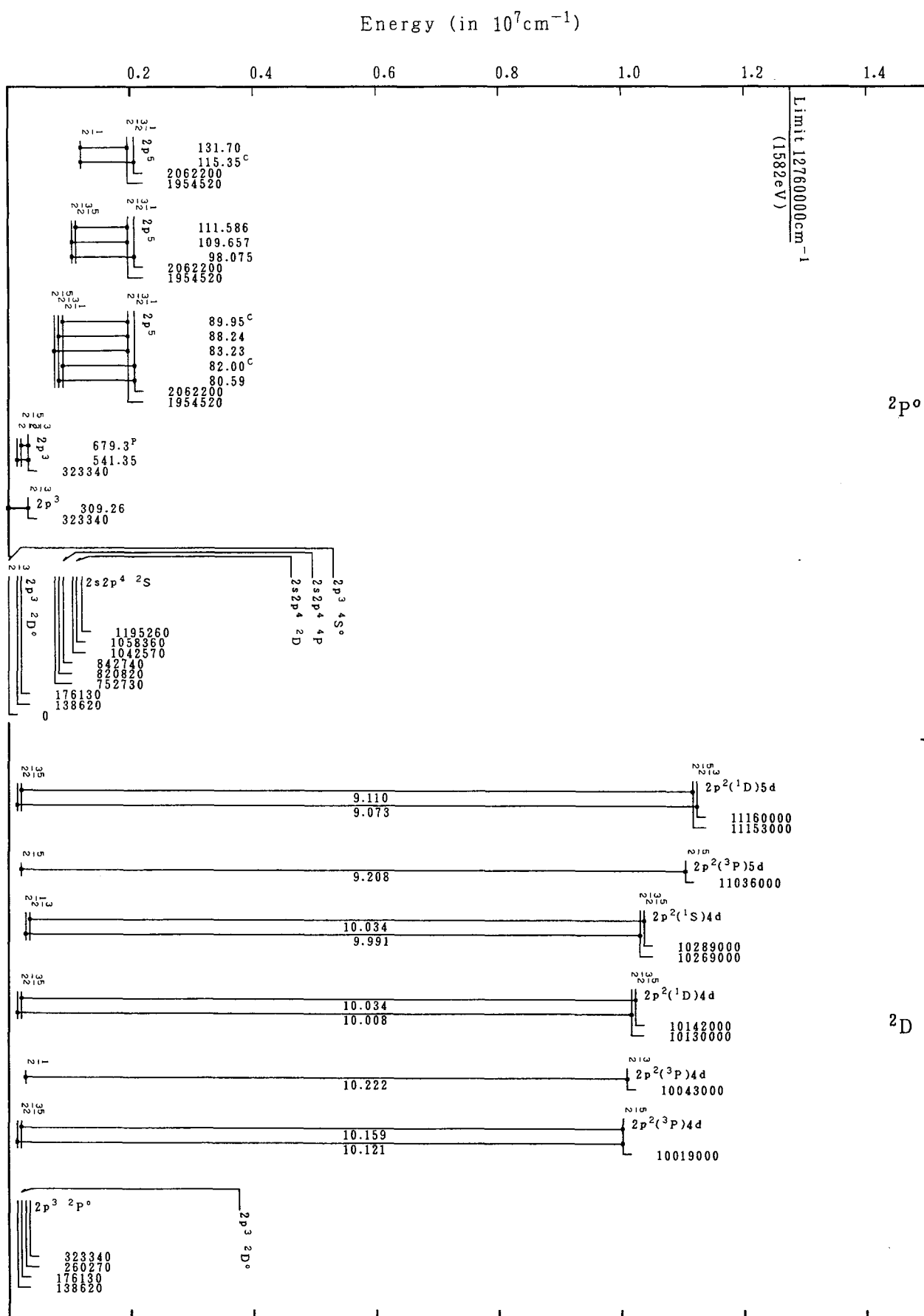
Grotrian Diagrams for Fe XX (N-Sequence)-Continued
