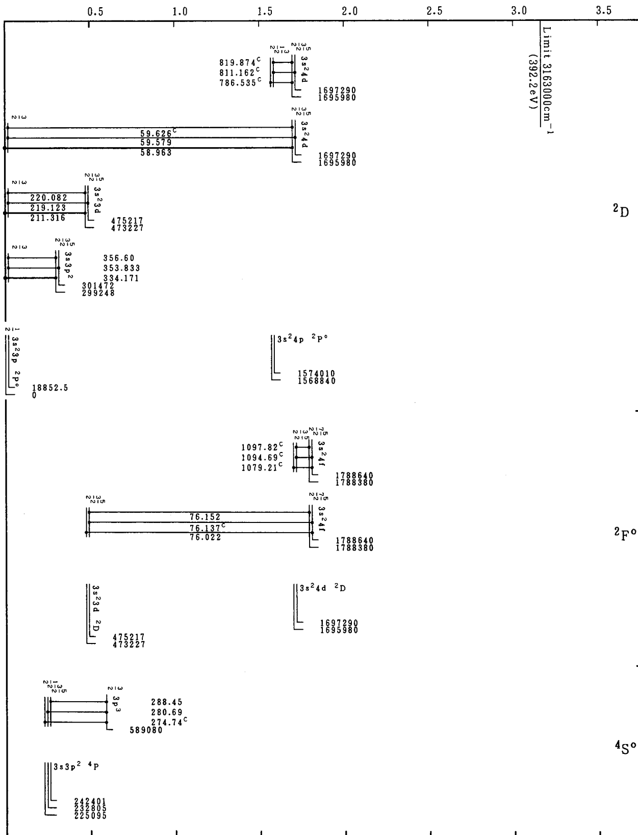
Grotrian Diagrams for Fe XIV (Al-Sequence)-Continued
