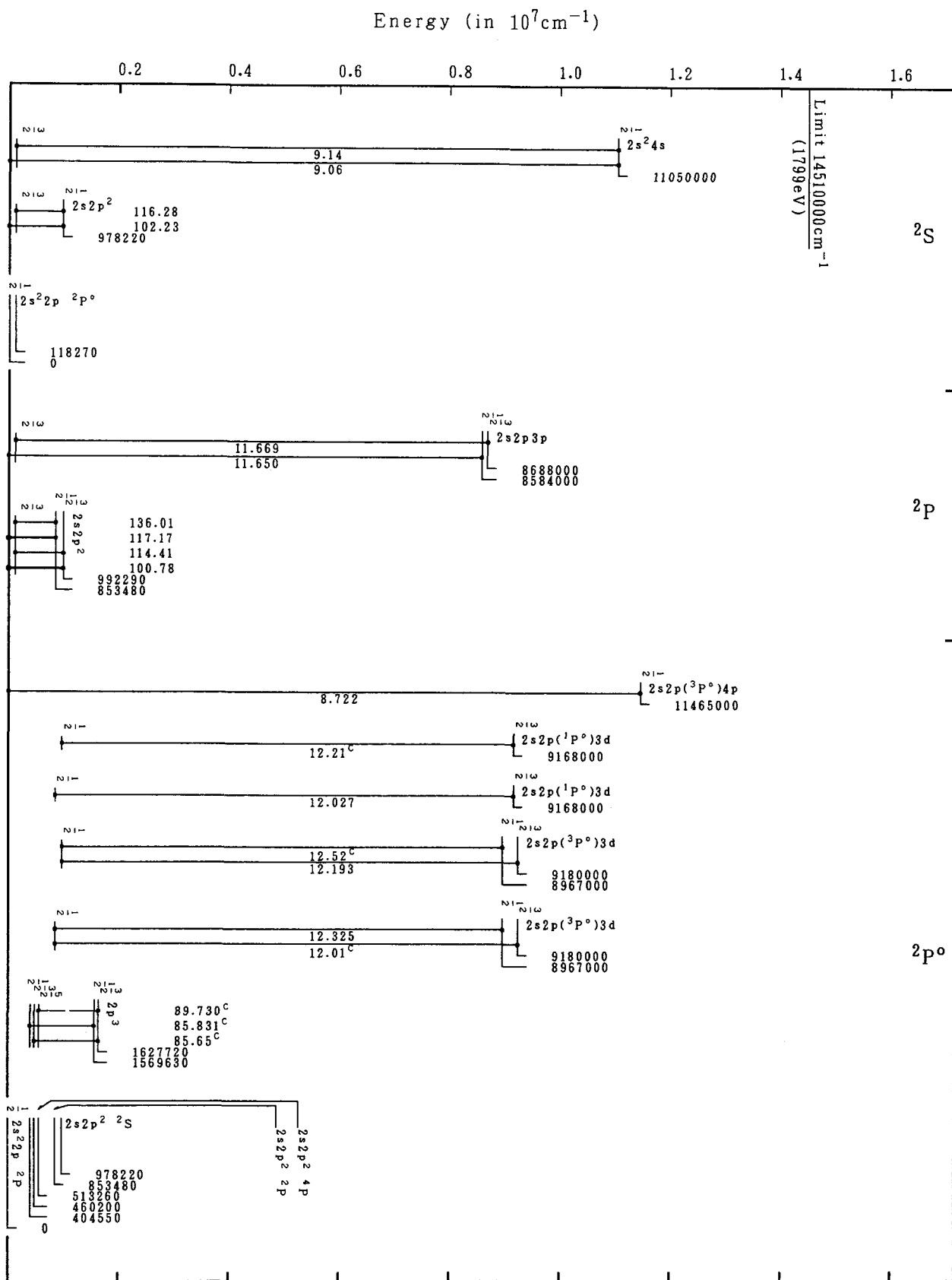
Grotrian Diagrams for Fe XXII (B-Sequence)
