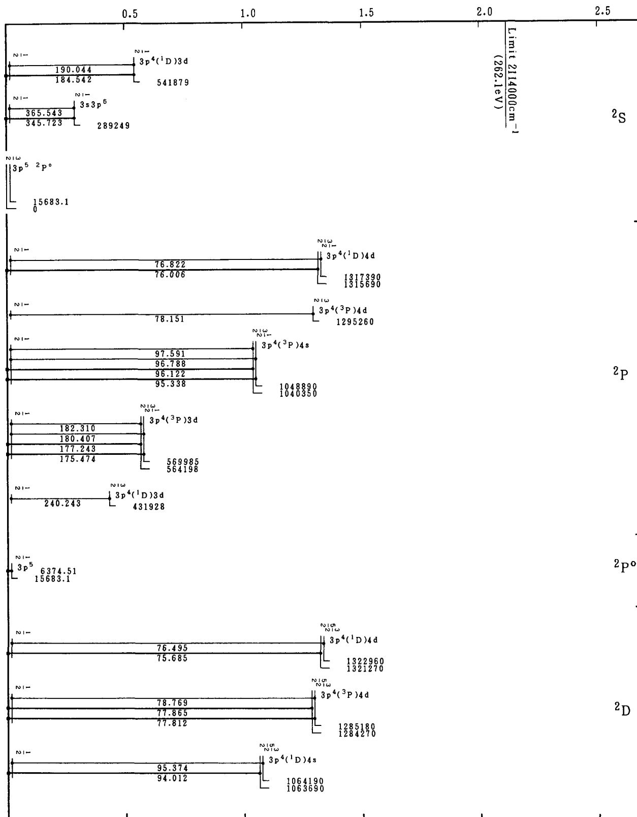
Grotrian Diagrams for Fe X (Cl-Sequence)
