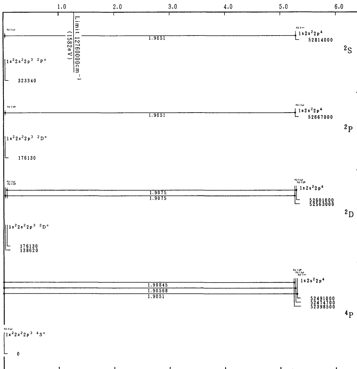
Grotrian Diagrams for Fe XX (N-Sequence)-Continued
