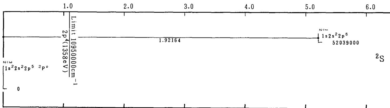
Grotrian Diagrams for Fe XVIII (F-Sequence)-Continued
