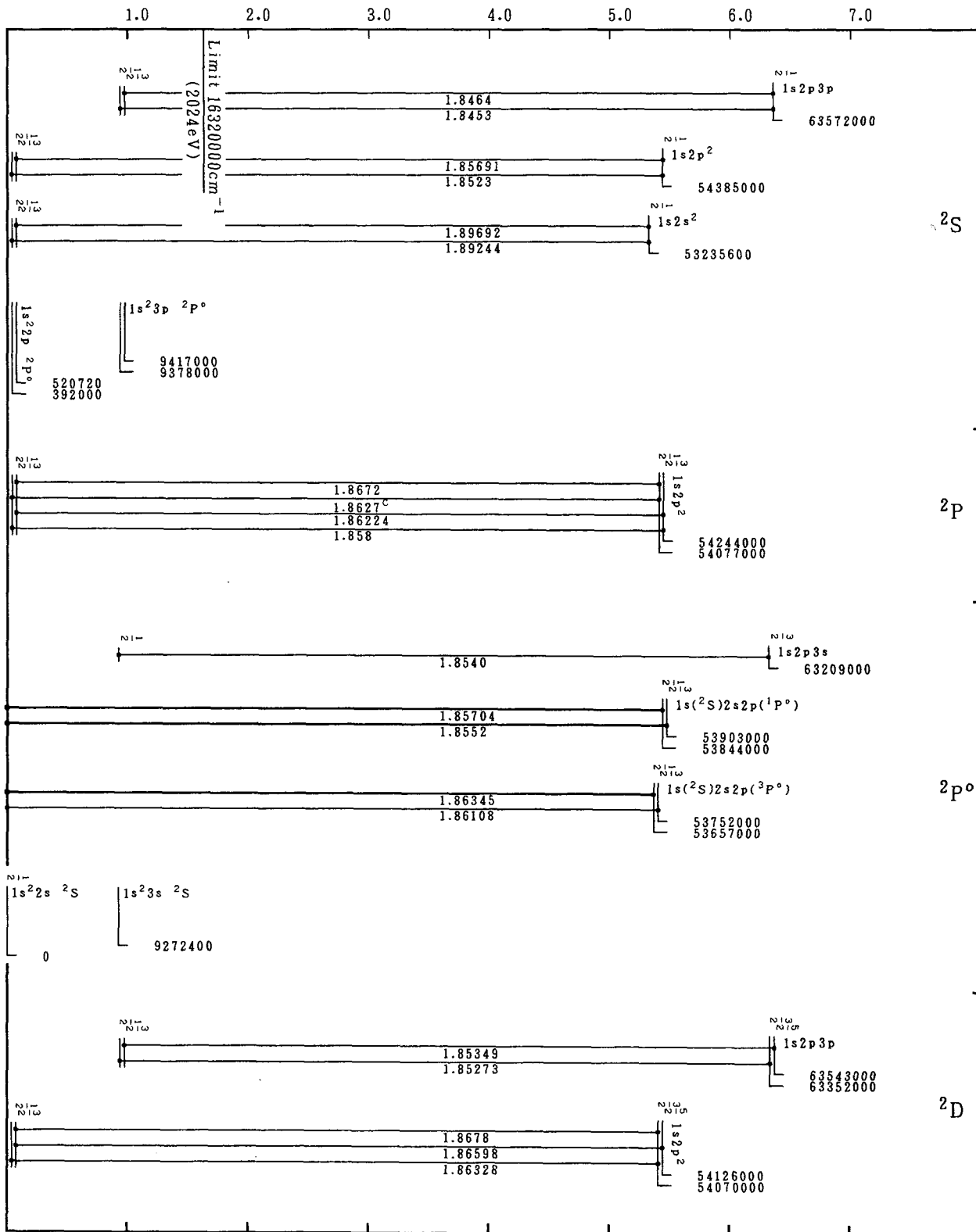
Grotrian Diagrams for Fe XXIV (Li-Sequence)-Continued
