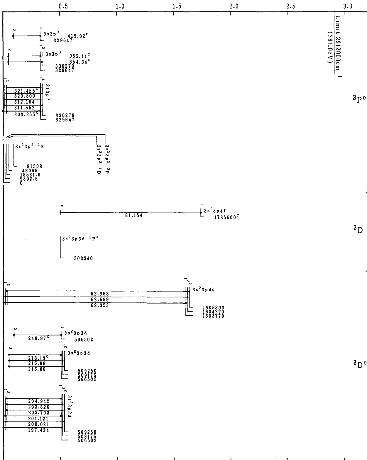
Grotrian Diagrams for Fe XIII (Si-Sequence)-Continued
