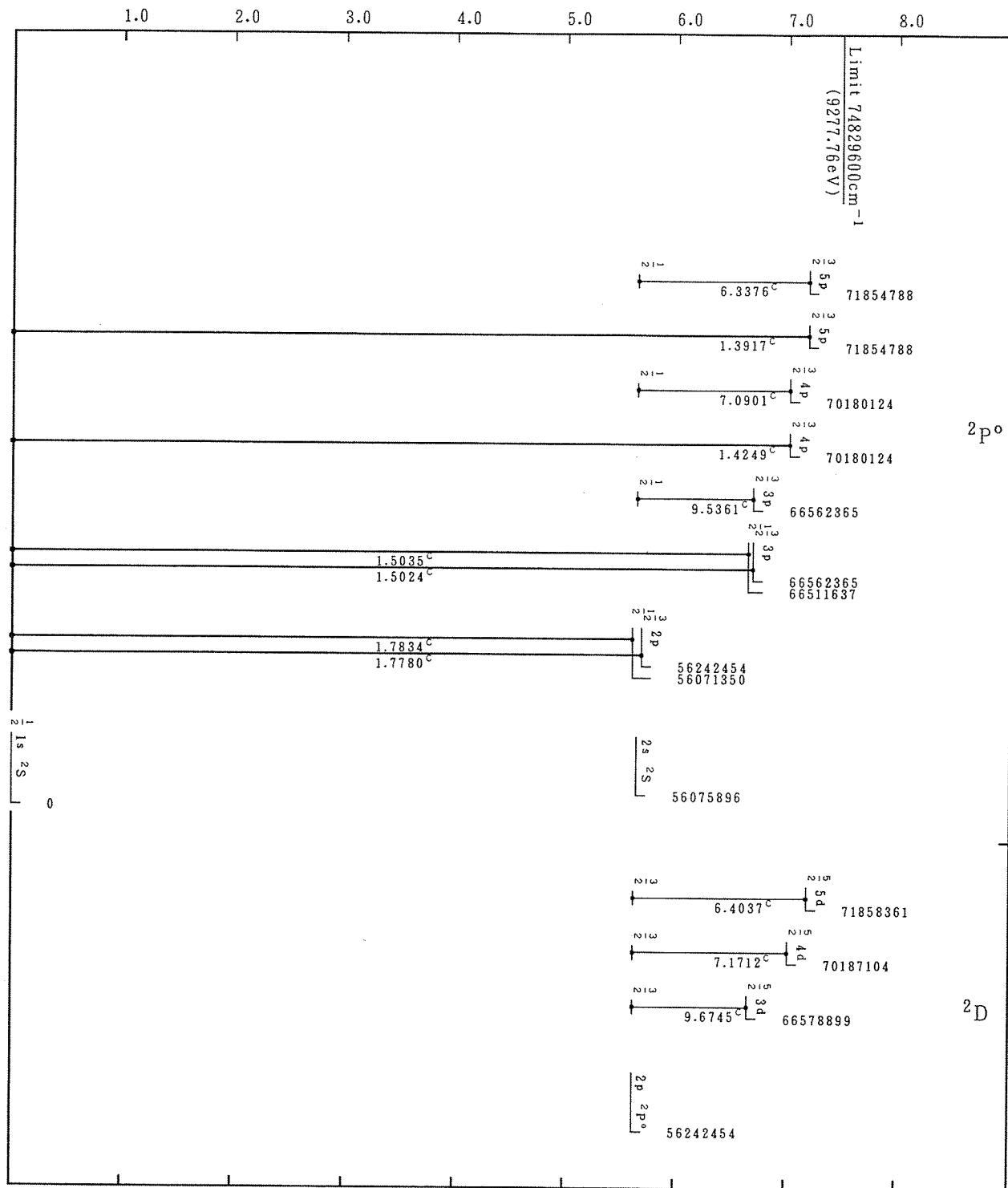
Grotrian Diagrams for Fe XXVI (H-Sequence)
