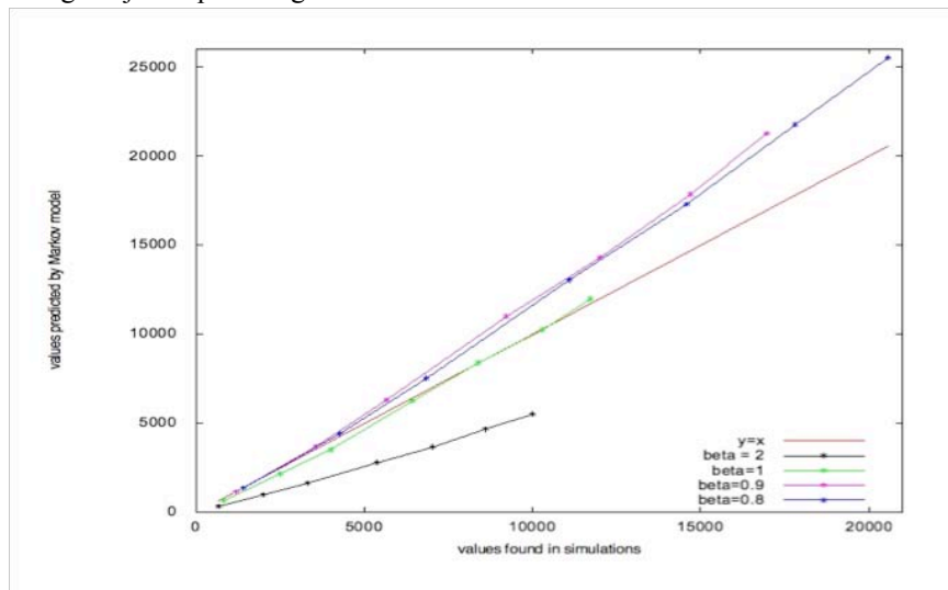
Comparison between the number of ants predicted by the Markov model for the phase transition to occur (prediction) and the number of ants necessary for the phase transition to occur in simulation. For each beta, there are 7 simulations (1000, 5000, 10000, 20000, 30000, 40000 and 50000 points). The perfect fit is y=x (the red line).
