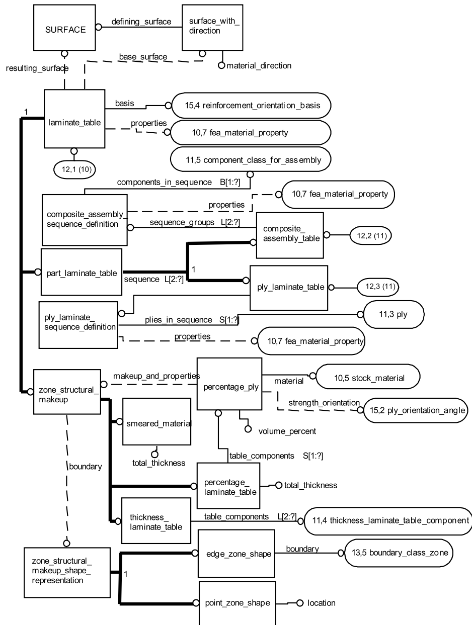
Fig. 2. The core of the STEP AP209 laminate table data model.
