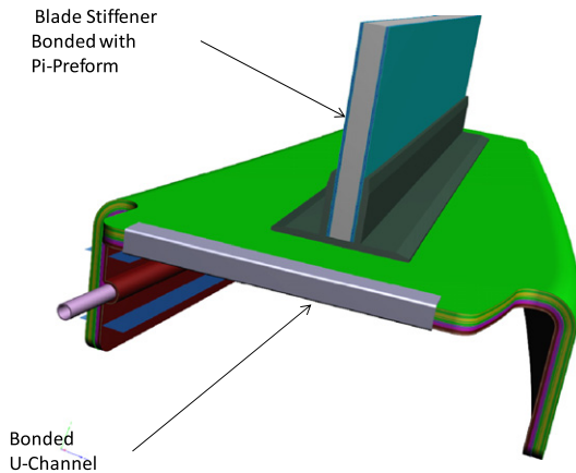
Fig. 7. A complex bonded assembly end view.
