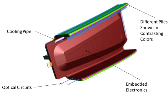
Fig. 6. A complex bonded assembly inside view.
