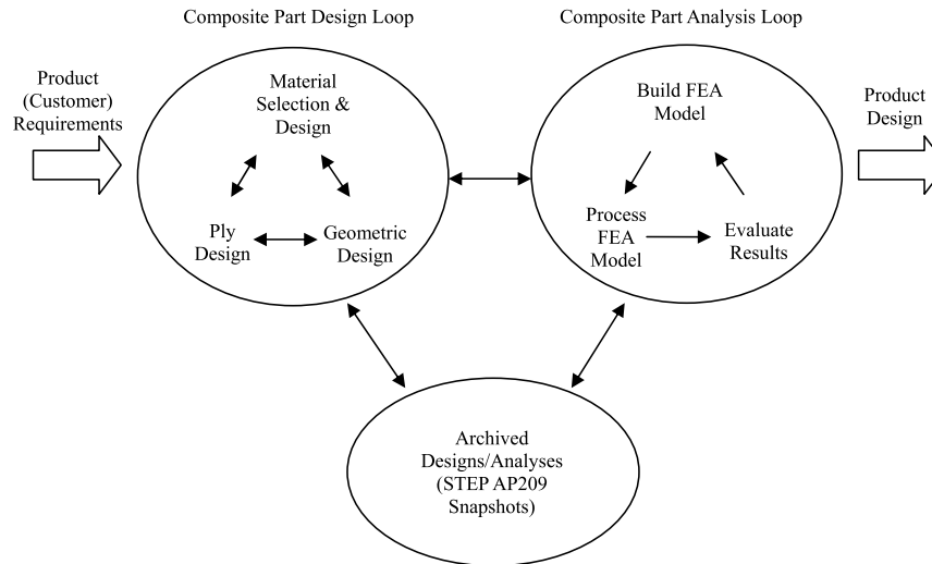
Fig. 1. A depiction of the role of STEP AP209 in the design and analysis of composite structures.
