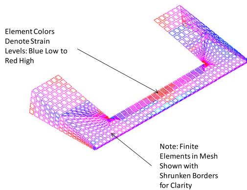
Fig. 4. The TACOM composite armored vehicle's nose finite element model, showing stress results.
