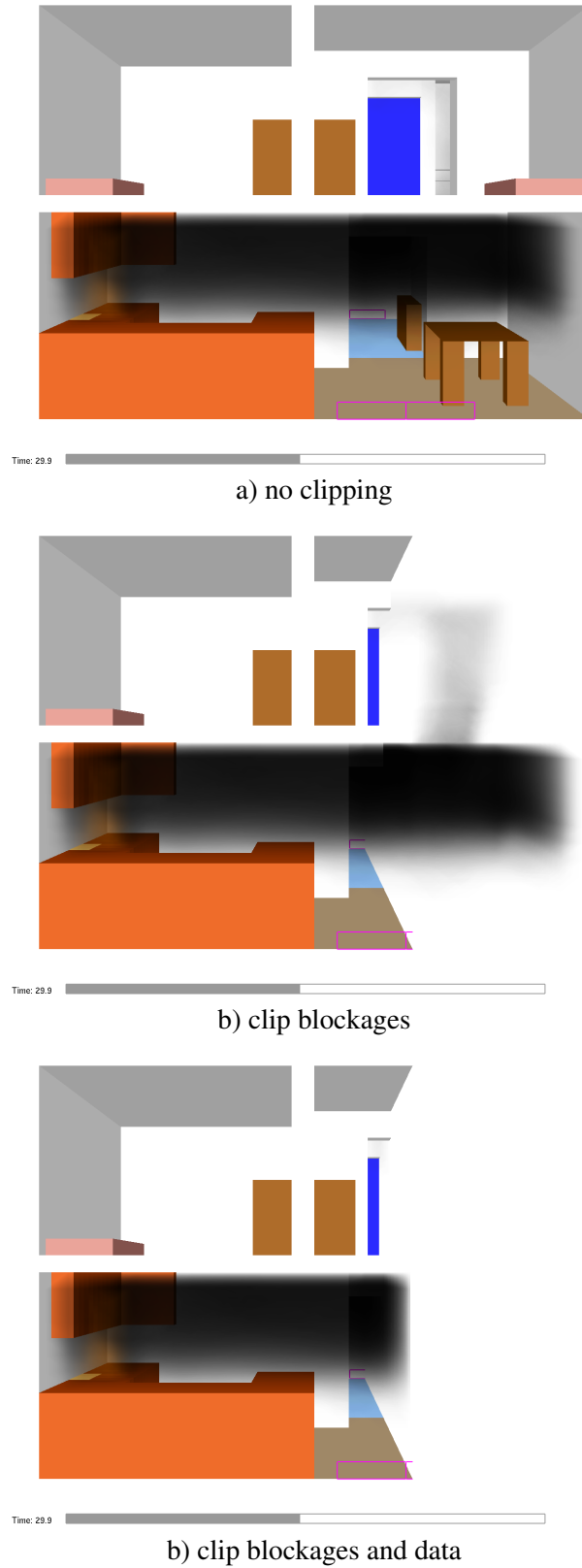
Figure 6.13: Three views of a scene. The first view is drawn without clipping, the second view shows the scene clipping only the geometry (blockages), the third view shows the scene clipping both the geometry and the data.
