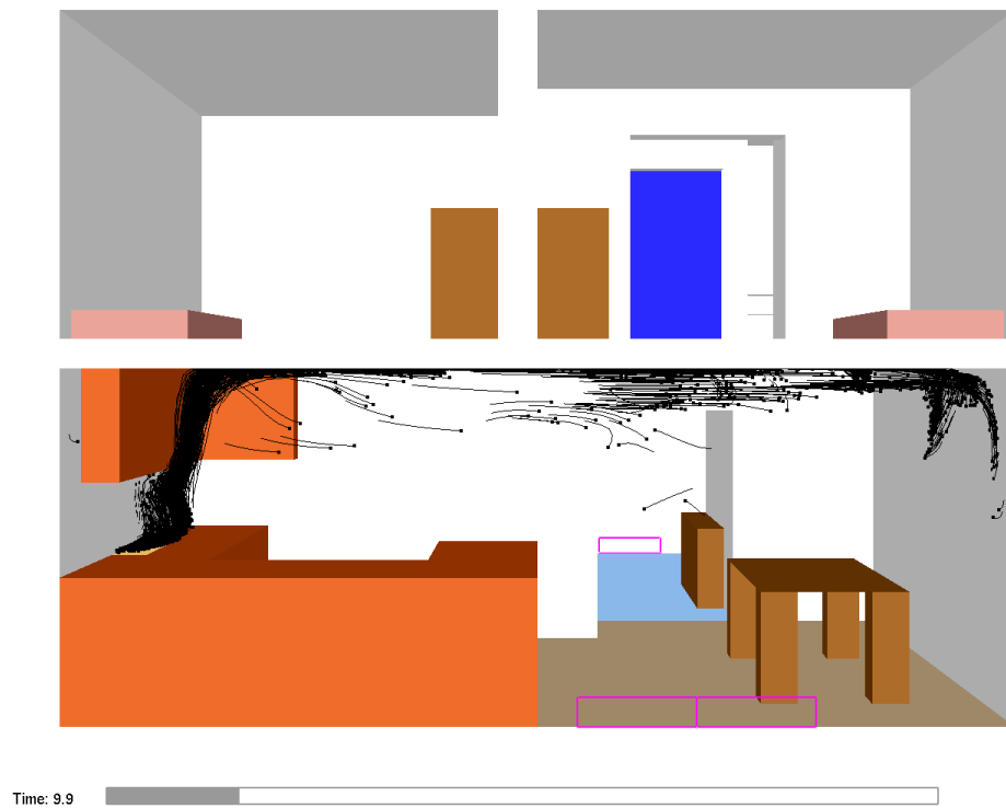
Figure 3.2: Townhouse kitchen fire visualized using streak lines. The pin heads shows flow conditions at 10 s, the corresponding tails shows conditions 1.0 s earlier.
