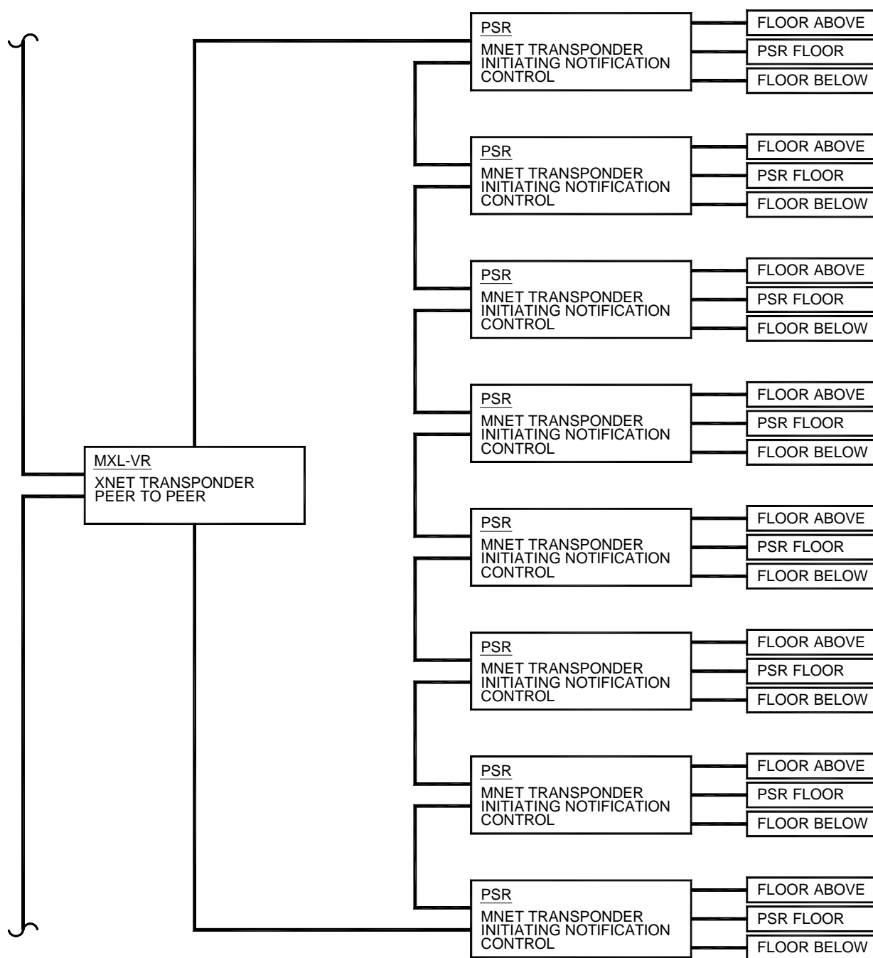
Figure 5–23. Single-line schematic of MNET network configuration.
