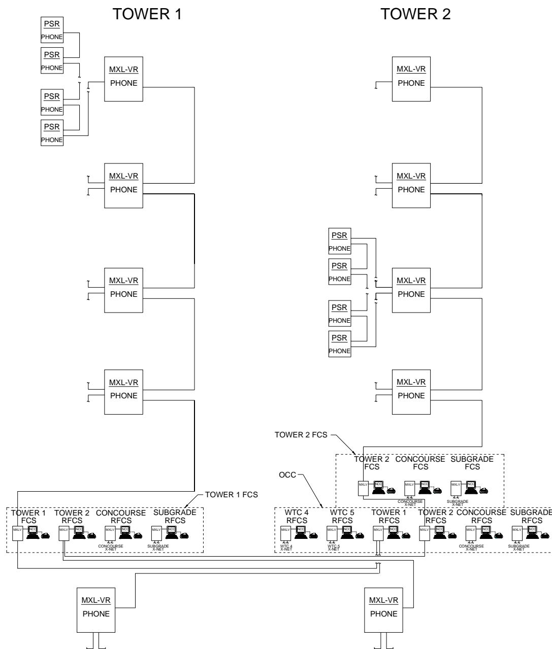
Figure 5–31. Single-line schematic of floor warden and fireman telephones.
