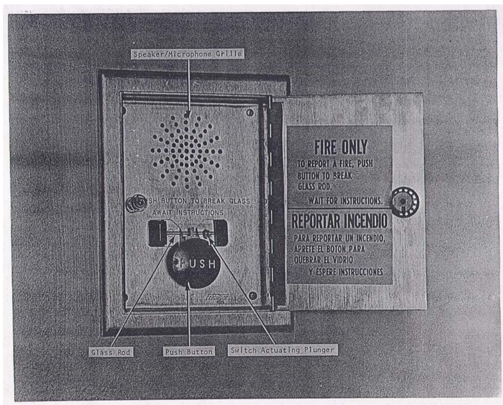
Figure 3–2. Interior of break-glass station.
