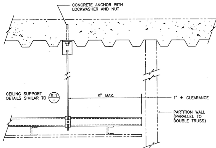
TYPICAL SECTION AT PARTITION WALL
