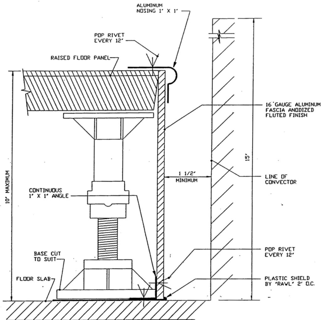
DETAIL OF RAISED FLOOR @ PERIMETER INDUCTION UNITS
