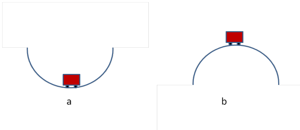
Figure 1: a) Stable equilibrium and b) unstable equilibrium.
