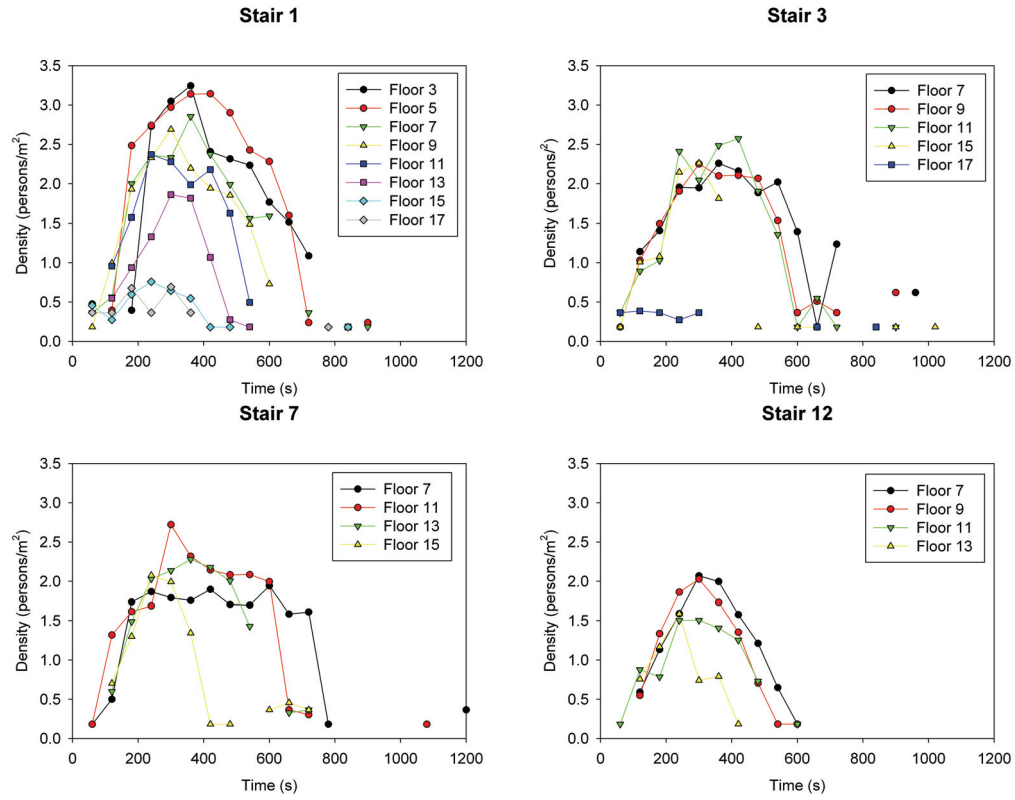
Figure 8. Evacuee density (people/m 2 ) as a function of time in four stairwells during a fire drill evacuation in an 18-story building
