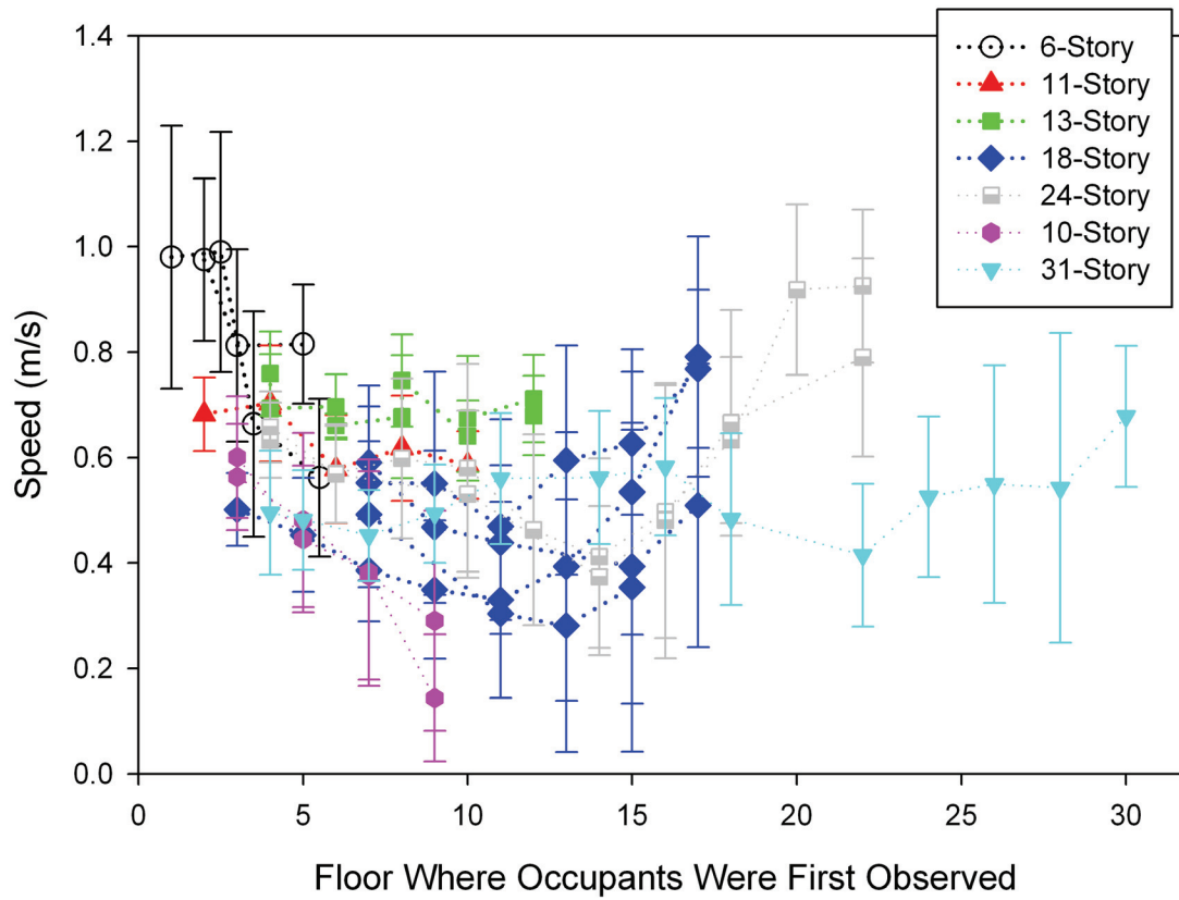
Figure 5. Occupant movement speed (with standard deviation) down stairwells in several fire drill evacuations.
