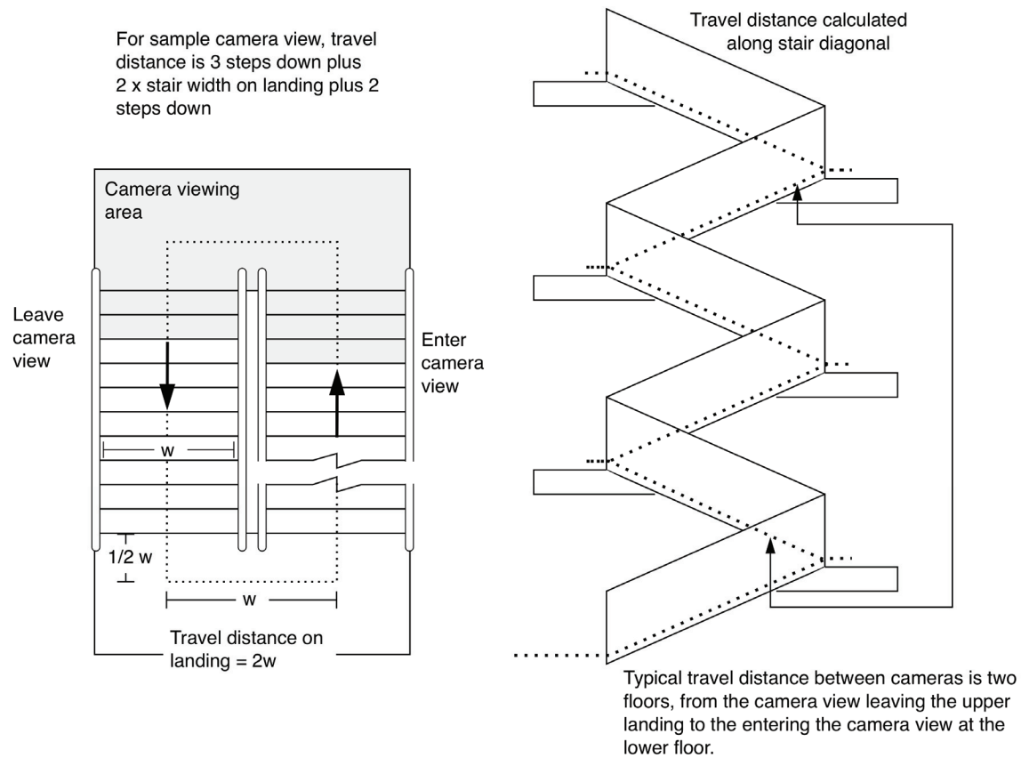
Figure 7. Details of camera views and travel distances used to calculate local movement speed and occupant density.
