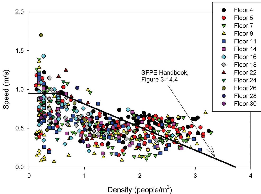
Figure 9. Local speed as a function of local density for evacuees in all stairwells of 10-, 18-, 24-, and 31-story buildings during fire drill evacuations.
