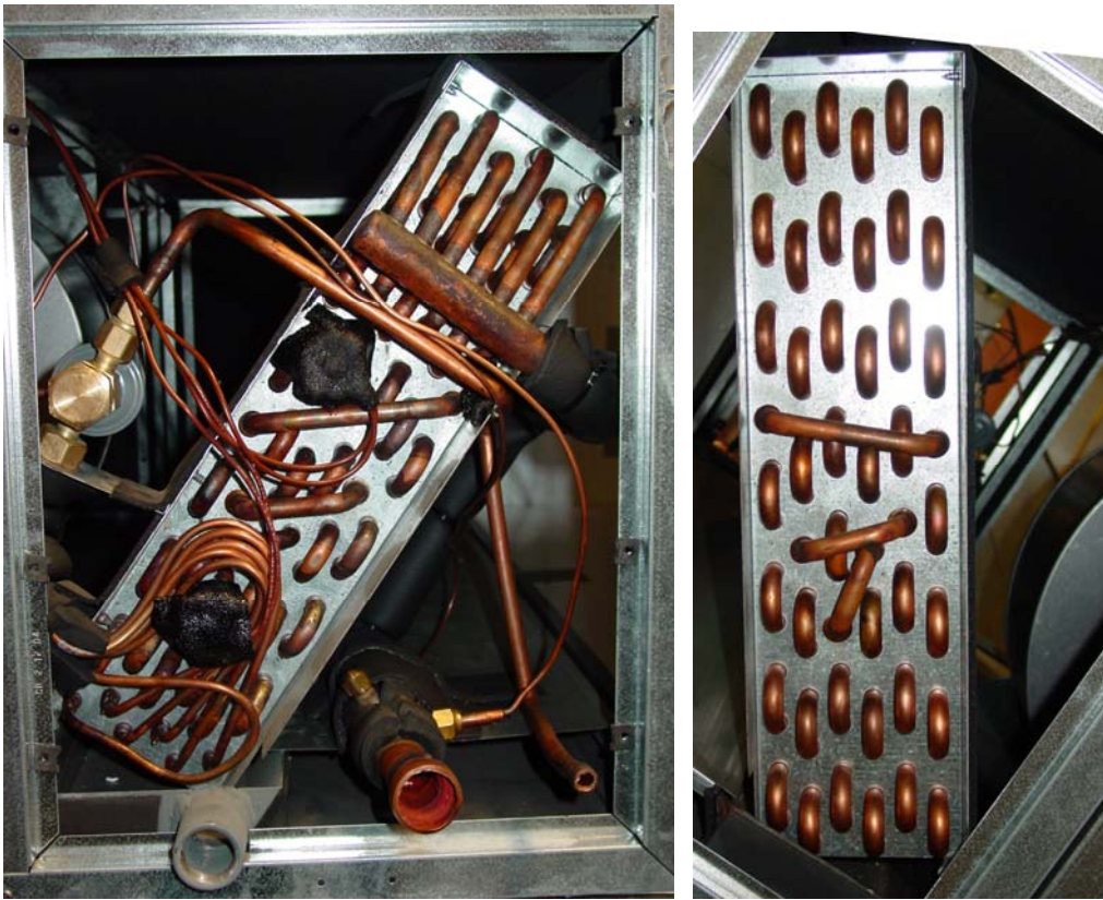
Figure A9: Mixed coil #2 side views
