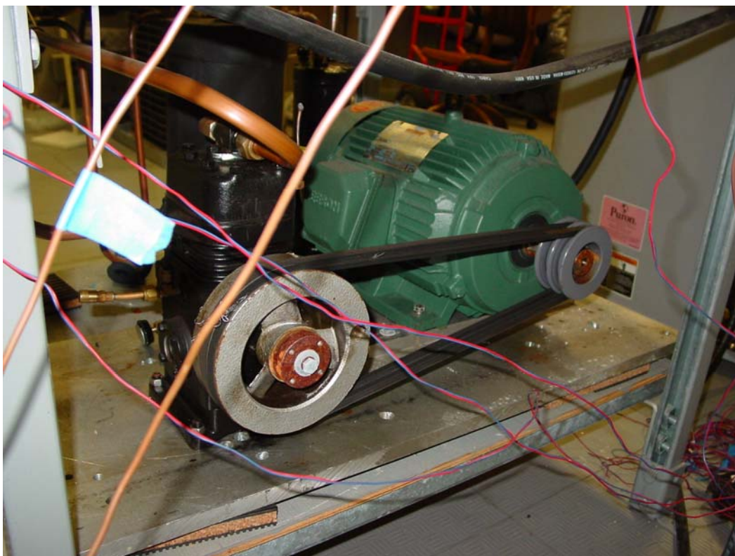
Figure B8: Compressor and motor for water-cooled condensing unit (guard removed)
