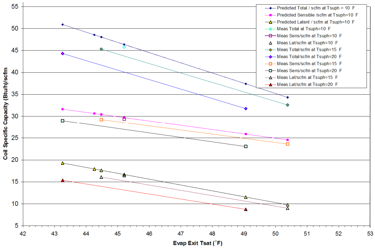
Figure 7.2.2: Mixed #2 coil-only capacity per unit airflow rate at different superheats
