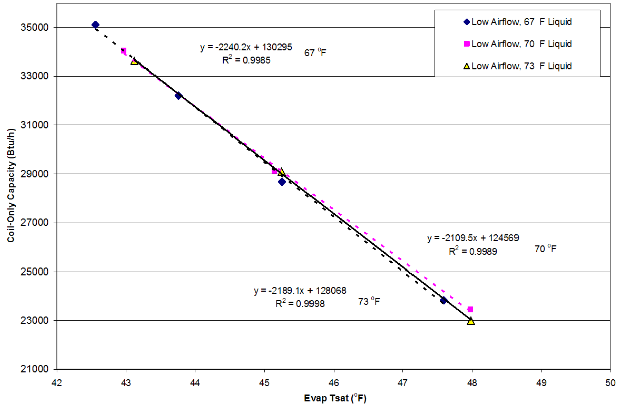
Figure 6.1.6: Mixed coil #1 F 1 coil-only capacity for different refrigerant liquid temperatures
