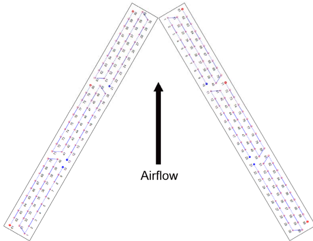
Figure A2: Matched coil refrigerant circuitry
