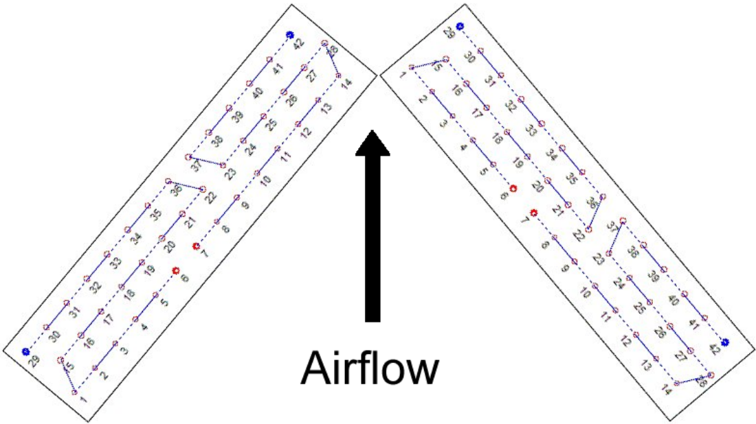
Figure A5: Mixed coil #1 refrigerant circuitry
