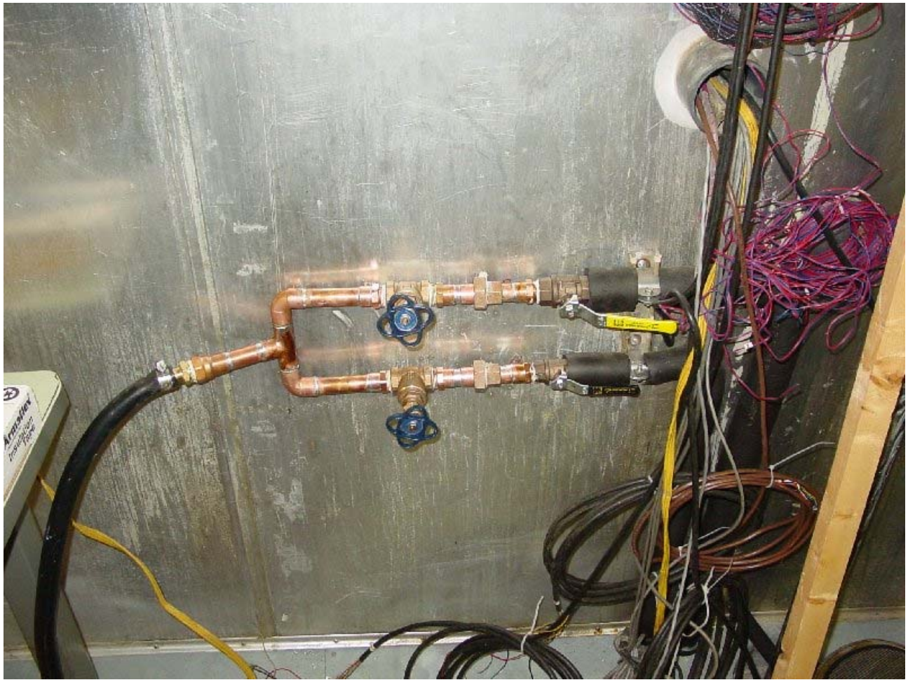
Figure C8: Hot and cold house water mixed before going to water-heated evaporator unit
