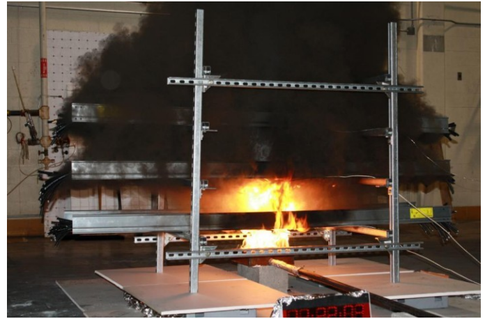
FIGURE 5. Multiple Tray (MT) cable test apparatus.
