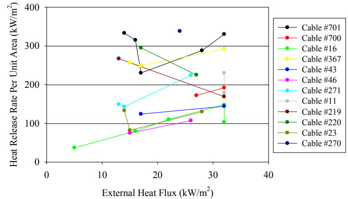
FIGURE 11. Summary of the radiant panel heat release rates.
