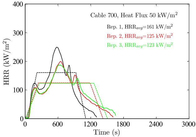
FIGURE 9. Cone calorimeter results for a thermoset cable. The heat flux of 50 kW/m 2 represents the power of the cone heater. The HRR values represent the heat released per unit area of sample for the three replicate experiments.
