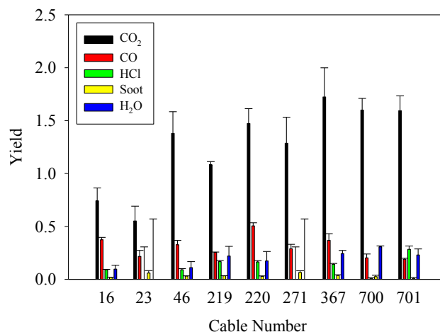
FIGURE 8. Yields (g/g) of major combustion products.
