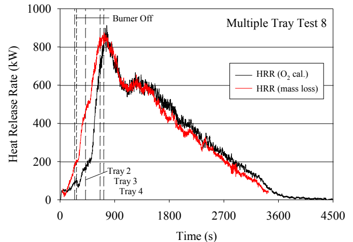
FIGURE 15. Heat release rate of a multiple tray test involving a thermoplastic cable. The vertical lines indicate when each tray became fully involved in the fire. Tray 1 refers to the lowest tray. Note that the involvement of Tray 1 coincided with the extinguishment of the burner.
