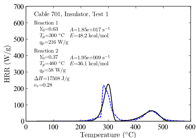
FIGURE 7. MCC results for a typical thermoplastic cable.
