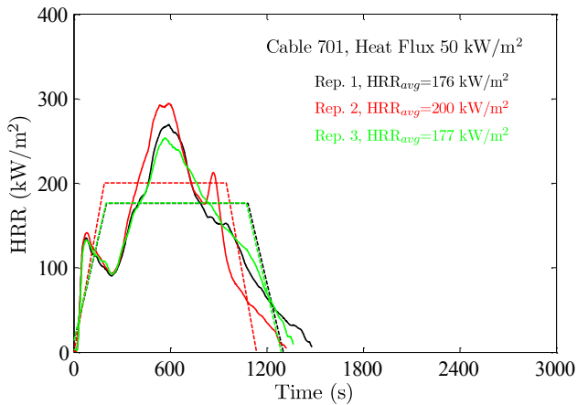
FIGURE 10. Cone calorimeter results for a thermoplastic.
