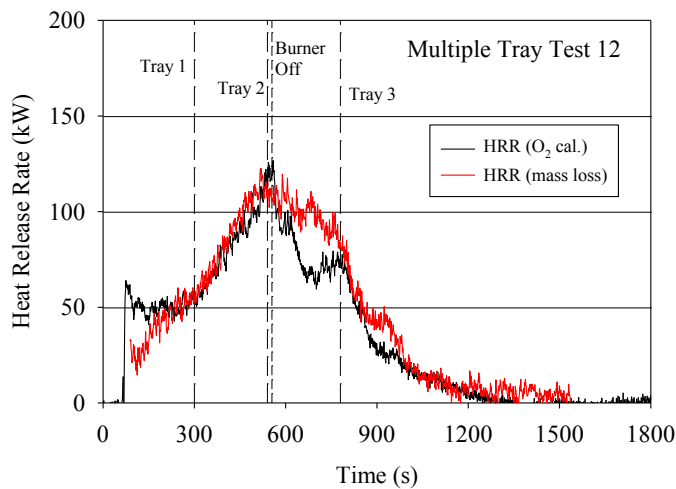
FIGURE 13. Heat Release Rate of a multiple tray test involving thermoset cables. The vertical lines indicate the time when each tray becomes fully involved in the fire. Tray 1 refers to the lowest tray.
