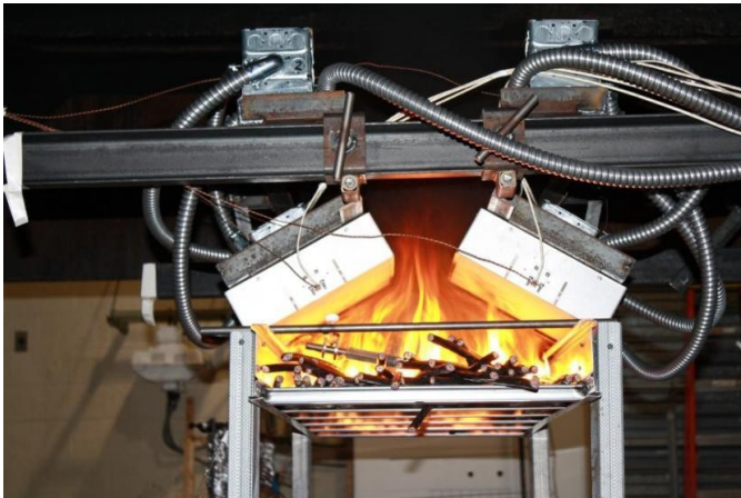
FIGURE 4. End view of radiant panel apparatus
