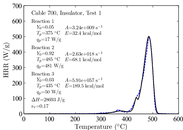
FIGURE 6. MCC results for a typical thermoset cable.
