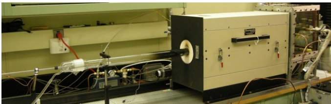
FIGURE 2. ISO/TS 19700 Tube Furnace.
