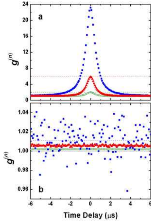
Fig. 2. Measured n^{\text{th}} -order temporal coherences for n = 2 (○), 3 (▲) and 4 (■). (a) Chaotic source data. The magnitude of photon bunching scales roughly as n! , as can be seen from the expected peak g^{(2)} , g^{(3)} and g^{(4)} values of 2 (dashed green line), 6 (dashed red line) and 24 (top axis). (b) Laser source data, also showing the expected value of 1 (black line) and the mean measured g^{(4)} value of 1.011 (dashed blue line). In both (a) and (b), the g^{(2)} data are displayed as a function of \tau , while the g^{(3)} and g^{(4)} data are plotted against parameterized delays that measure temporal distance from the origin, \tau_{P3} = \pm (\tau_1^2 + \tau_2^2)^{1/2} and \tau_{P4} = \pm (\tau_1^2 + \tau_2^2 + \tau_3^2)^{1/2} , respectively, where \pm is determined by the sign of \tau_1 . These trace out cross sections from (\tau_1, \tau_2) = (-6/\sqrt{2} \mu\text{s}, 6/\sqrt{2} \mu\text{s}) to (6/\sqrt{2} \mu\text{s}, -6/\sqrt{2} \mu\text{s}) and (\tau_1, \tau_2, \tau_3) from (-4 \mu\text{s}, 2 \mu\text{s}, 4 \mu\text{s}) to (4 \mu\text{s}, -2 \mu\text{s}, -4 \mu\text{s}) .
