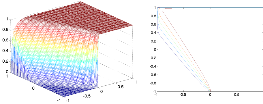
Fig. 4.2: Computed solution (left) and contours (right) of a convection-dominated steady convection-diffusion flow, Pe = 250 , corresponding to example 4.2.
