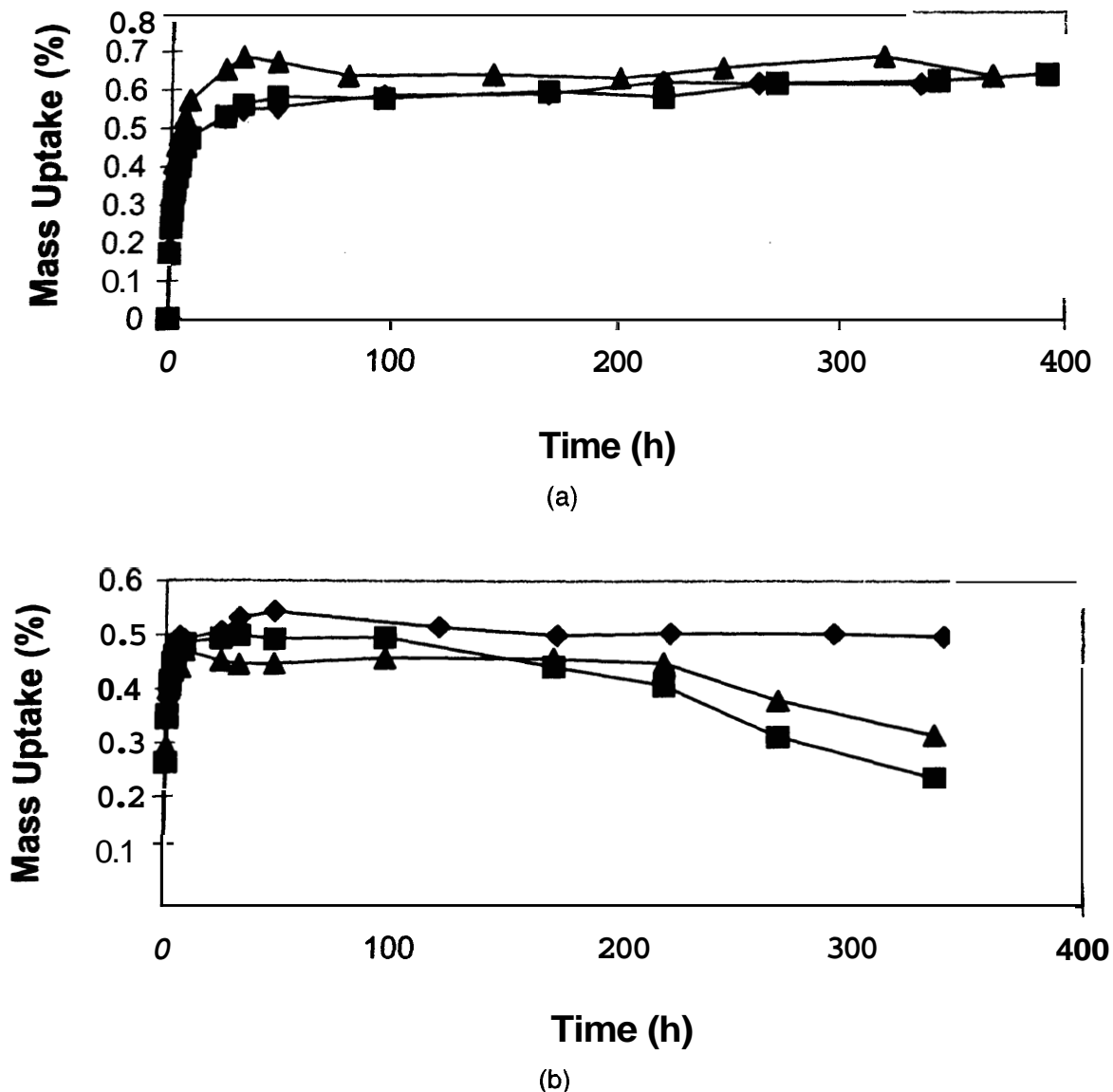
Fig. 4. Mass uptake curves for (a) vinyl ester and (b) isopolyester in water ♦, salt solution A ▲ and concrete pore solution ■ at 60°C (estimated standard deviation is 0.08 mass%).
