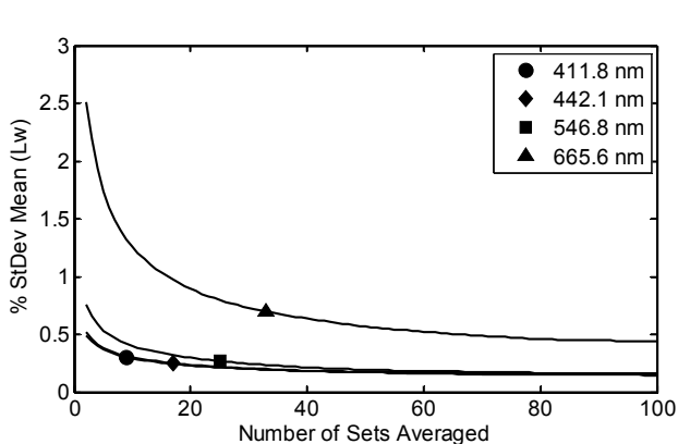
Fig. 9. Percent standard deviation of the mean water-leaving radiance as a function of the number of sets averaged.
