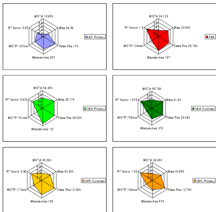
Fig. 24. 3D Person Tracking – Multimodal subtask: Radar Charts
